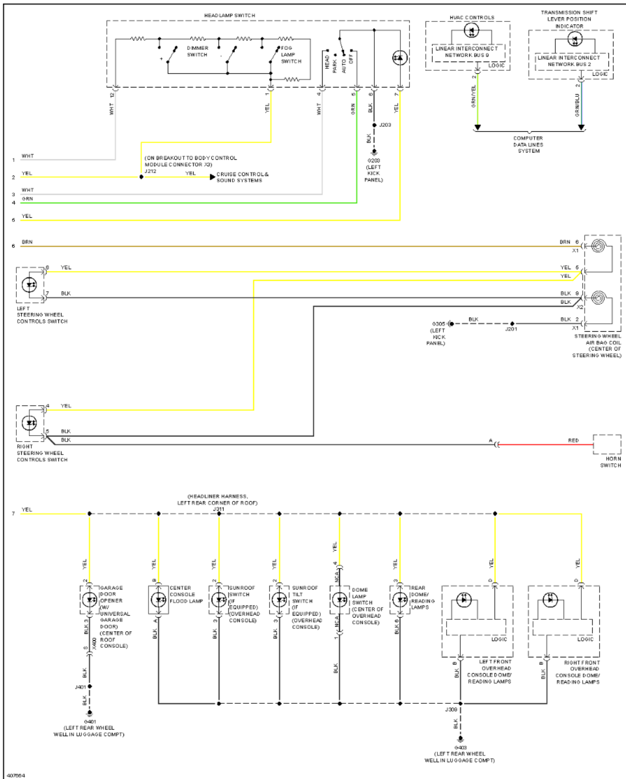
Fig. 72: Instrument Illumination Circuit (2 of 2)
