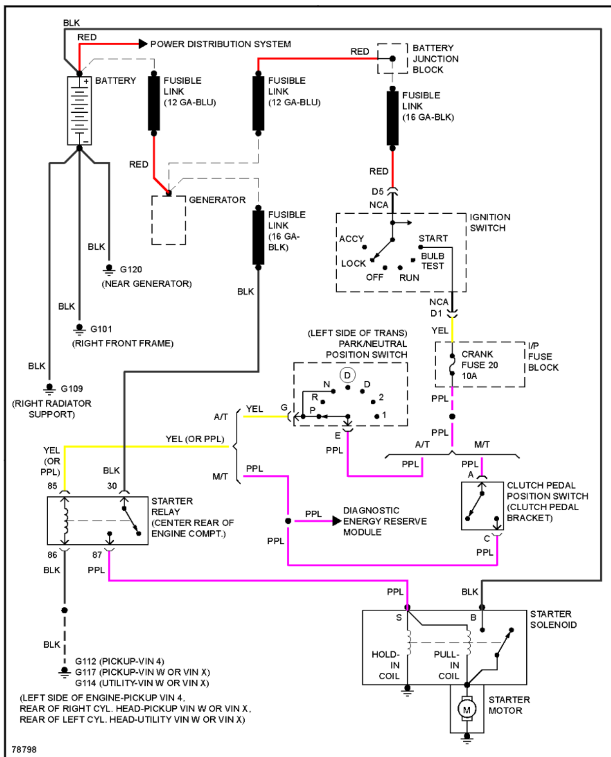
Fig. 34: Starting Circuit
