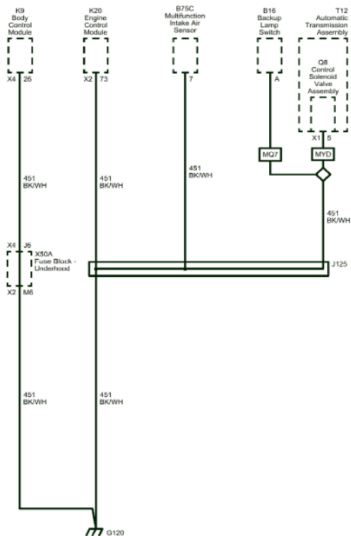
Fig. 5: G120 (2500/3500 with L96 or LC8) Courtesy of GENERAL MOTORS COMPANY
