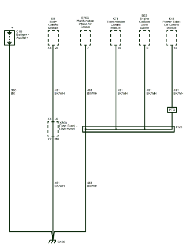
Fig. 6: G120 (2500/3500 with L5P) Courtesy of GENERAL MOTORS COMPANY
