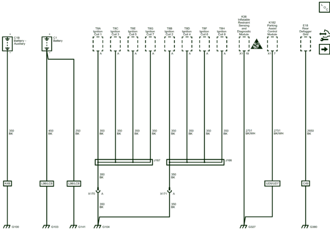
Fig. 1: G100, G103, G104, G141, G327, and G380 (2500/3500)
