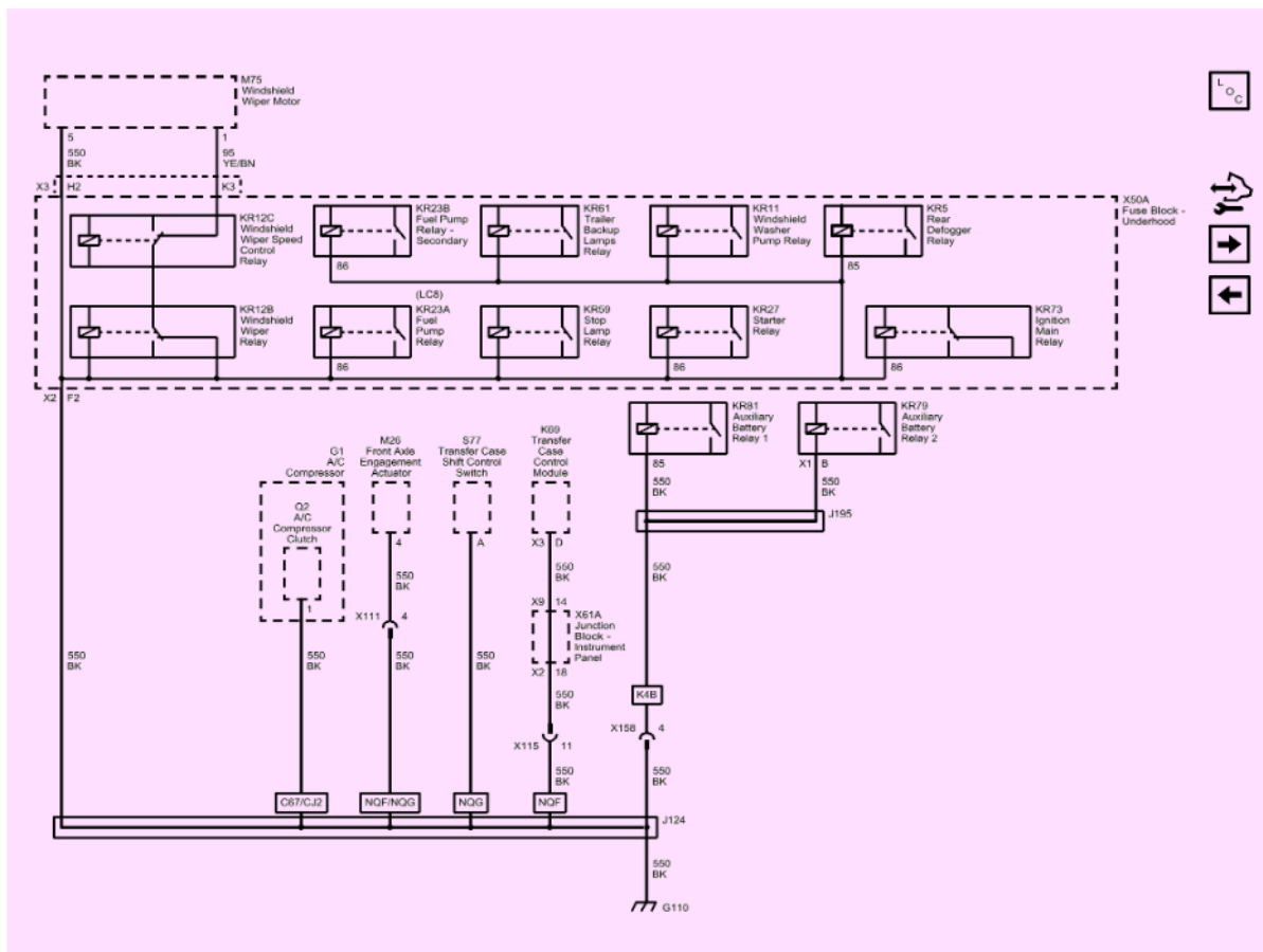
Fig. 3: G110 (2500/3500 with L96 or LC8) Courtesy of GENERAL MOTORS COMPANY
