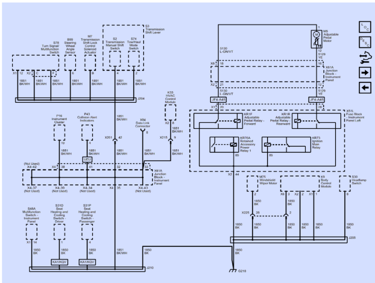
Fig. 12: G218 (2500/3500 except E29) Courtesy of GENERAL MOTORS COMPANY
