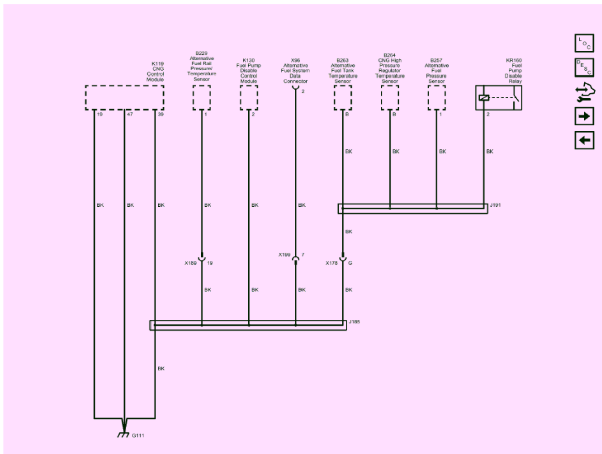
Fig. 7: G111 (2500/3500 with LC8)
