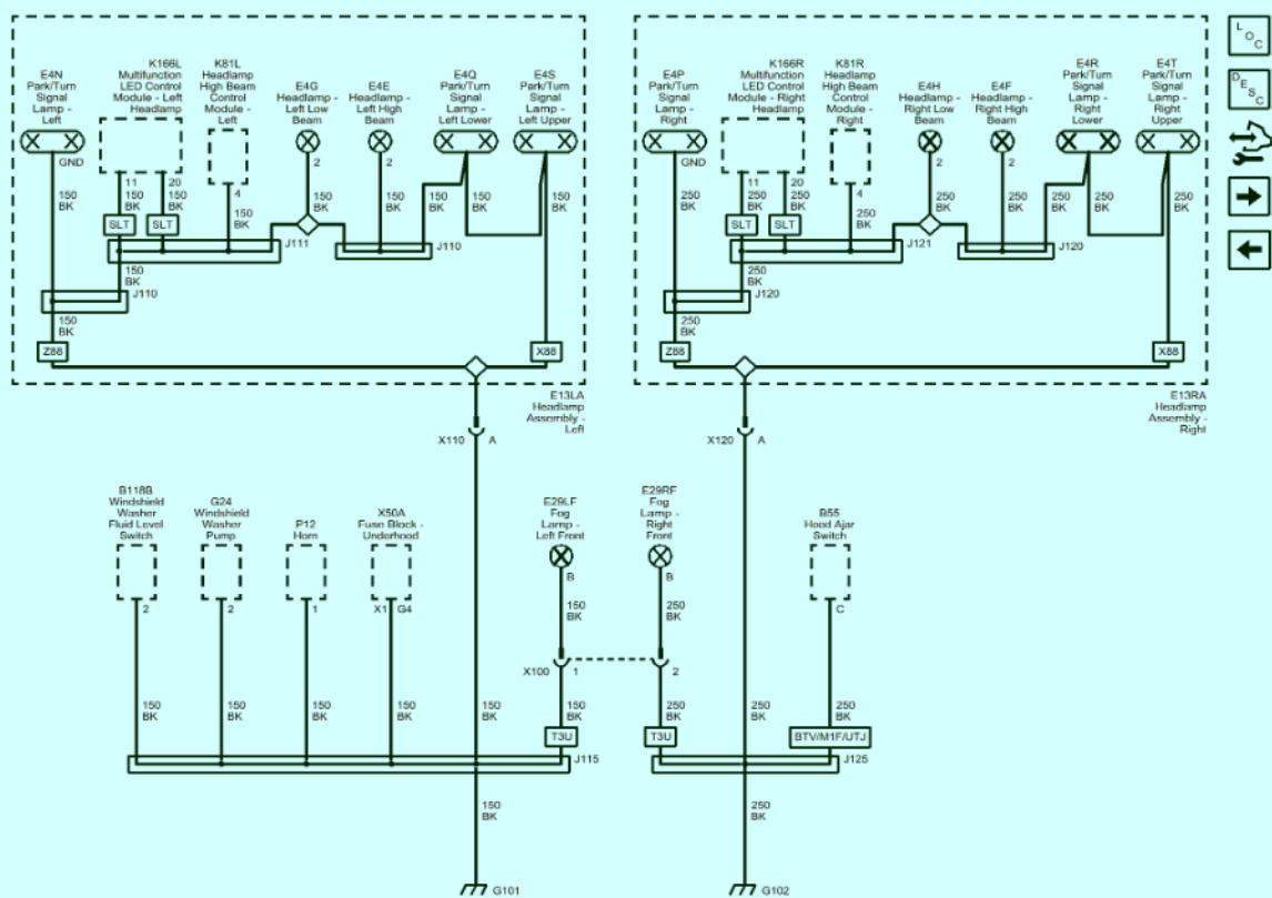
Fig. 2: G101 and G102 (2500/3500) Courtesy of GENERAL MOTORS COMPANY
