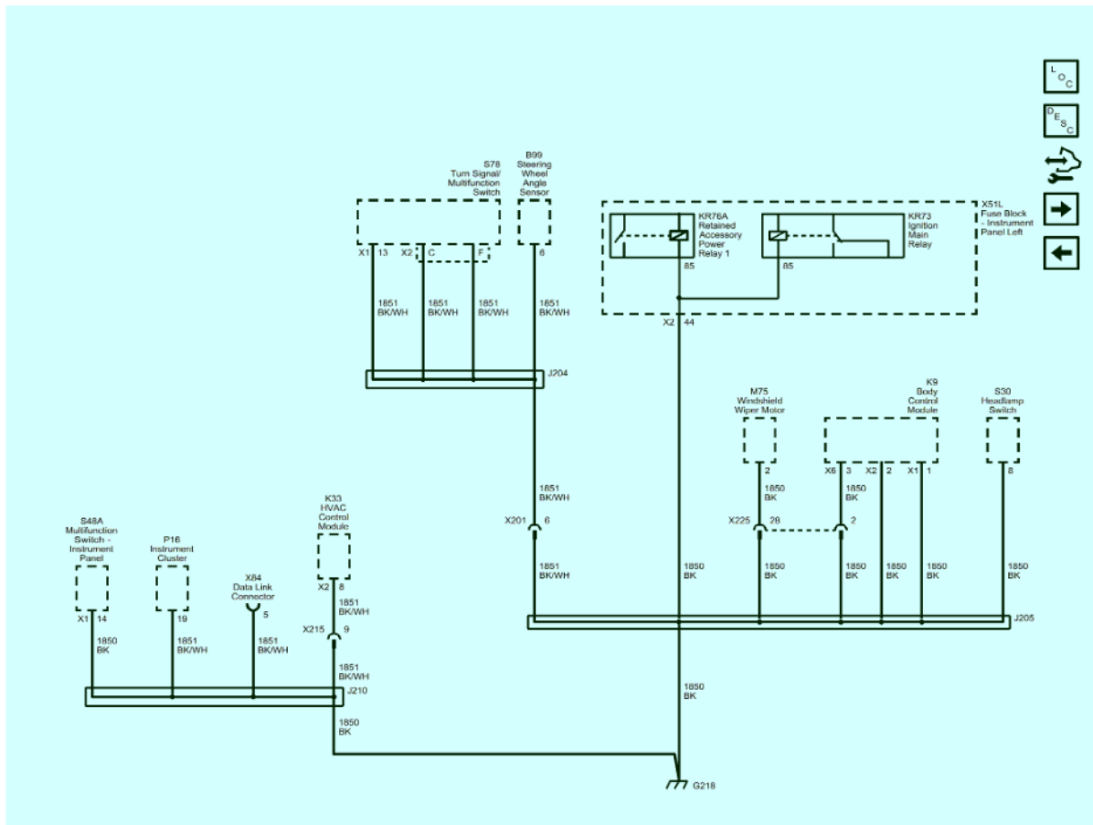
Fig. 13: G218 (2500/3500 with E29) Courtesy of GENERAL MOTORS COMPANY
