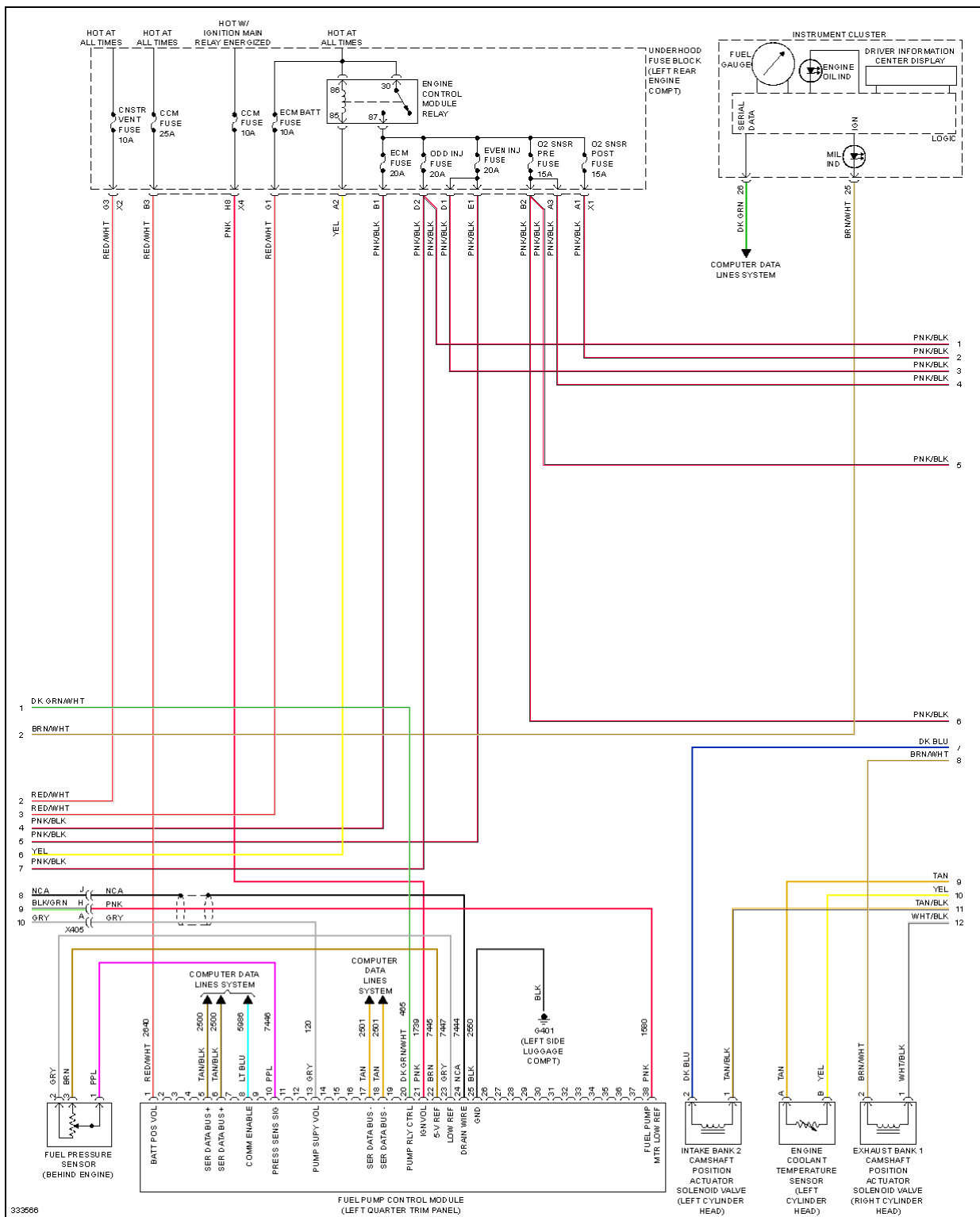
Fig. 25: 3.0L VIN Y, Engine Performance Circuit (2 of 5)
