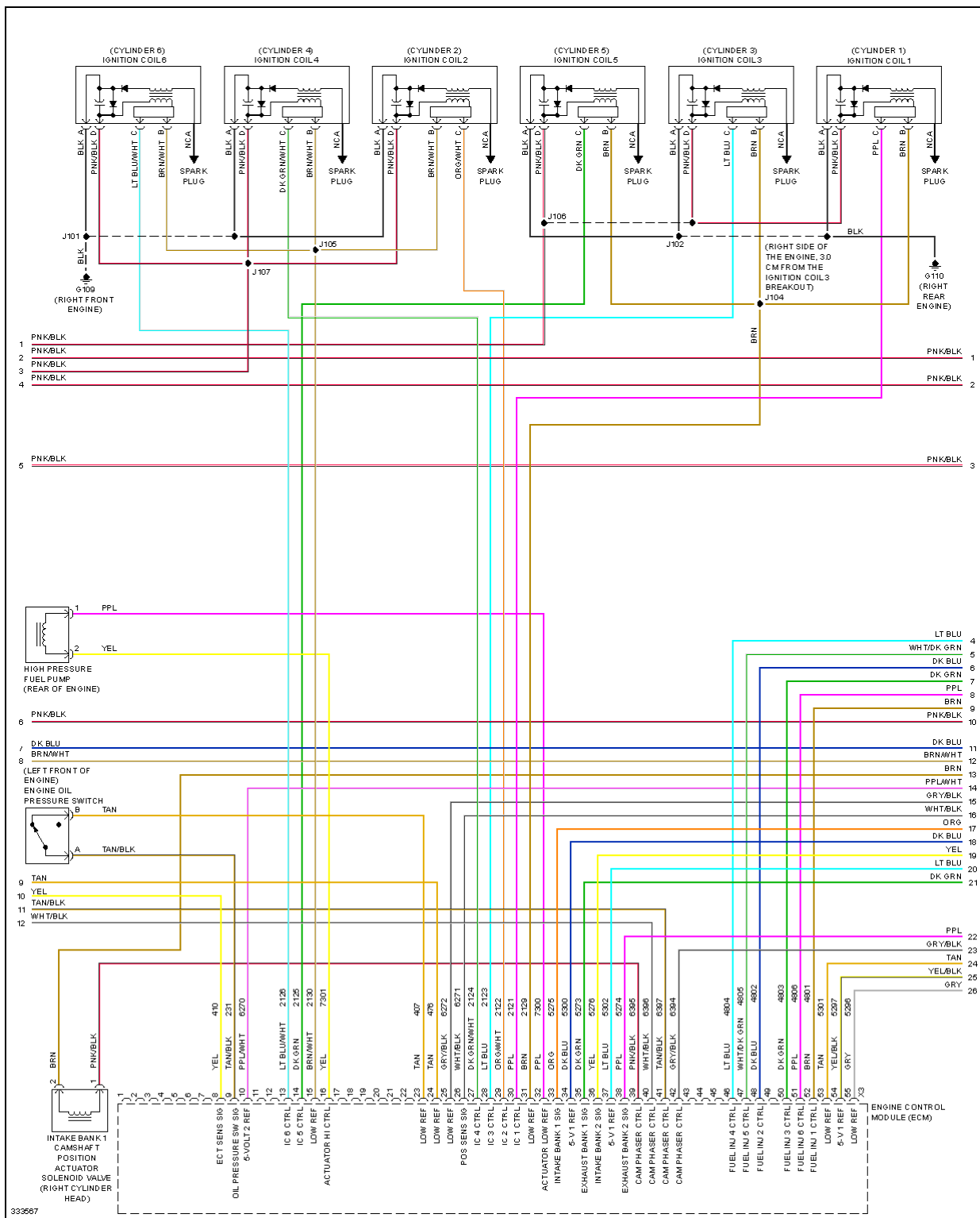
Fig. 26: 3.0L VIN Y, Engine Performance Circuit (3 of 5)
