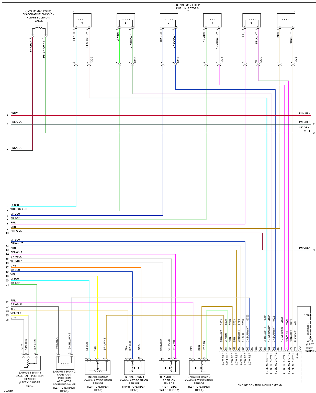
Fig. 27: 3.0L VIN Y, Engine Performance Circuit (4 of 5)
