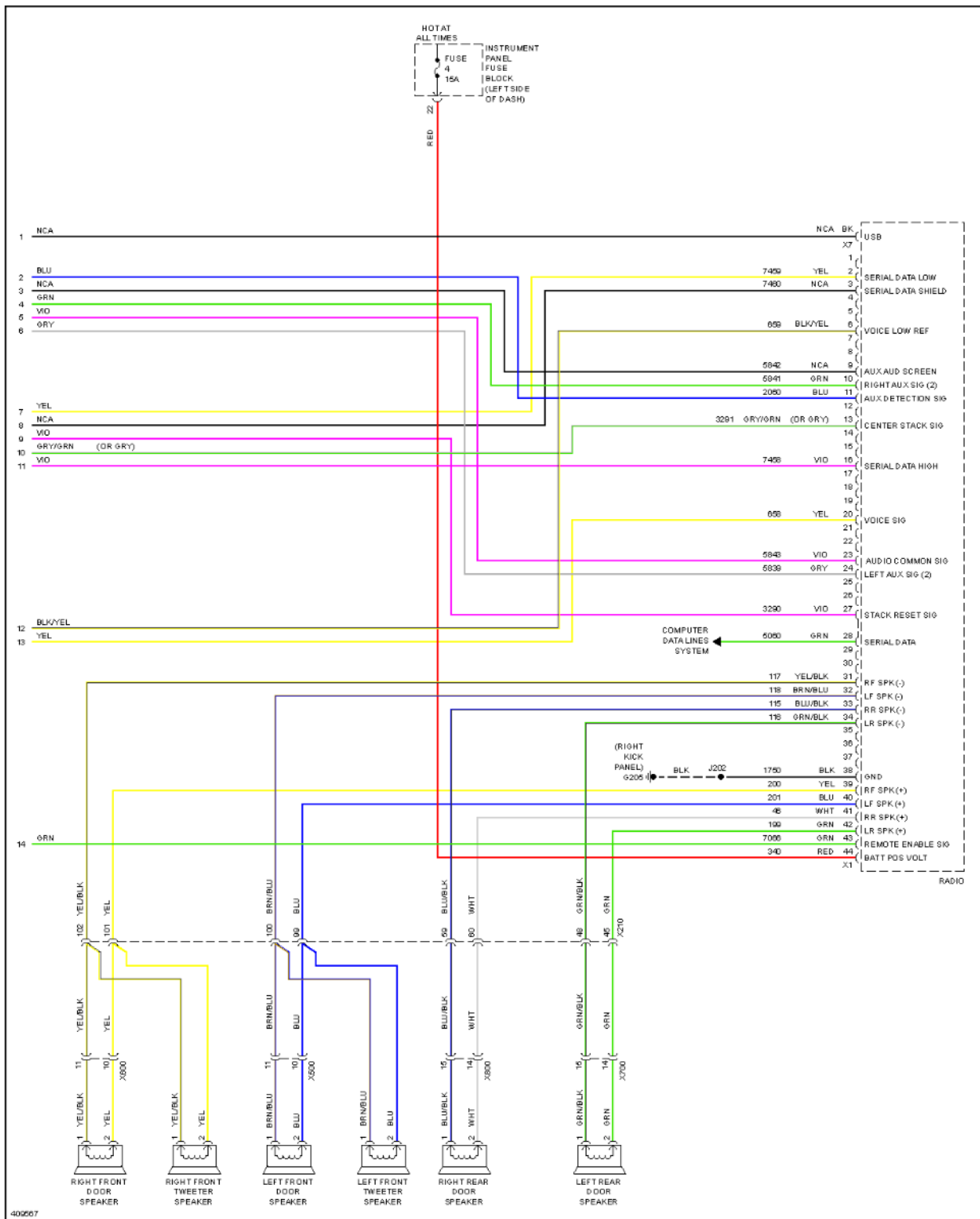
Fig. 85: Navigation Circuit, W/O Amplifier (4 of 4)
