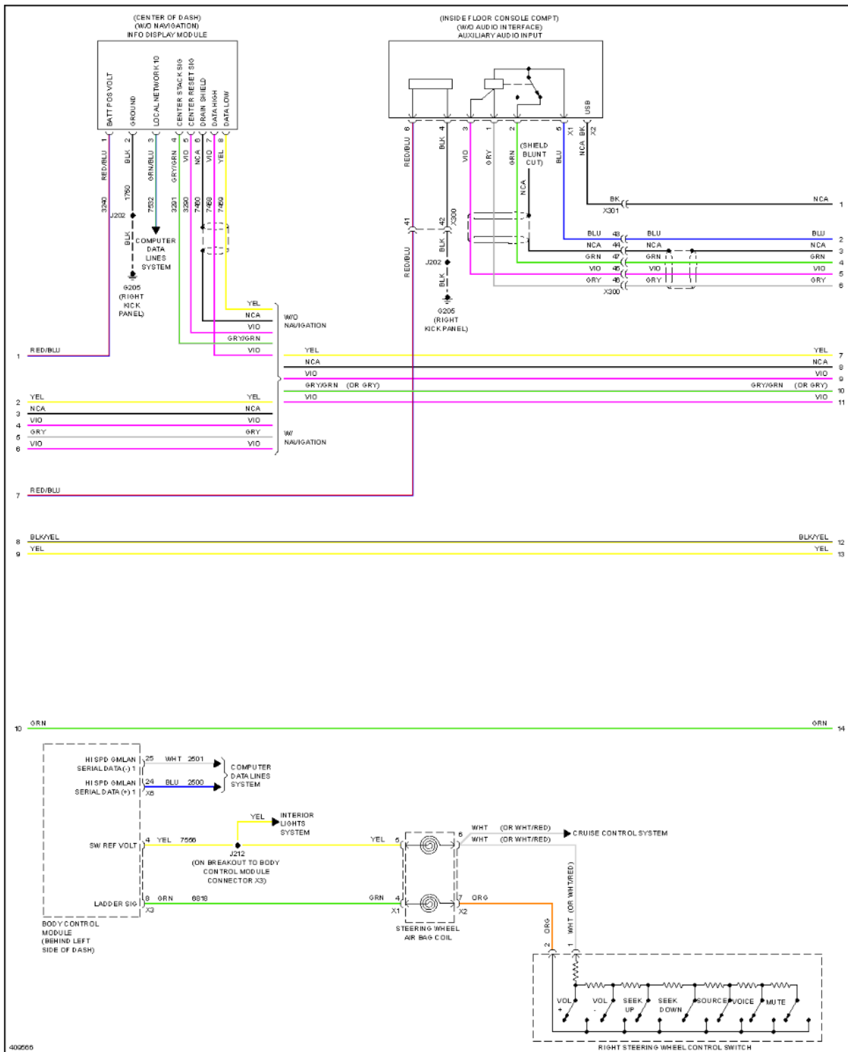
Fig. 84: Navigation Circuit, W/O Amplifier (3 of 4)
