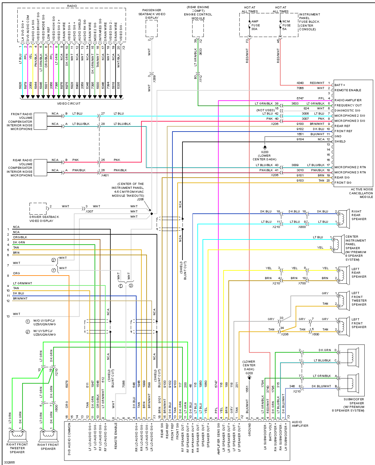
Fig. 67: Radio Circuit (3 of 3)
