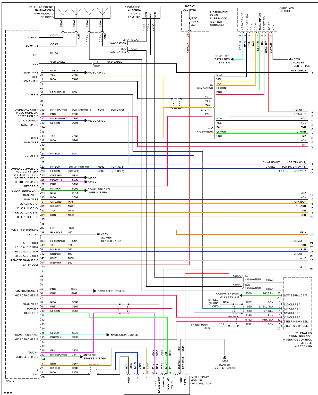
Fig. 65: Radio Circuit (1 of 3)
