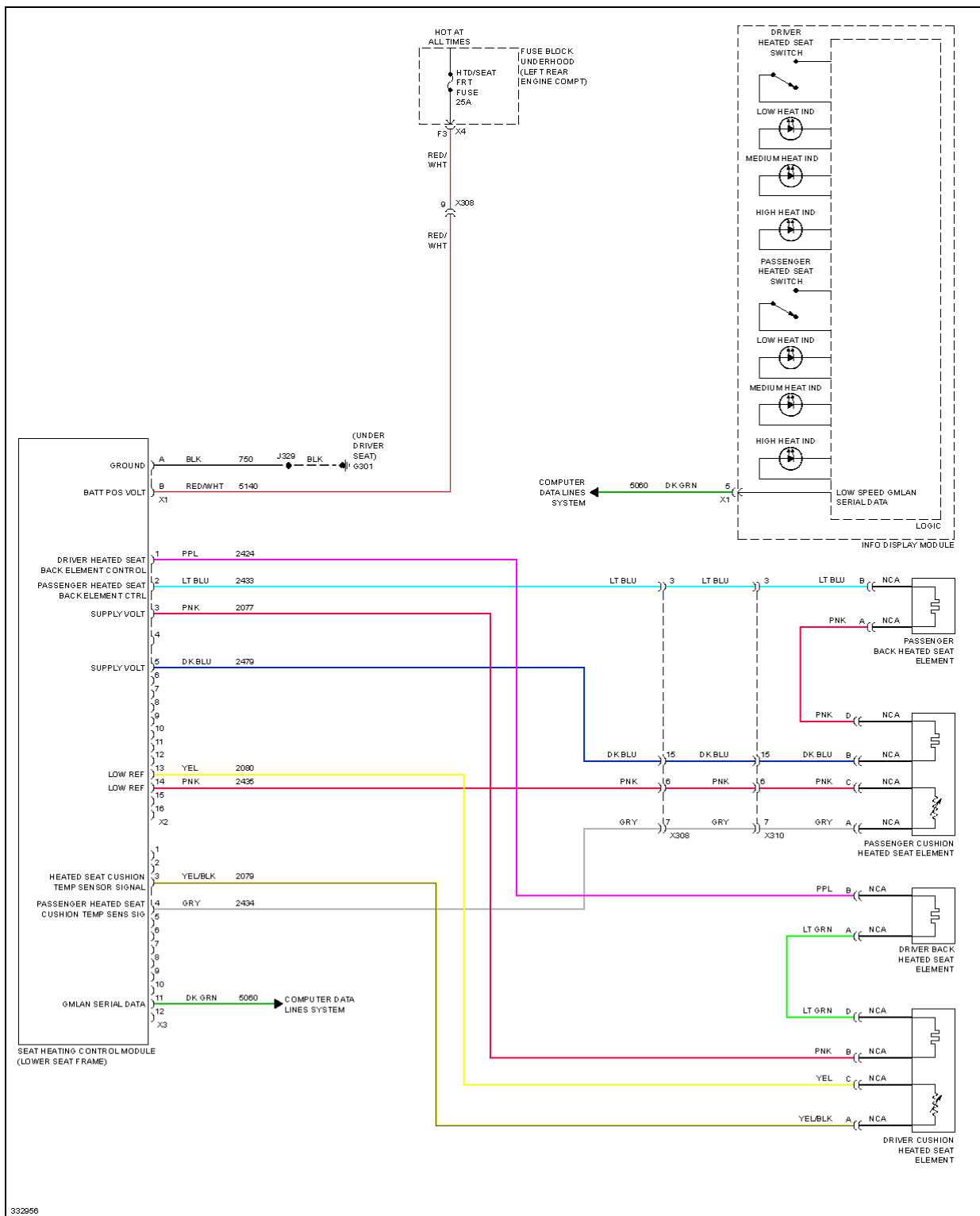
Fig. 60: Heated Seats Circuit, W/O SPO Heated Seats & Memory
