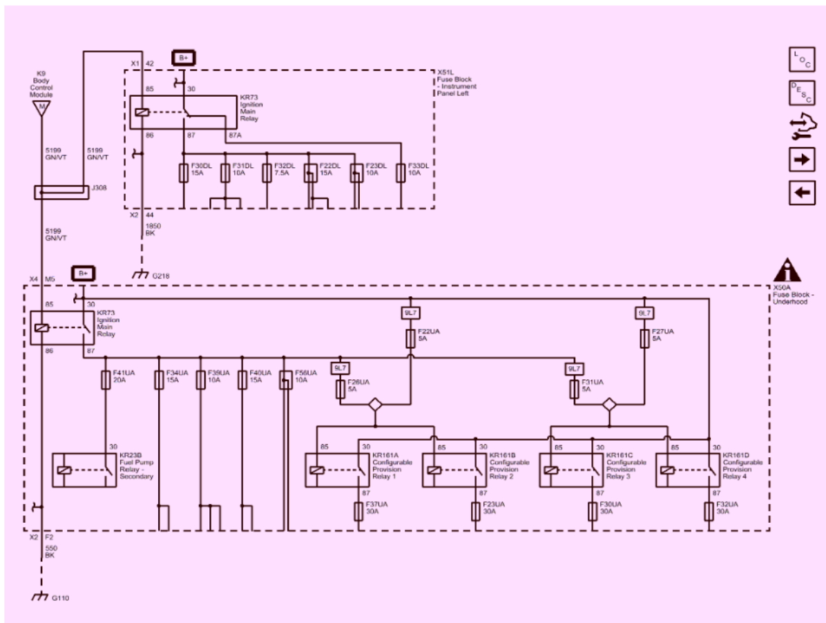
Fig. 2: Ignition Main Relays
