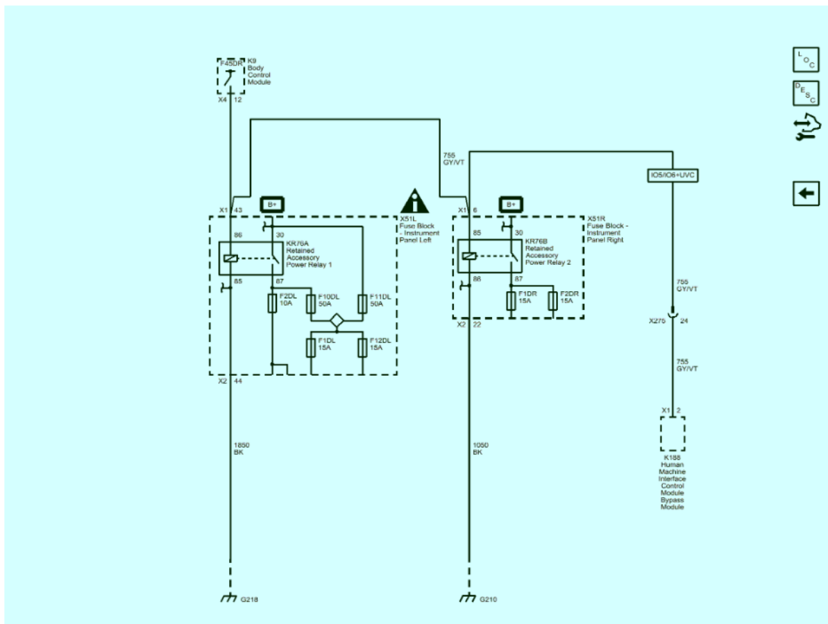
Fig. 3: Retained Accessory Power Relays Courtesy of GENERAL MOTORS COMPANY
