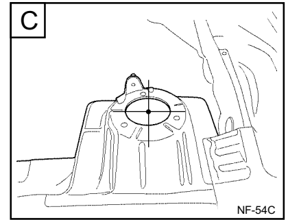
Front strut hole (Ø85)
