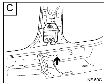
Seat belt lower anchor mounting hole (Ø 15)
