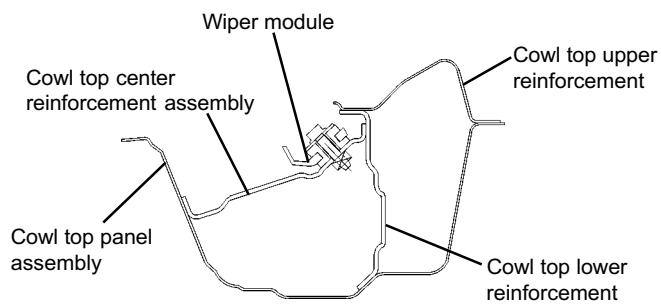
SECTION C-C'
