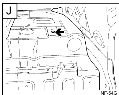
Seat belt retractor mounting hole (Ø 15)
