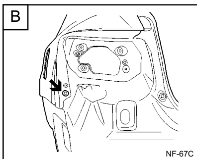
Rear combination lamp mounting hole (Ø 14)
