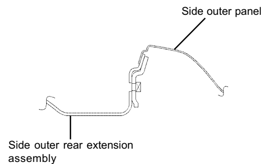
SECTION D-D'
