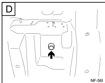
Sub frame rear mounting pipe nut (Ø 14)
