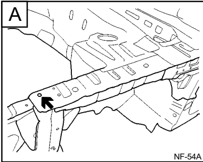
Front end module mounting hole Ø 13)
