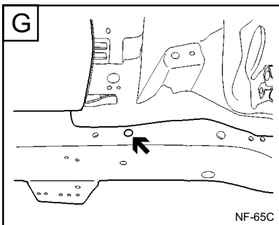
Engine mountin gbracket mount- ing hole (Ø13)
