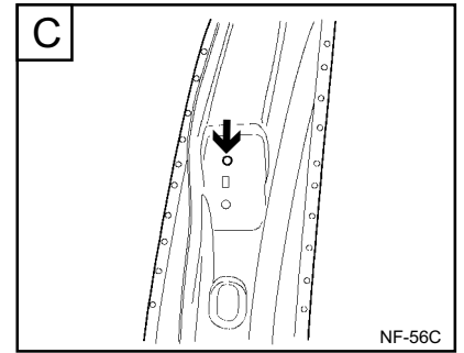
Rear door hinge upper mounting hole (Ø 13)
