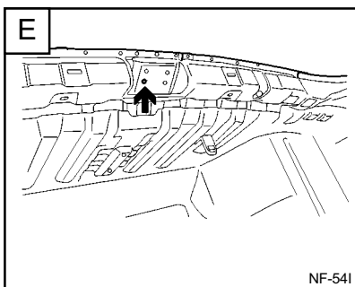
Trunk lid striker mounting hole (Ø 9)
