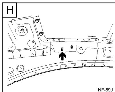
Rear assist handle bracket mounting bolt (Ø 15)
