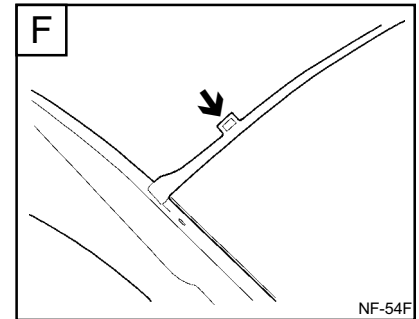
Rear glass right stopper hole (□ 7x15)
