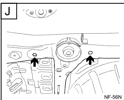
Rear cross member holes (Ø 17)
