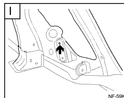
Rear seat tilting hinge mounting hole (Ø 6.6)
