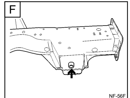
Sub frame front mounting pipe nut (Ø 14)
