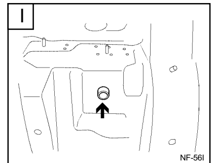
Sub frame rear mounting pipe nut (Ø 14)
