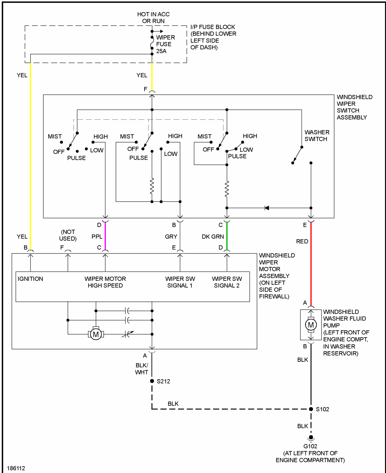
Fig. 43: Pulse Wiper/Washer Circuit
