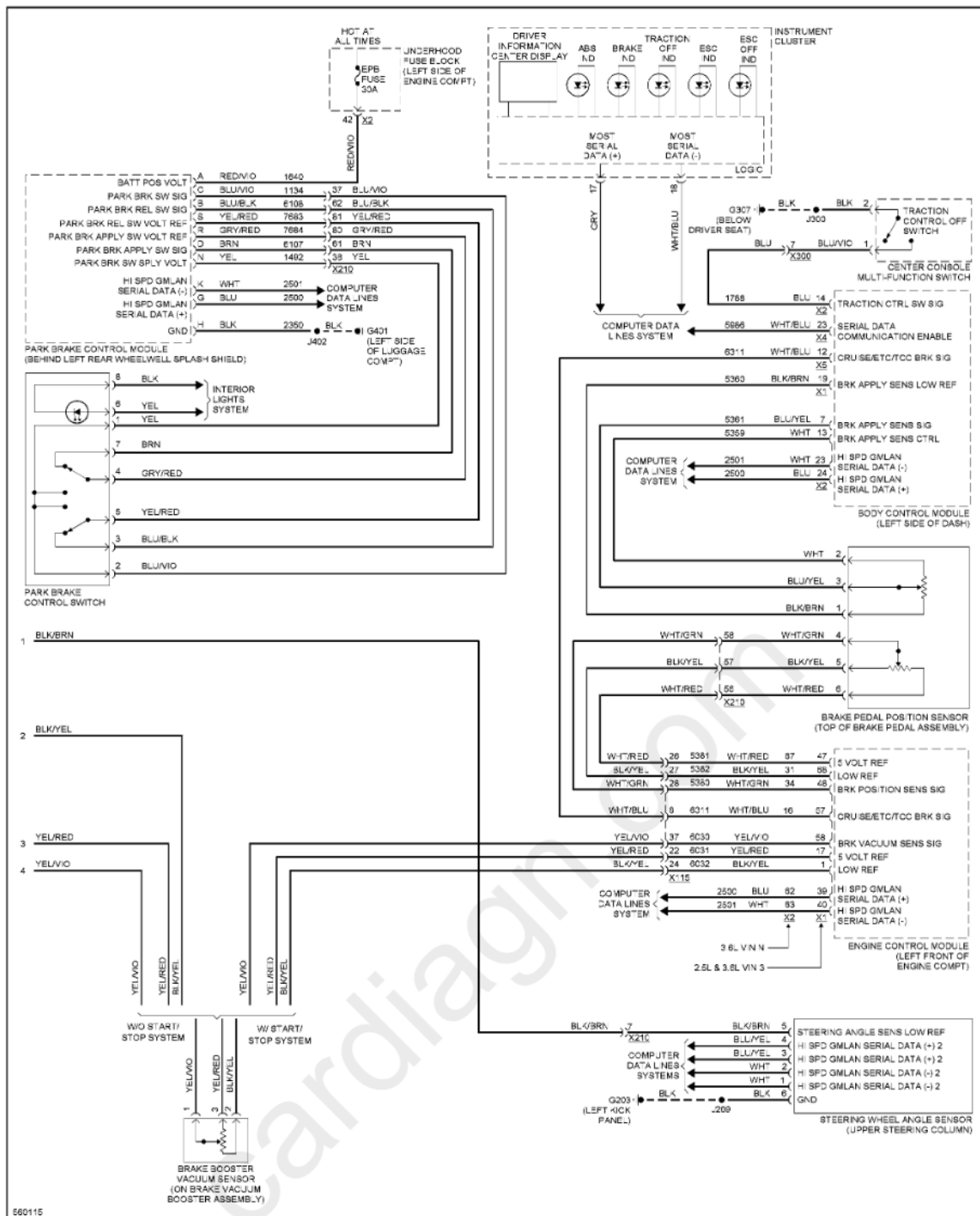
Fig. 10: Anti-lock Brakes Circuit (2 of 2)
