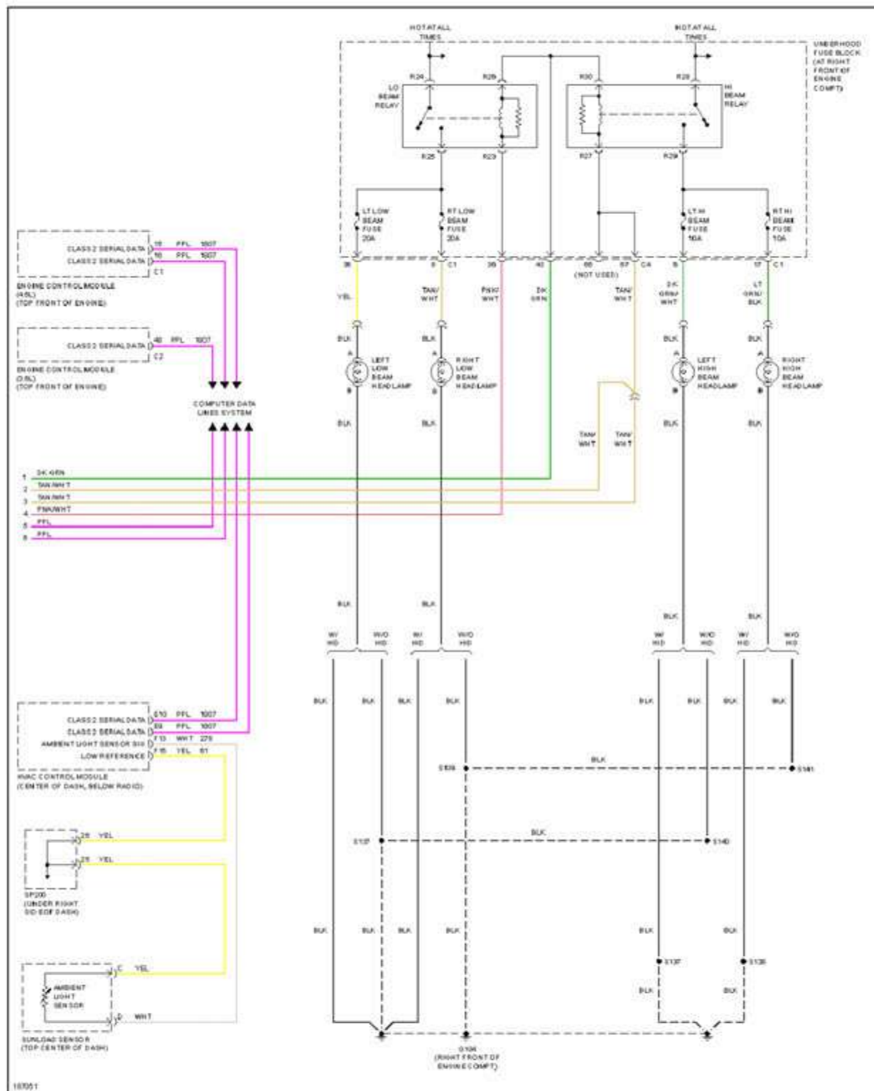
Fig. 35: Headlights Circuit (2 of 2)
