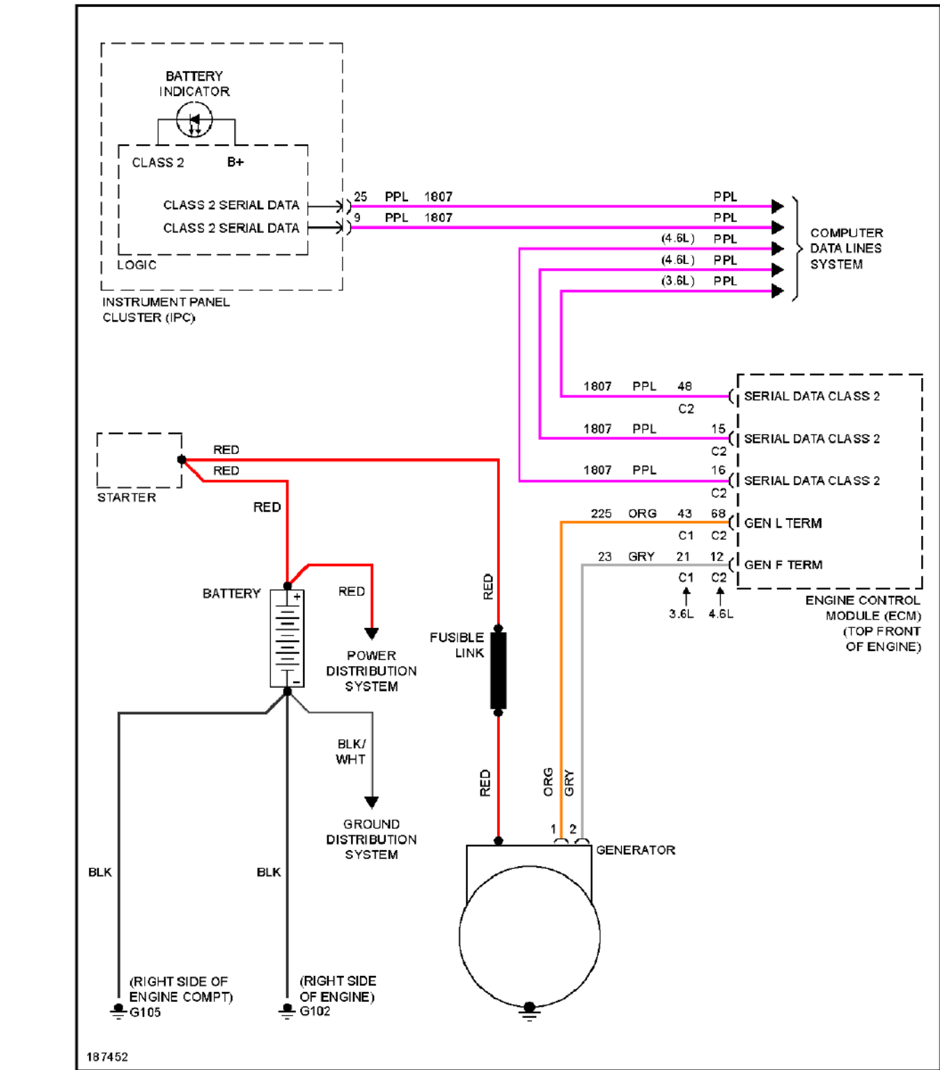
Fig. 79: Charging Circuit
