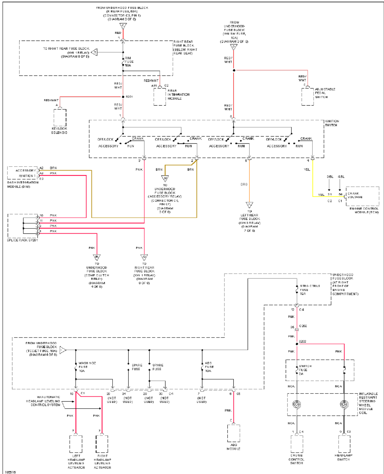
Fig. 53: Power Distribution Circuit (5 of 8)
