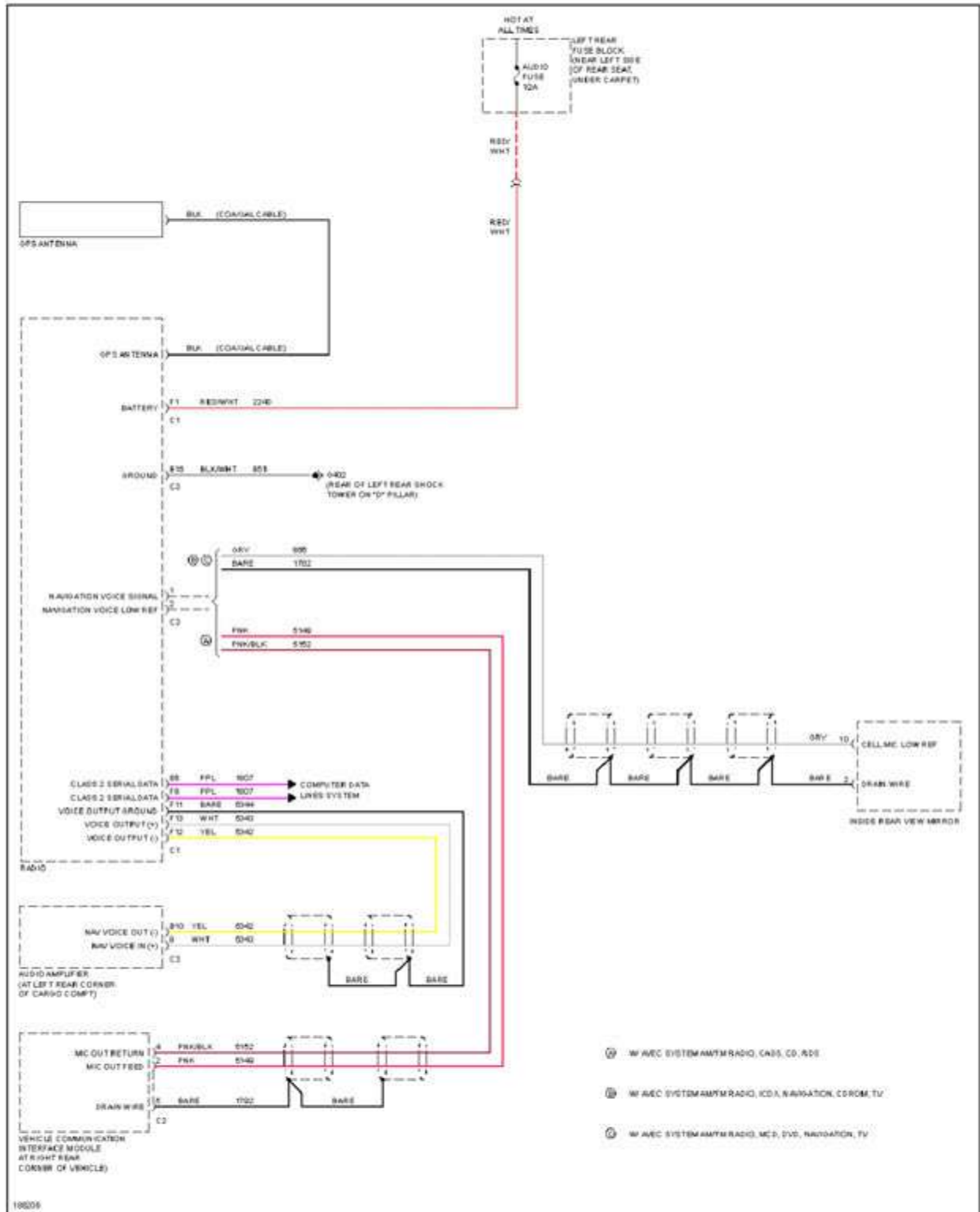
Fig. 47: Navigation Circuit
