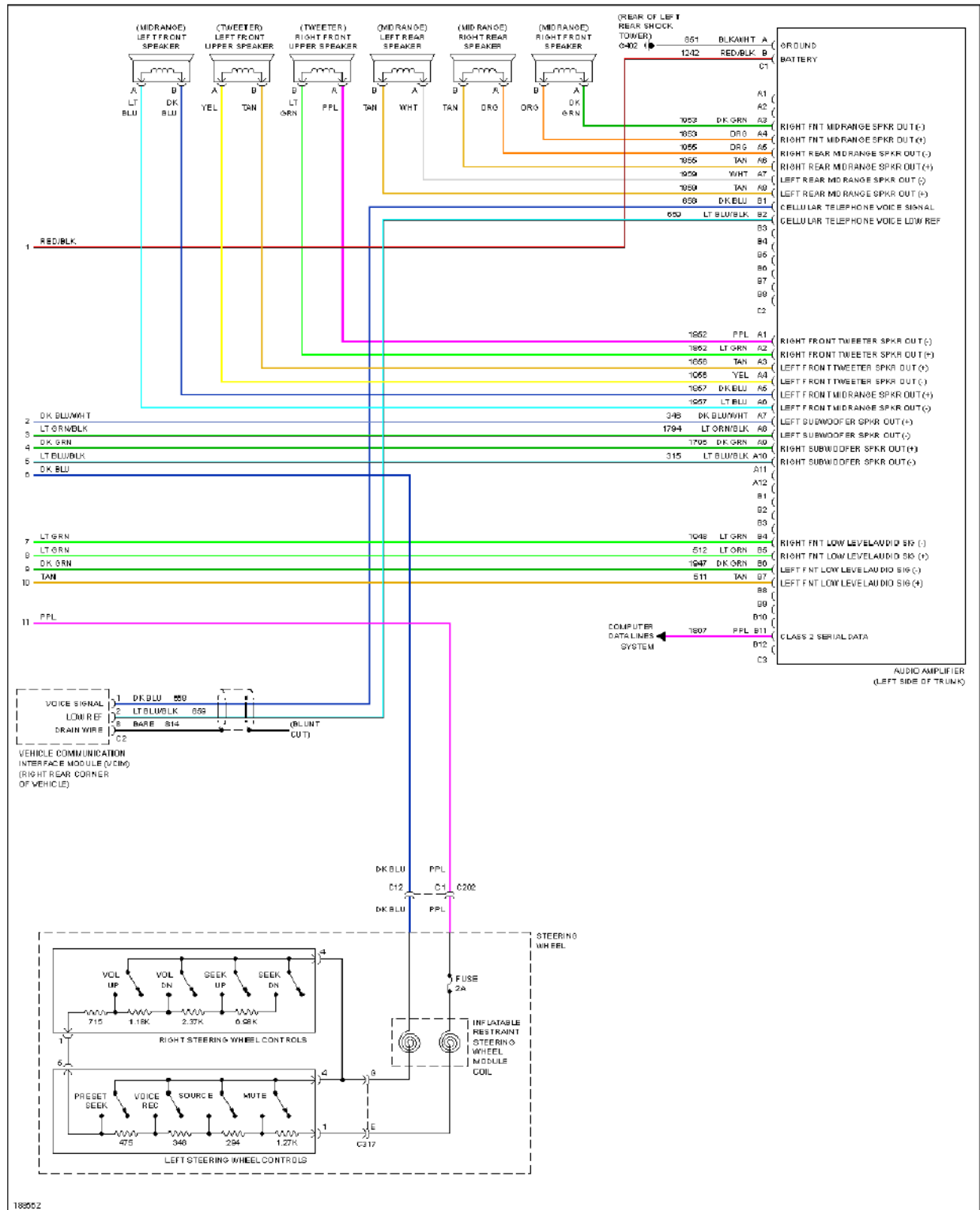
Fig. 70: Base Radio Circuit (2 of 2)
