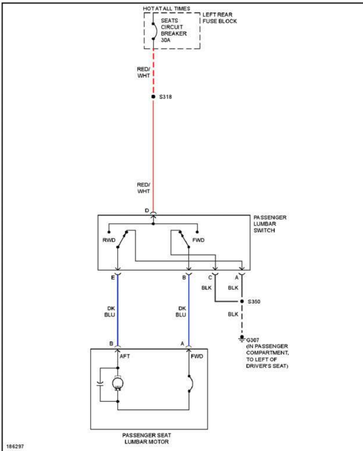
Fig. 63: Passenger's Lumbar Circuit
