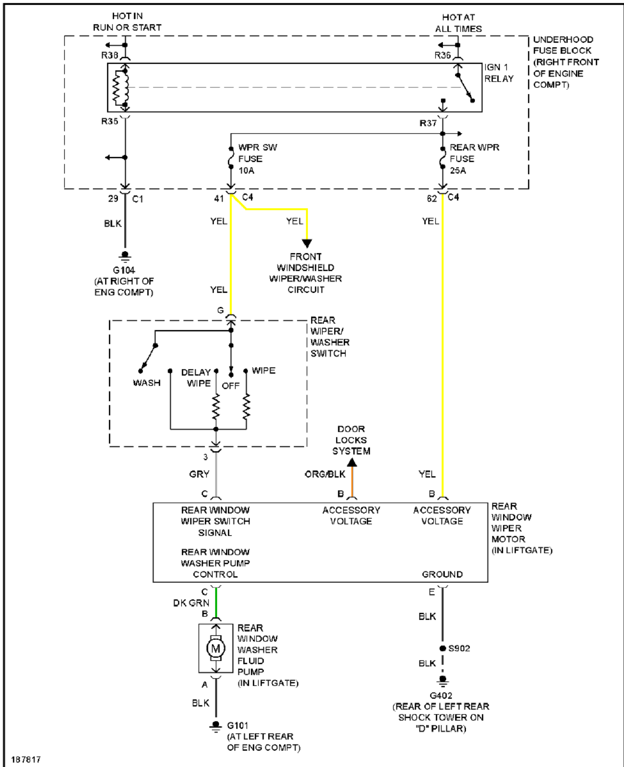
Fig. 87: Rear Wiper/Washer Circuit
