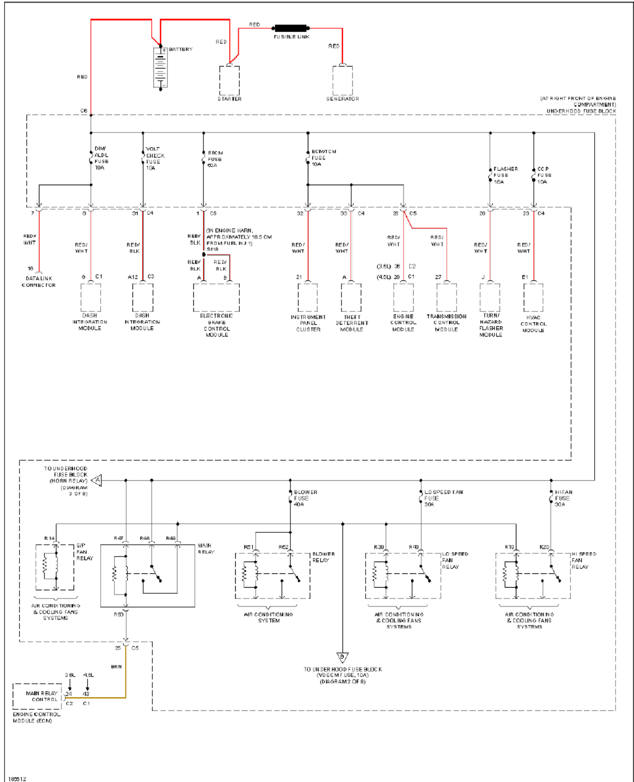
Fig. 49: Power Distribution Circuit (1 of 8)
