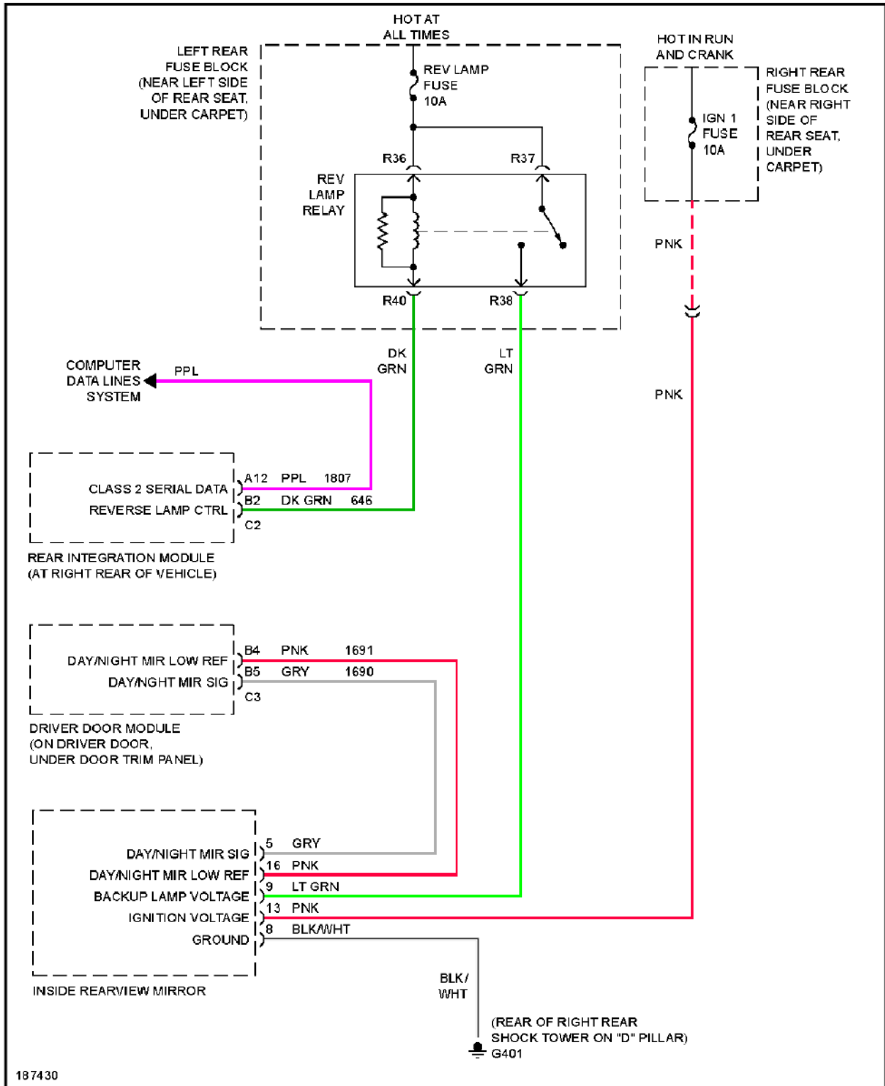
Fig. 59: Automatic Day/Night Mirror Circuit
