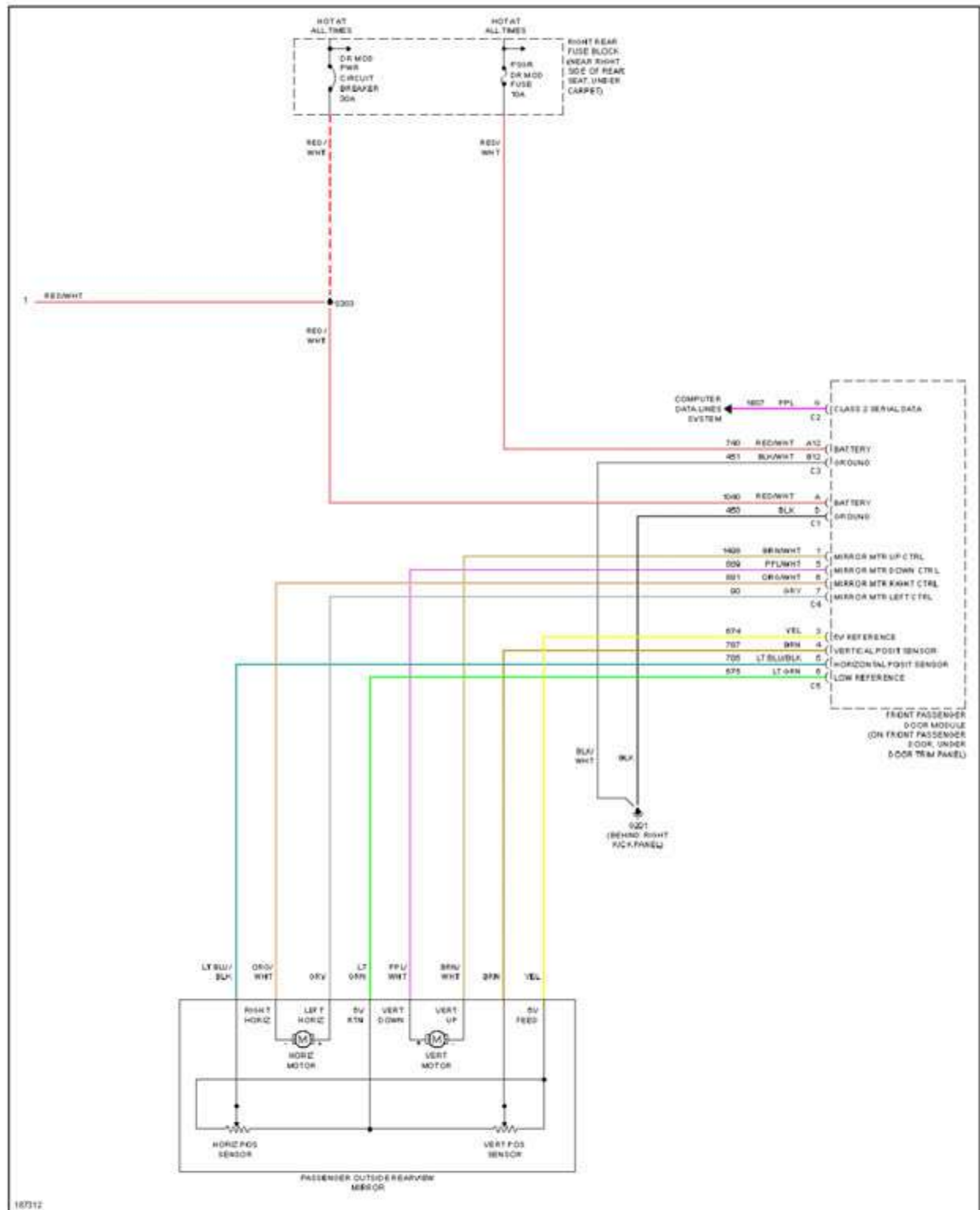
Fig. 44: Memory Mirrors Circuit (2 of 2)
