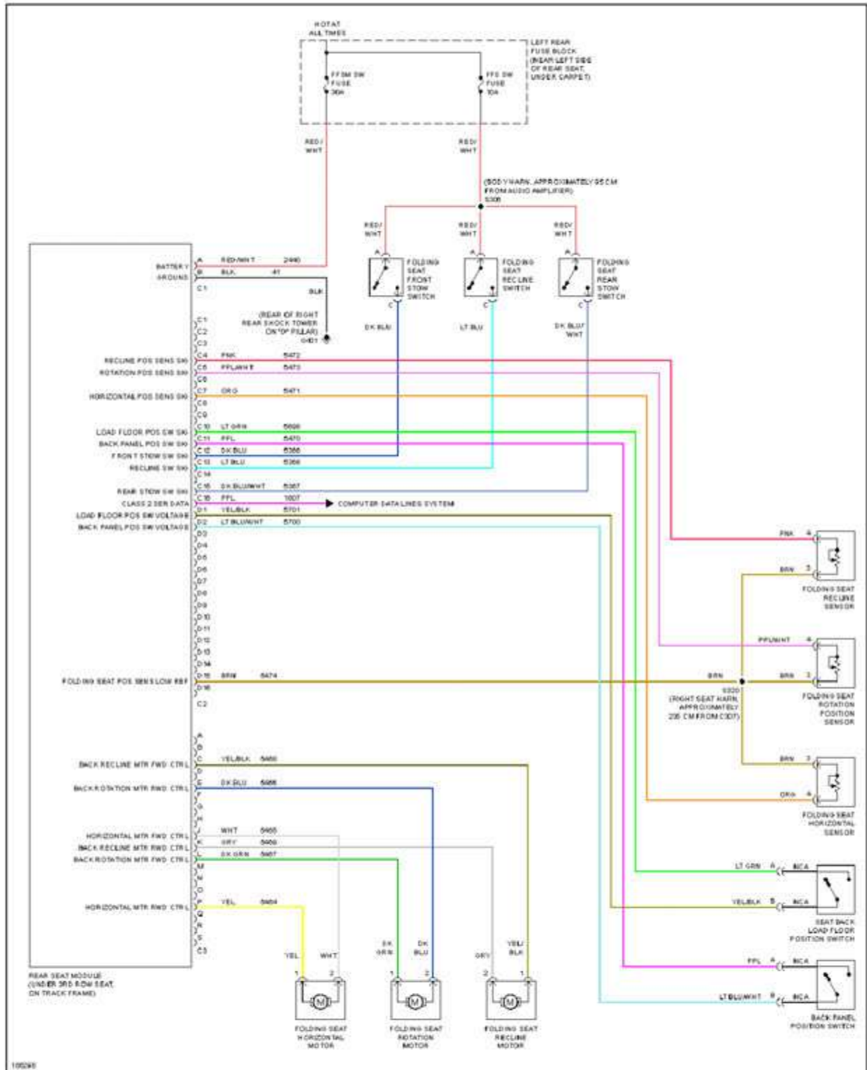
Fig. 64: Rear Power Seat Circuit
