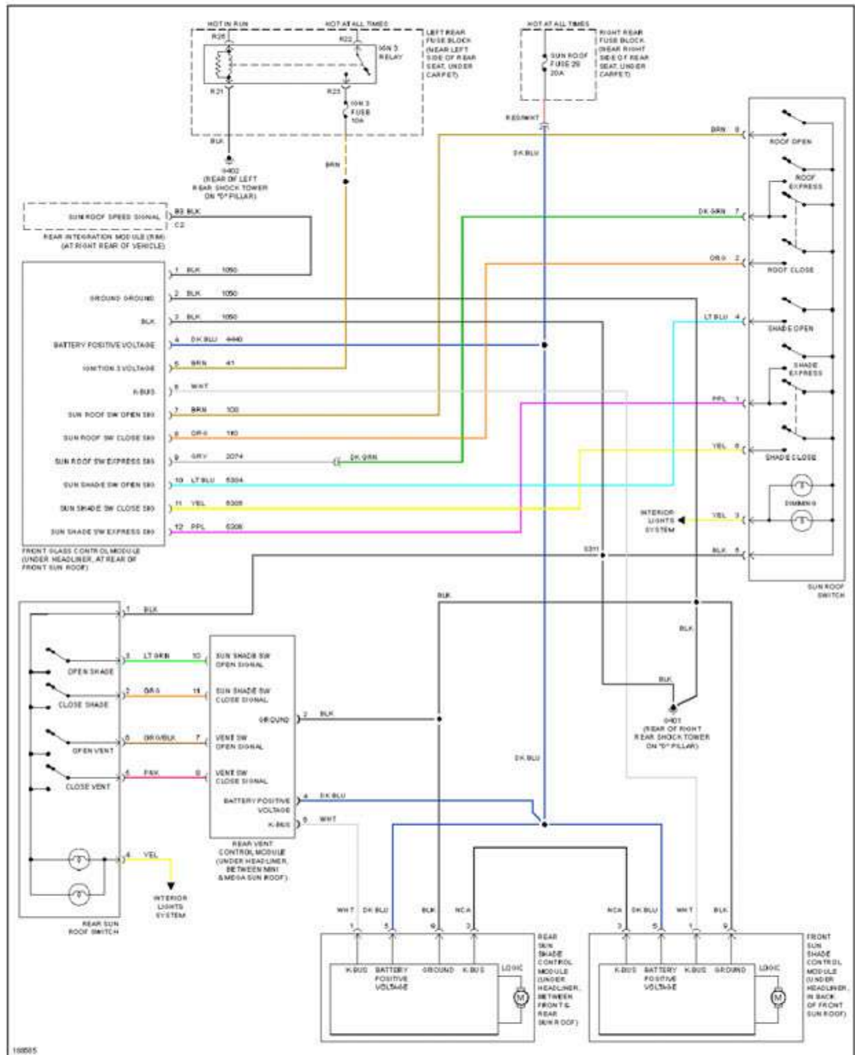
Fig. 65: Sunroof Circuit, W/ Mega Sunroof
