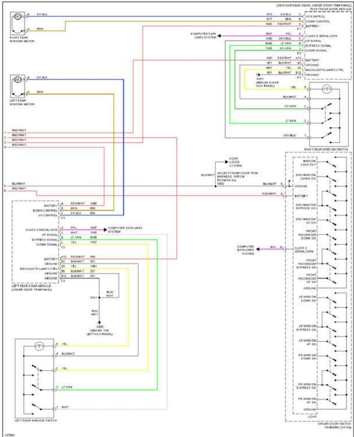
Fig. 68: Power Windows Circuit (2 of 2)
