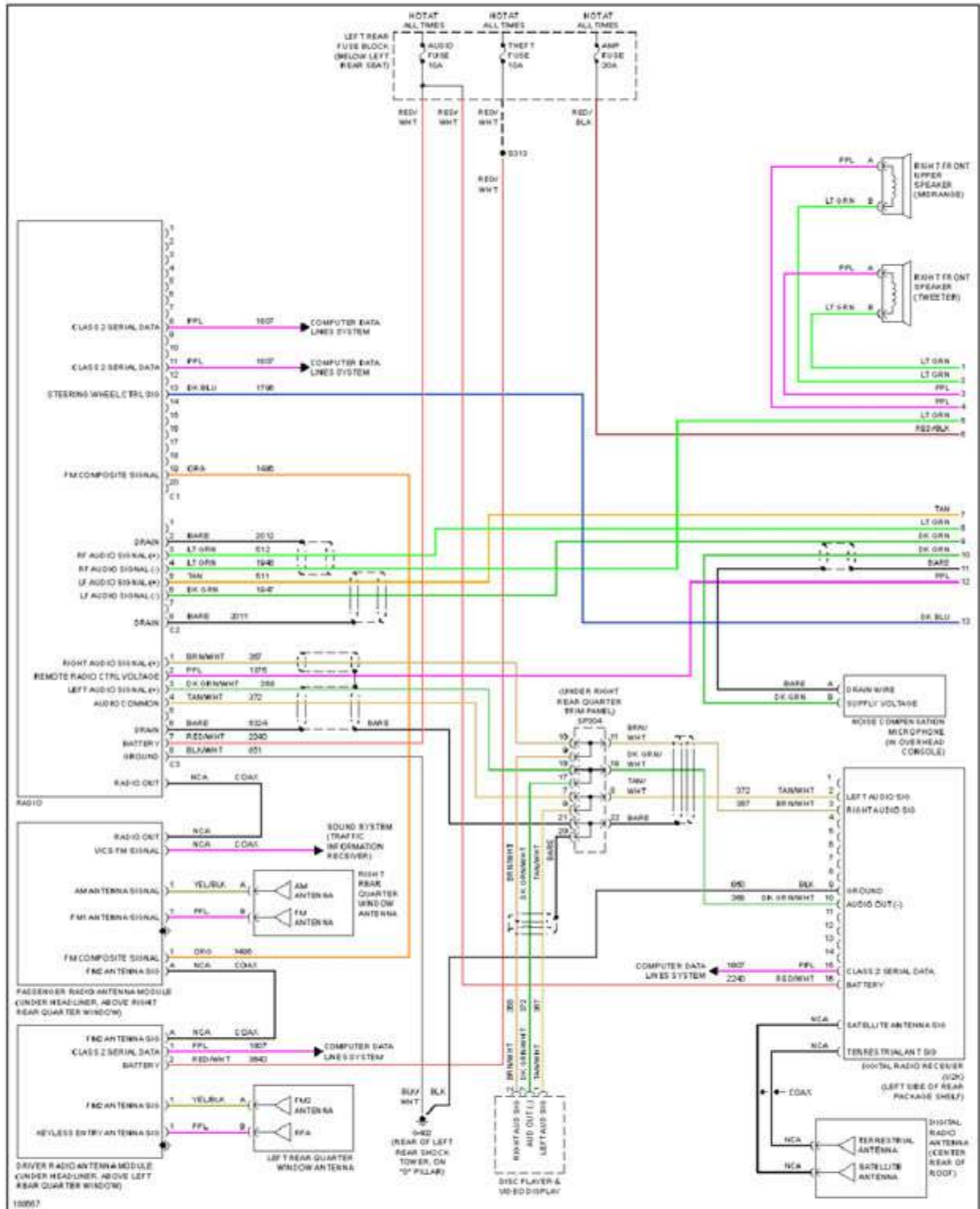
Fig. 73: Premium Sound Radio Circuit, W/O CD Changer (1 of 2)
