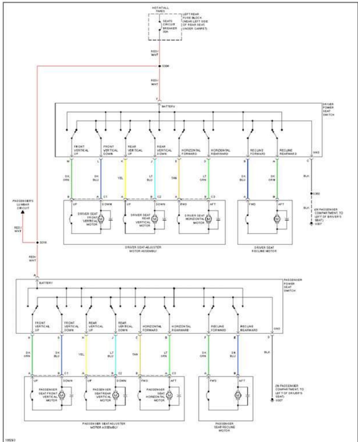
Fig. 61: Front Power Seat Circuit
