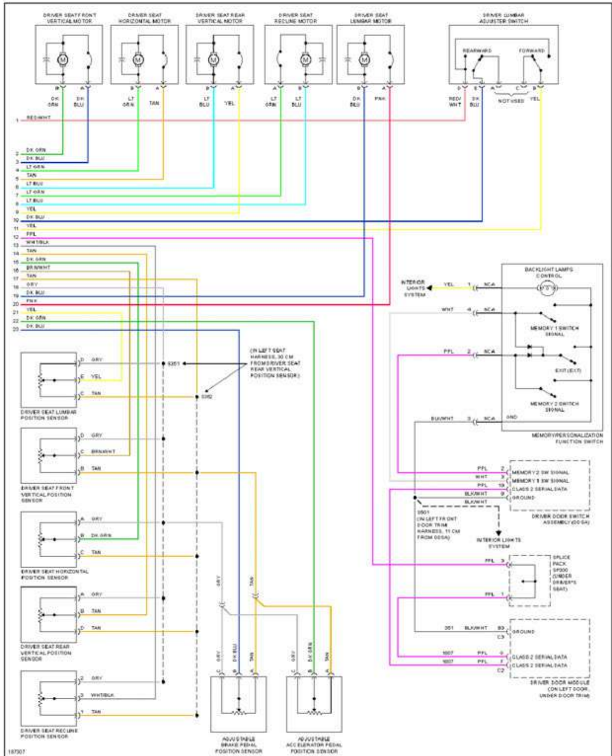
Fig. 46: Memory Seat Circuit (2 of 2)
