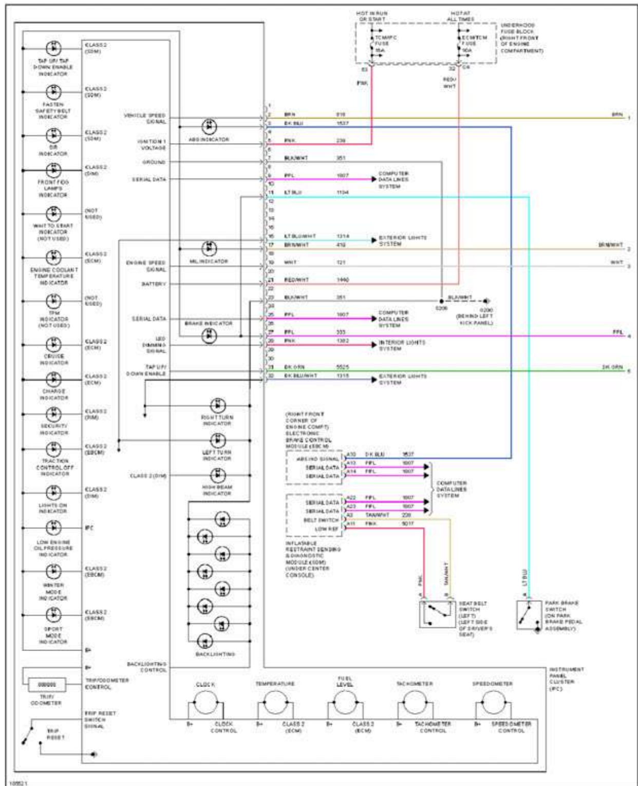
Fig. 37: 3.6L VIN 7, Instrument Cluster Circuit (1 of 2)
