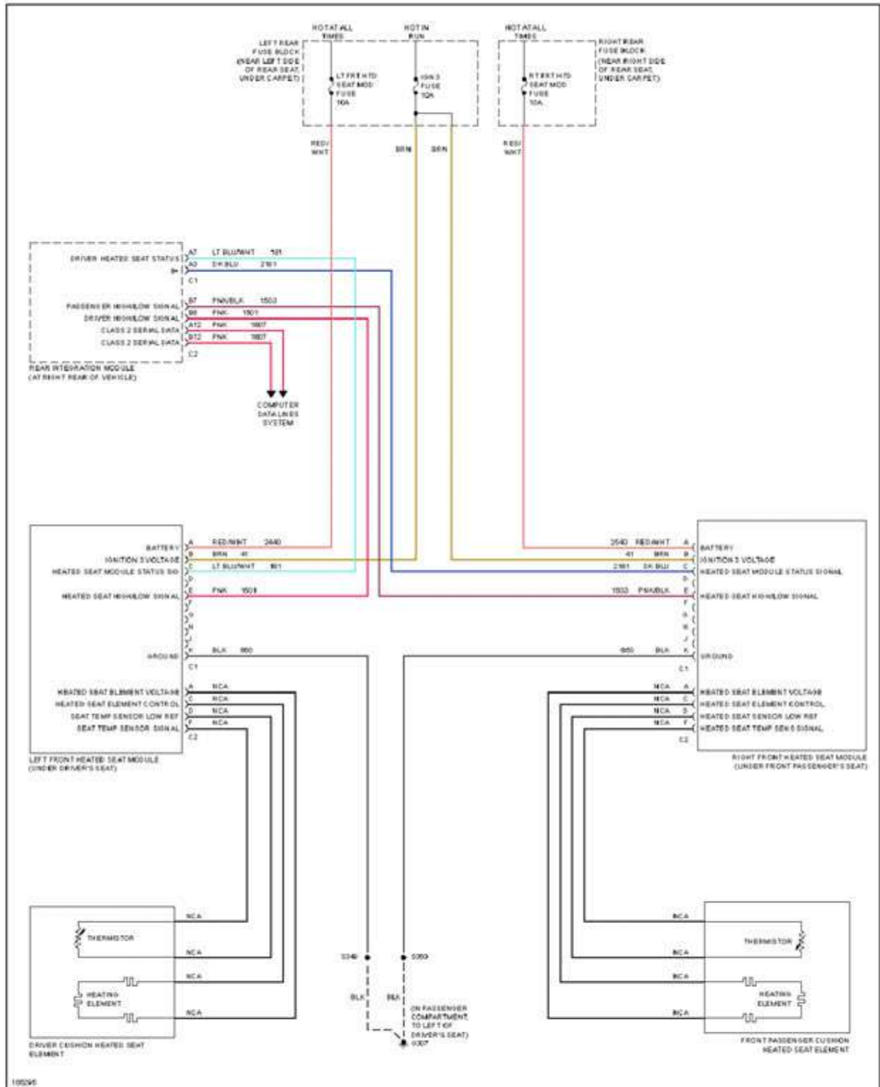
Fig. 62: Heated Seats Circuit
