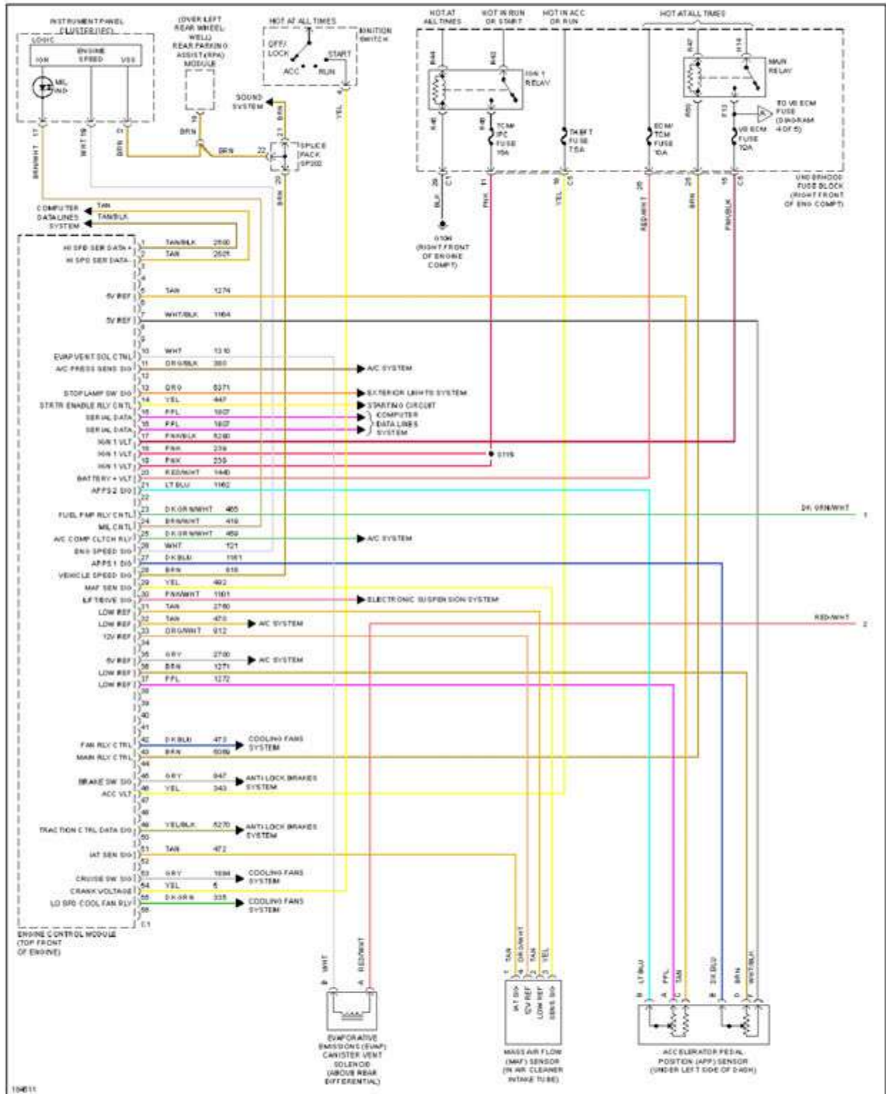
Fig. 23: 4.6L VIN A, Engine Performance Circuit (1 of 5)
