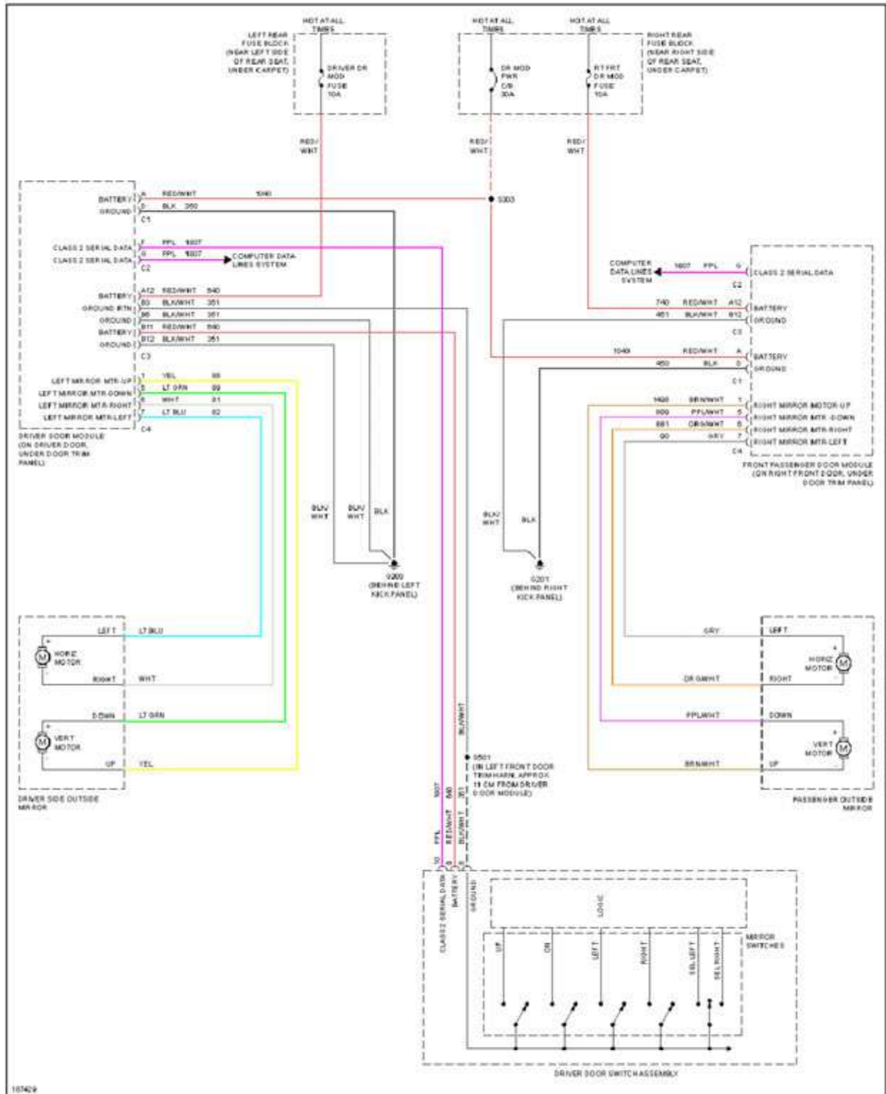
Fig. 60: Power Mirrors Circuit
