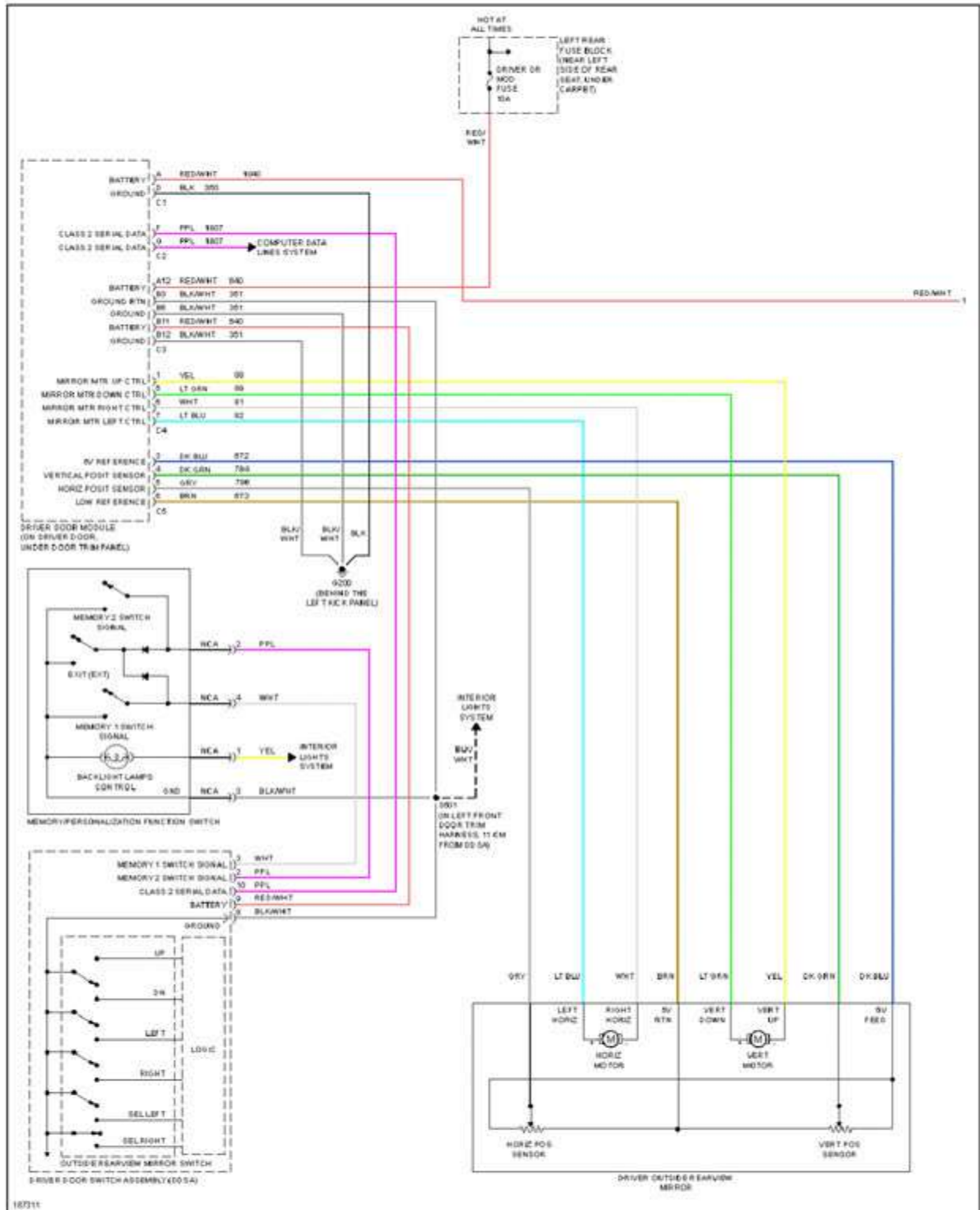
Fig. 43: Memory Mirrors Circuit (1 of 2)
