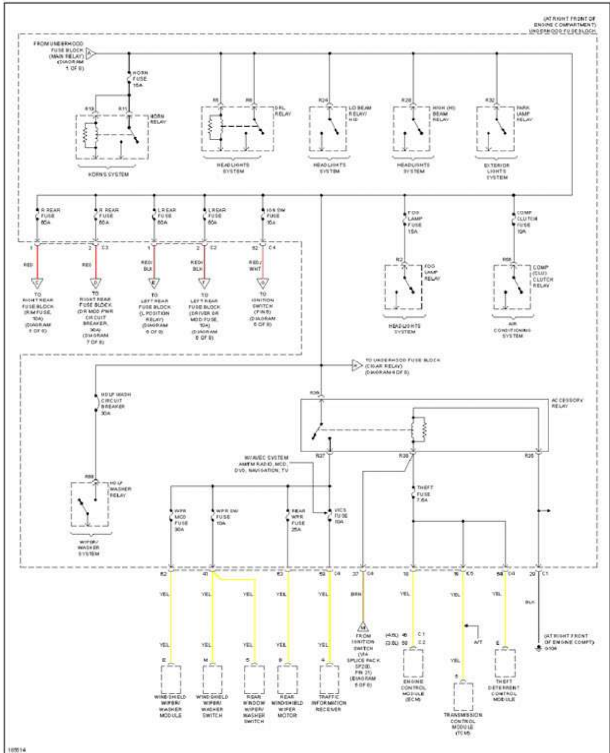
Fig. 51: Power Distribution Circuit (3 of 8)
