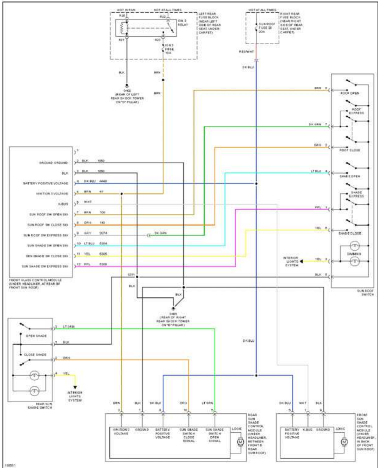
Fig. 66: Sunroof Circuit, W/O Mega Sunroof
