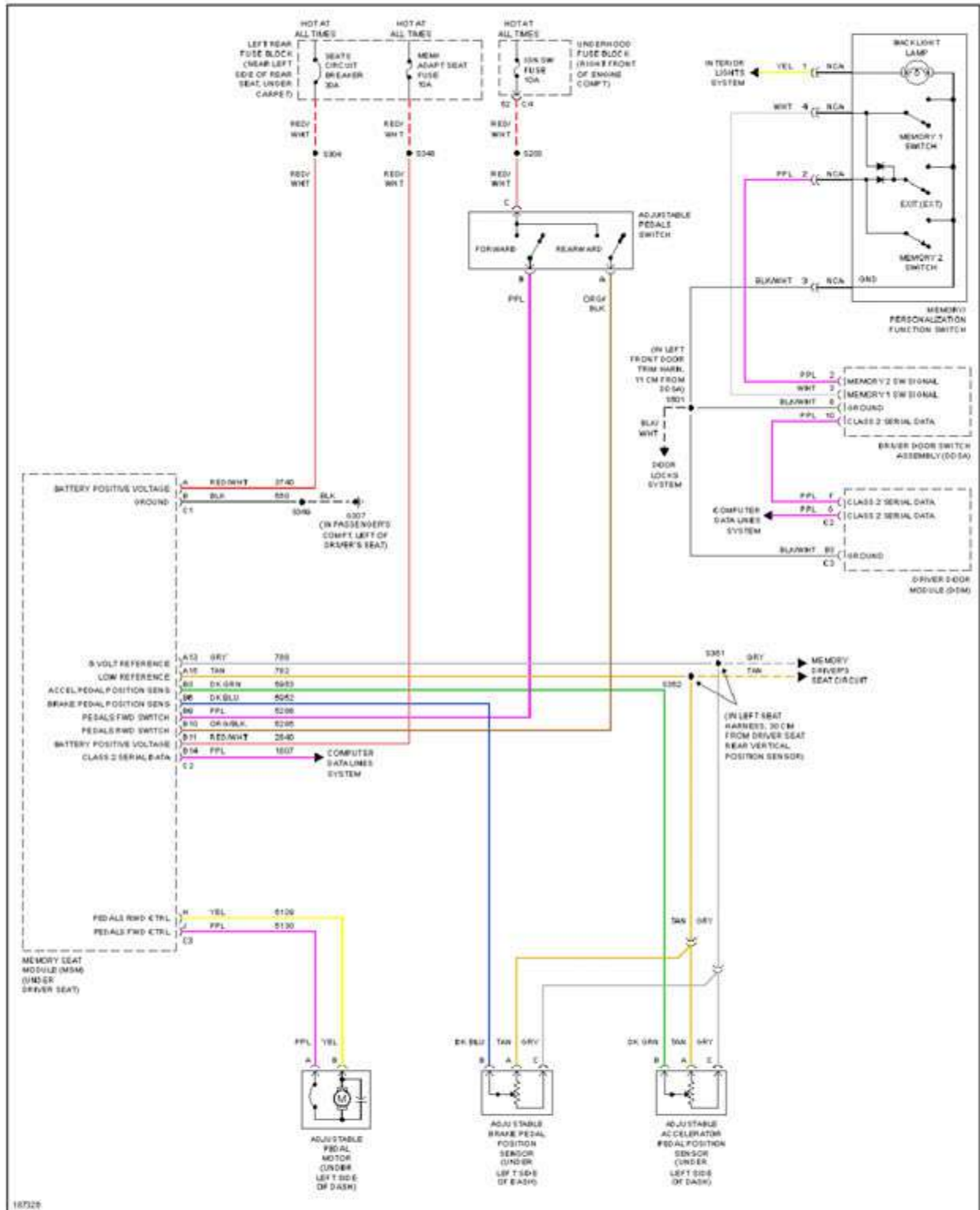
Fig. 42: Adjustable Pedal Circuit
