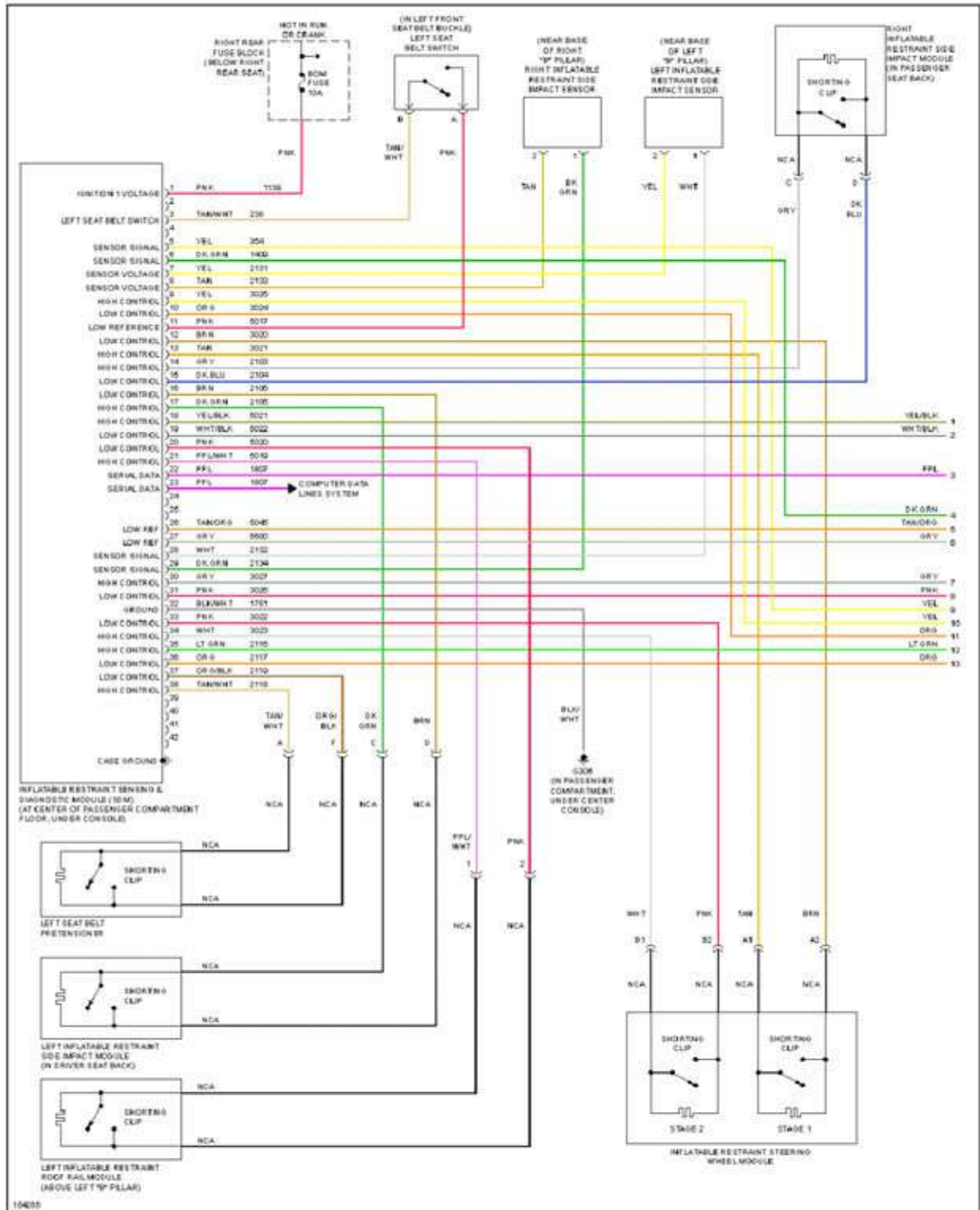
Fig. 81: Supplemental Restraints Circuit (1 of 2)
