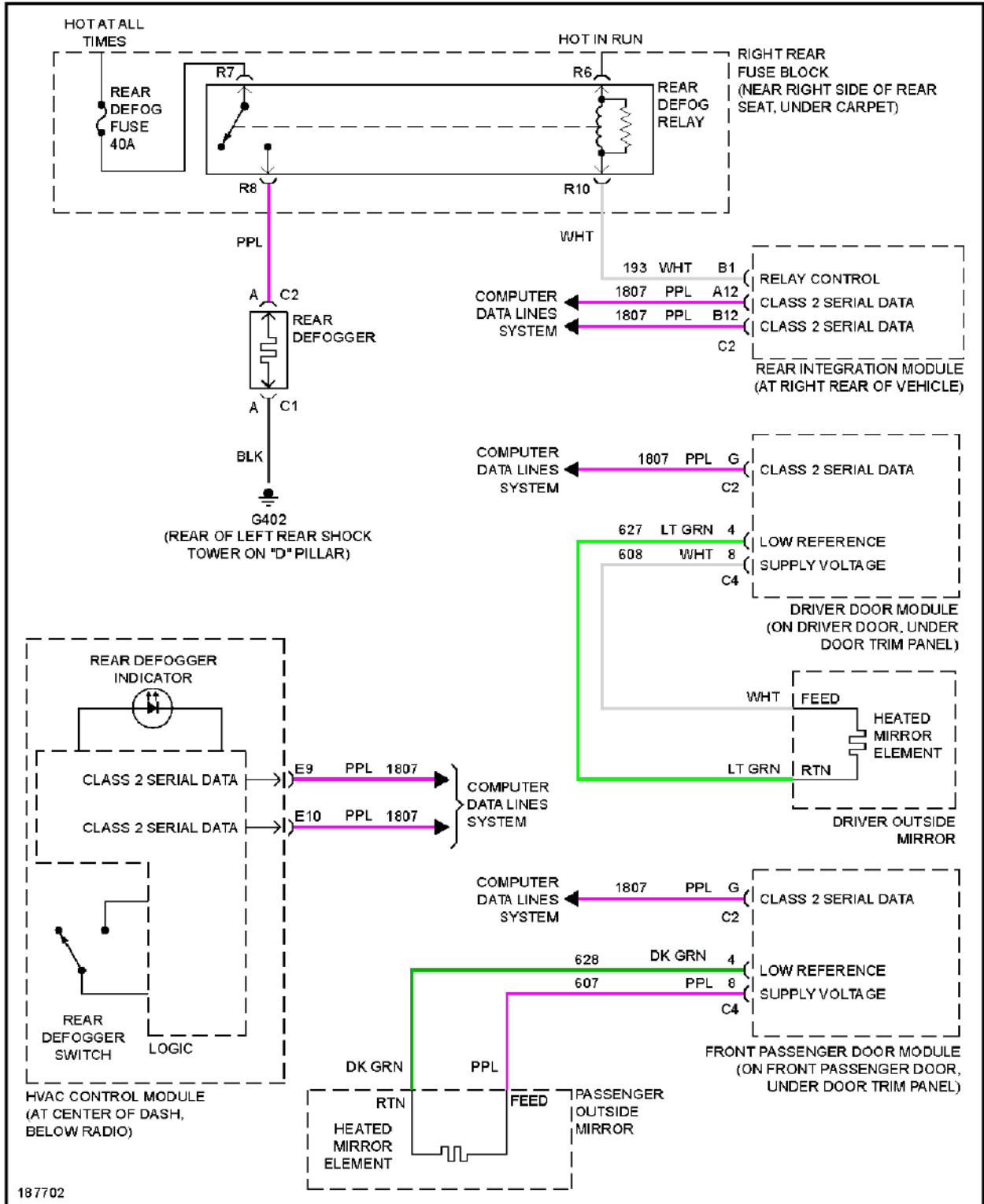
Fig. 16: Defoggers Circuit
