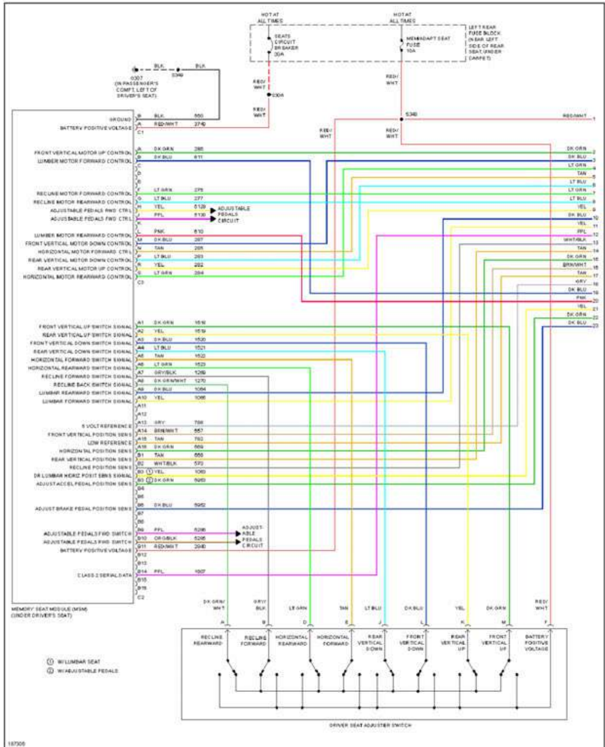
Fig. 45: Memory Seat Circuit (1 of 2)
