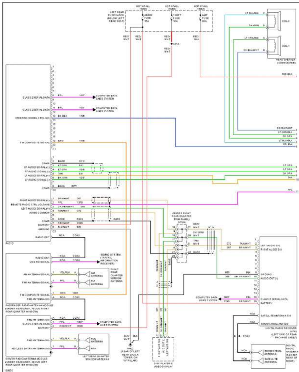
Fig. 69: Base Radio Circuit (1 of 2)
