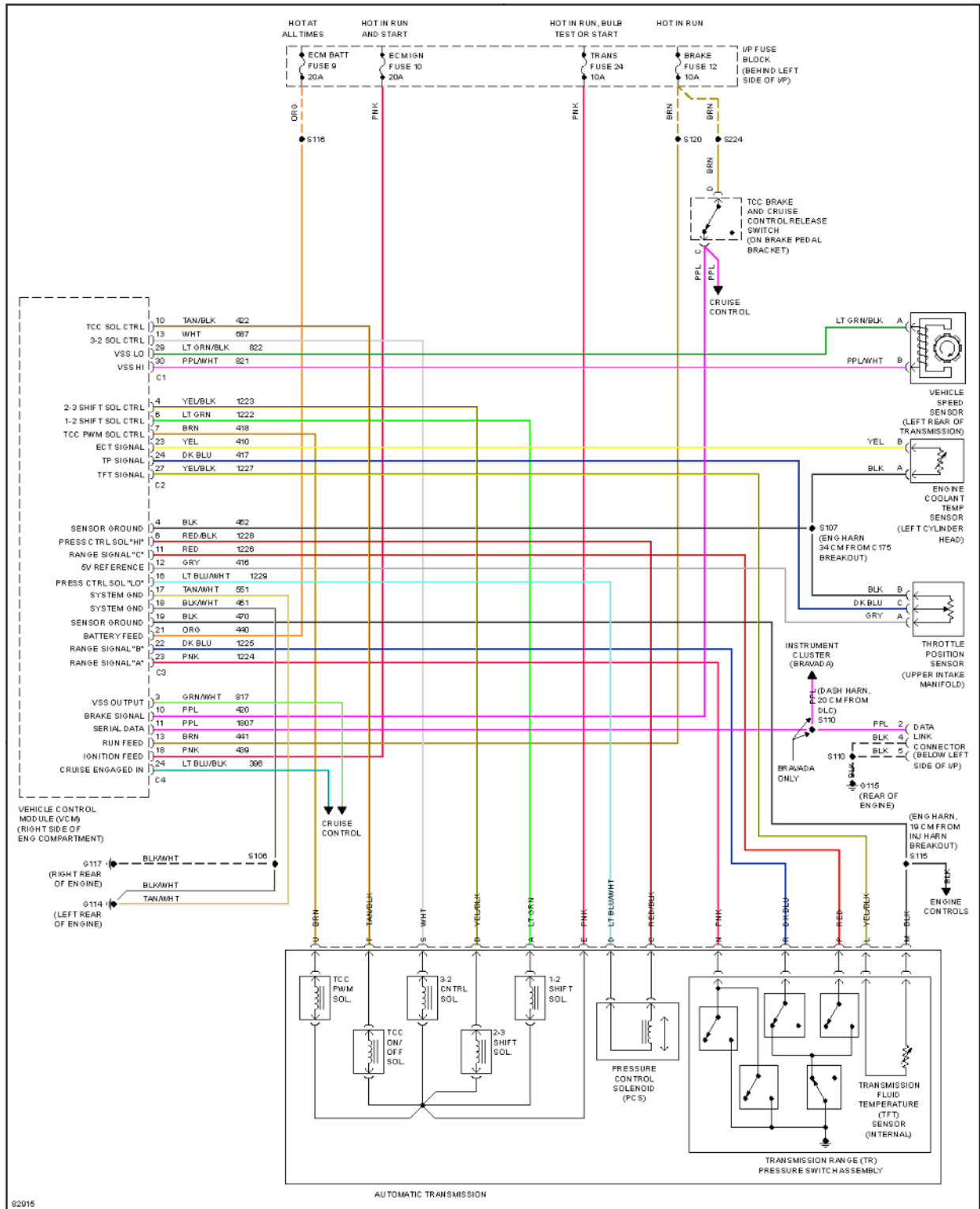
Fig. 37: 4.3L (VIN X), Transmission Circuit
