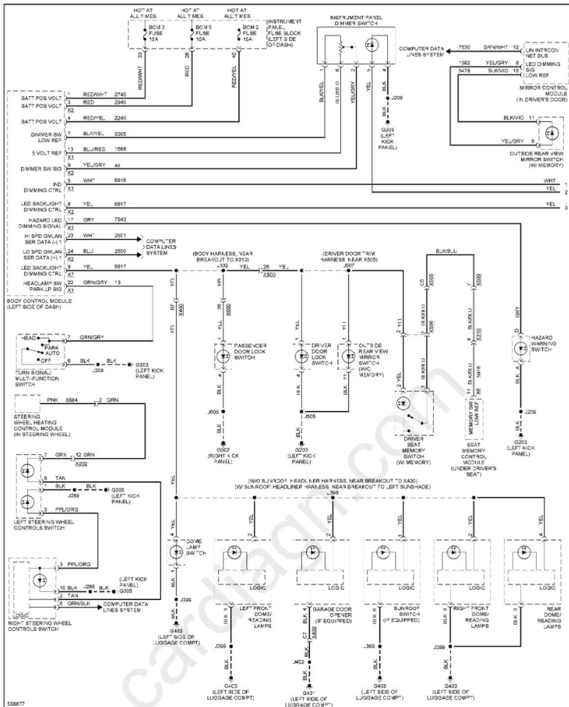
Fig. 68: Instrument Illumination Circuit (1 of 2)
