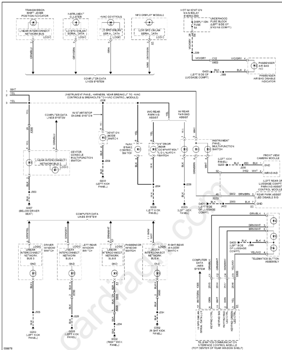
Fig. 69: Instrument Illumination Circuit (2 of 2)
