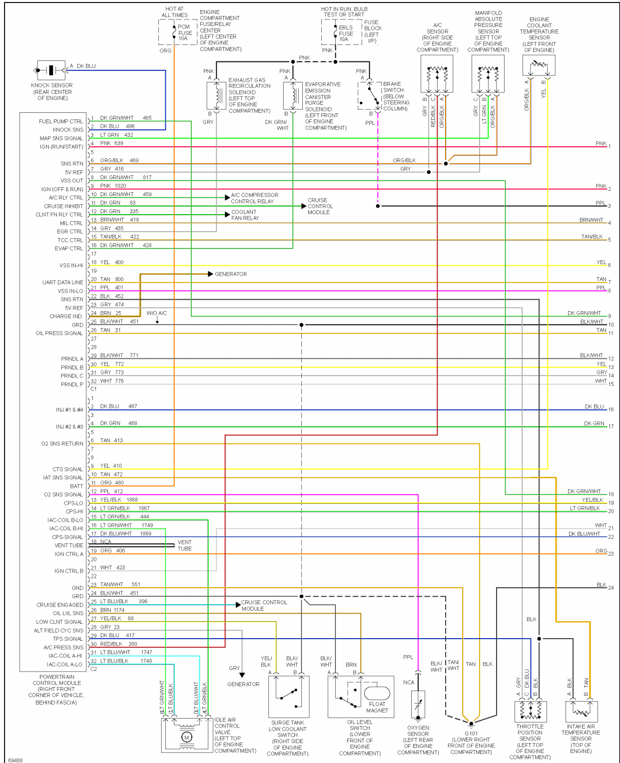
Fig. 10: 2.2L (VIN 4), Engine Performance Circuits (1 of 2)
