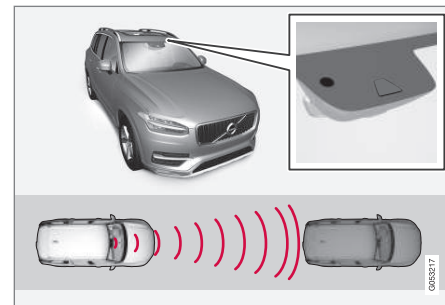
Location of the camera and the radar sensor
