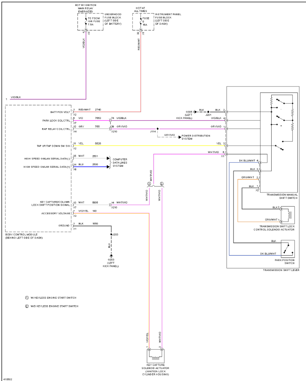
Fig. 131: 2.0L VIN X, Transmission Circuit (2 of 2)
