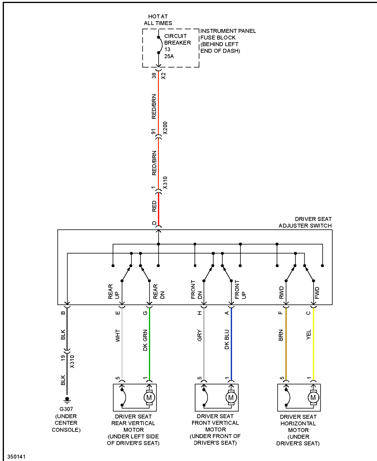
Fig. 55: Driver Power Seat Circuit
