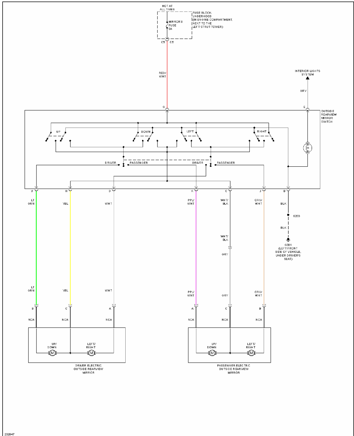
Fig. 45: Power Mirrors Circuit
