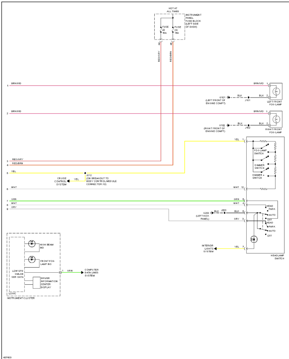
Fig. 64: Headlights Circuit, W/O High Intensity Discharge (2 of 2)
