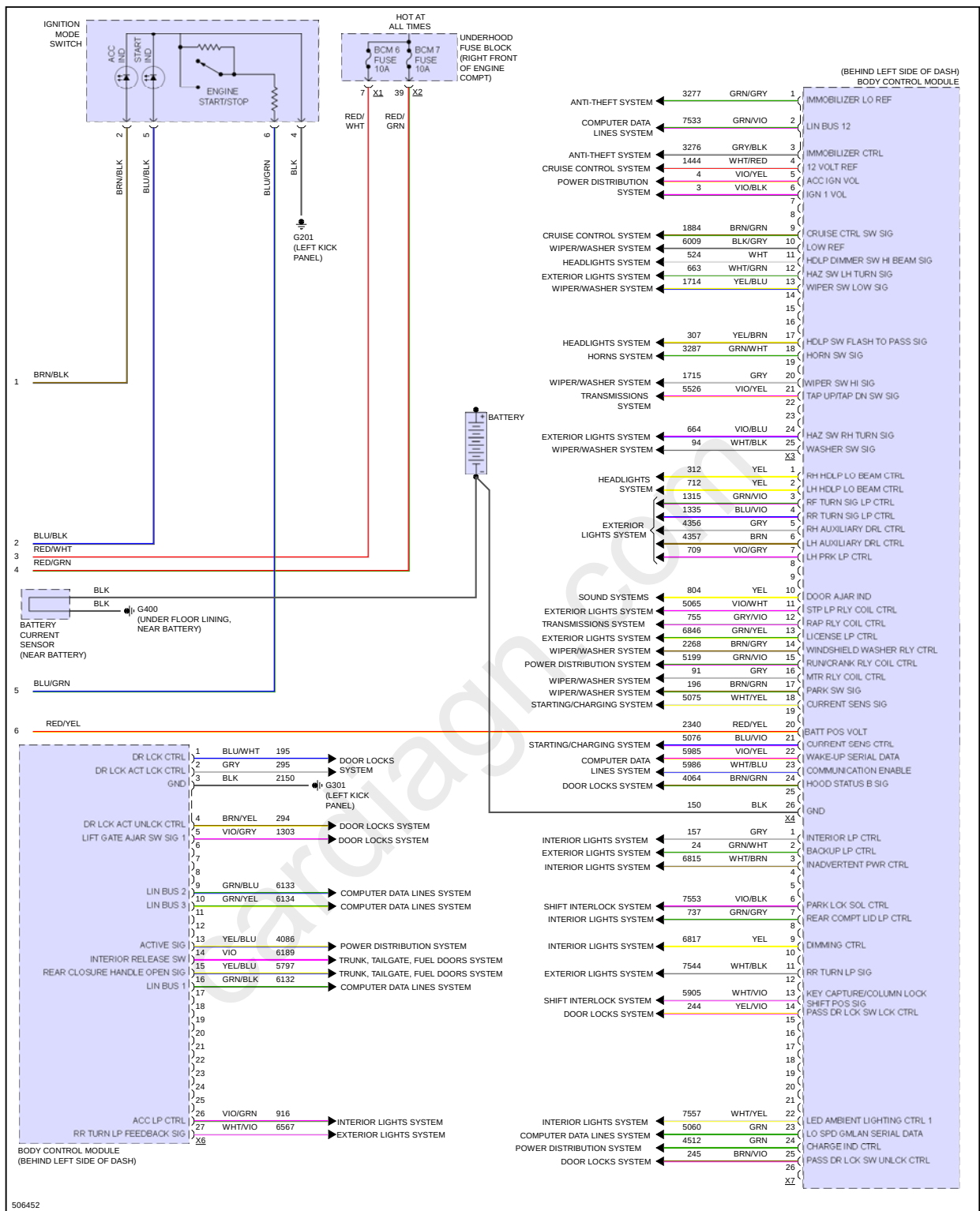
Fig 2: Body Control Modules Circuit (2 of 2)
