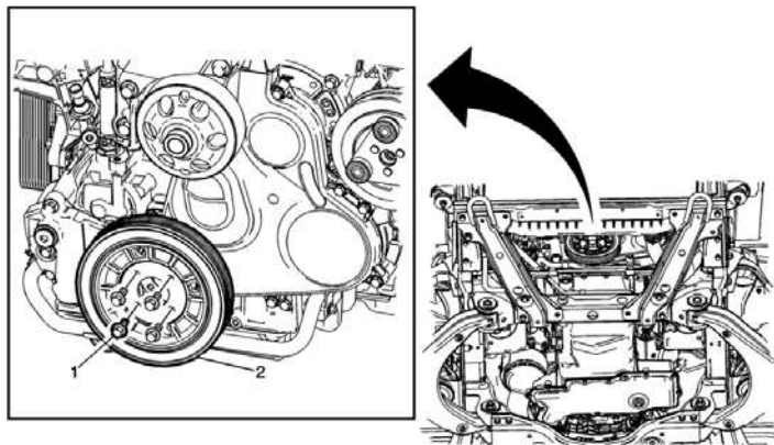
Crankshaft Pulley Replacement
