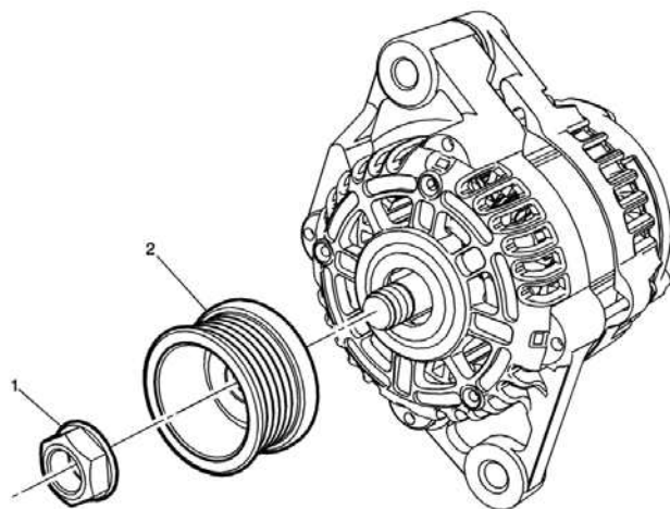
Generator Pulley Replacement
