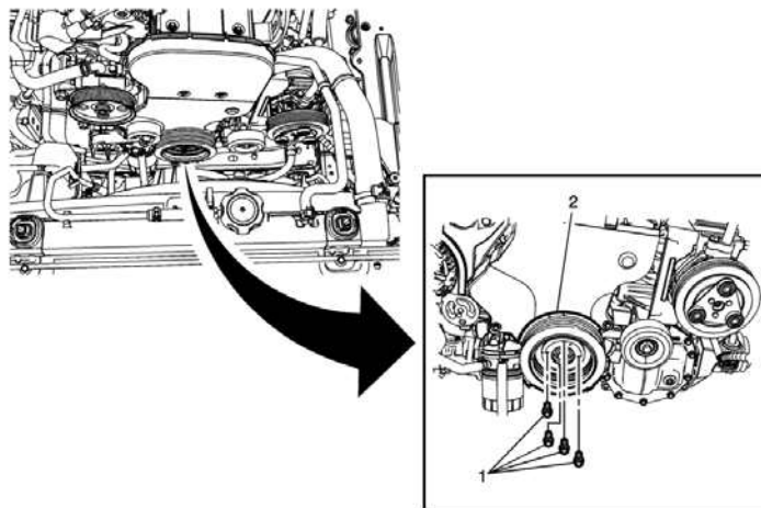
Crankshaft Pulley Replacement
