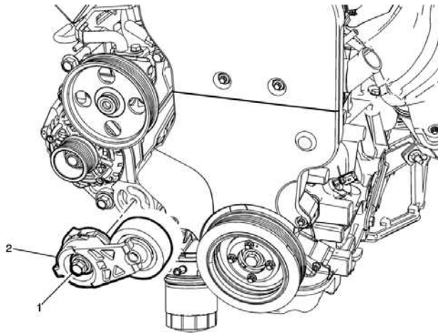
Drive Belt Tensioner Replacement
