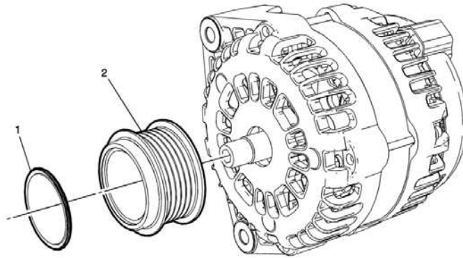
Generator Pulley Replacement
