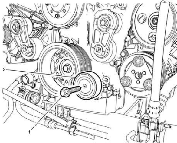
Drive Belt Idler Pulley Replacement
