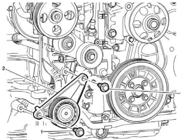
Belt Idler Pulley Replacement - Lower
