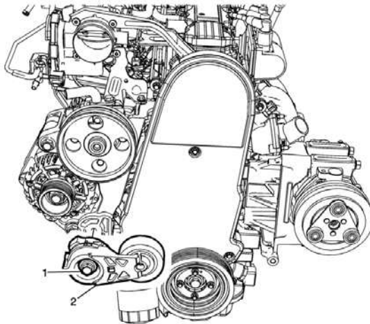
Drive Belt Tensioner Replacement
