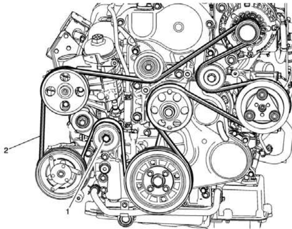
Drive Belt Replacement
