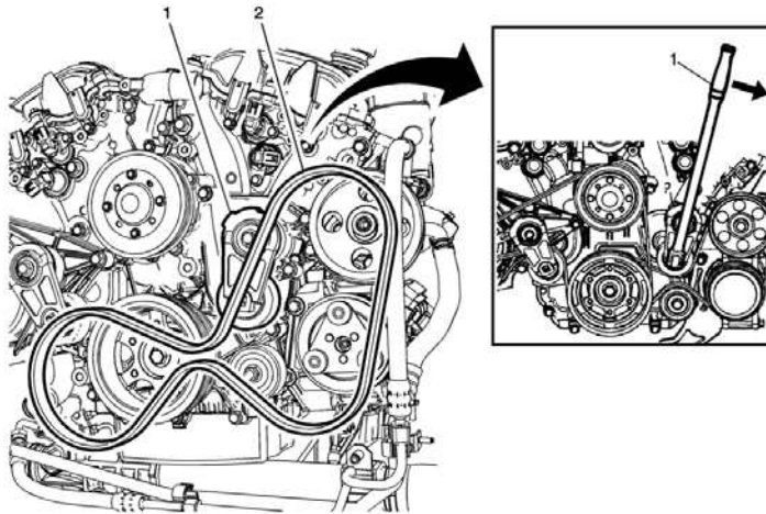
Air Conditioning Compressor and Power Steering Pump Belt Replacement
