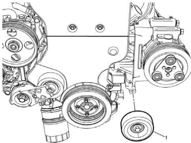
Belt Idler Pulley Replacement
