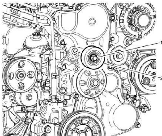
Drive Belt Idler Pulley Replacement - Right Side
