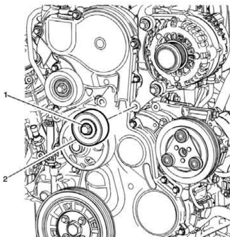
Drive Belt Idler Pulley Replacement - Left Side
