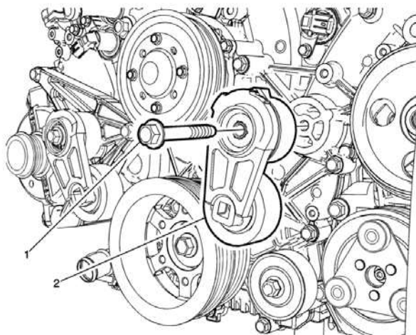
Air Conditioning Compressor and Power Steering Pump Belt Tensioner Replacement
