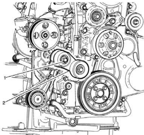
Drive Belt Tensioner Replacement
