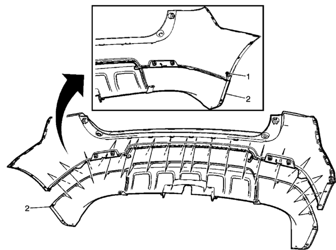
Fig. 22: Identifying Rear Bumper Lower Fascia Components (Equinox) Courtesy of GENERAL MOTORS CORP.
