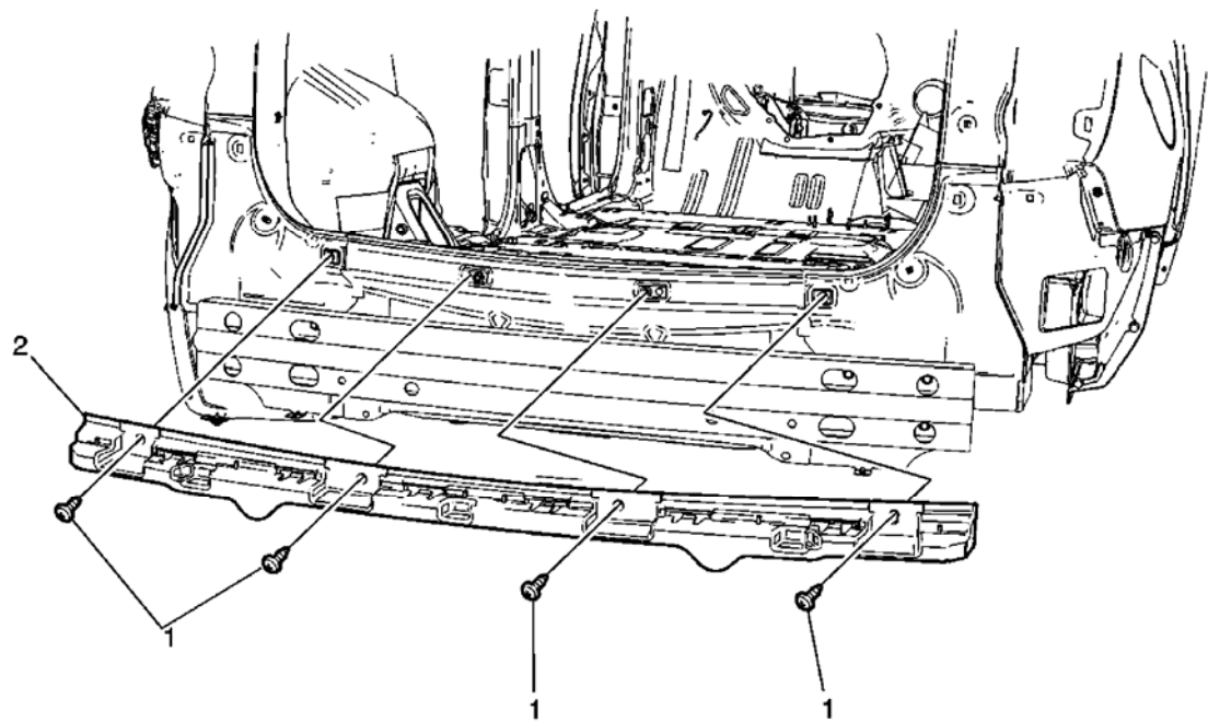
Fig. 24: Identifying Rear Bumper Fascia Support Components Courtesy of GENERAL MOTORS CORP.
