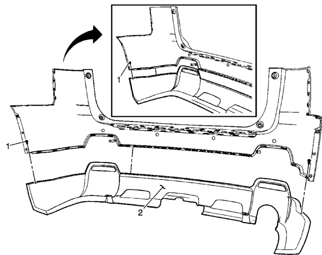
Fig. 23: Identifying Rear Bumper Lower Fascia Components (Terrain) Courtesy of GENERAL MOTORS CORP.
