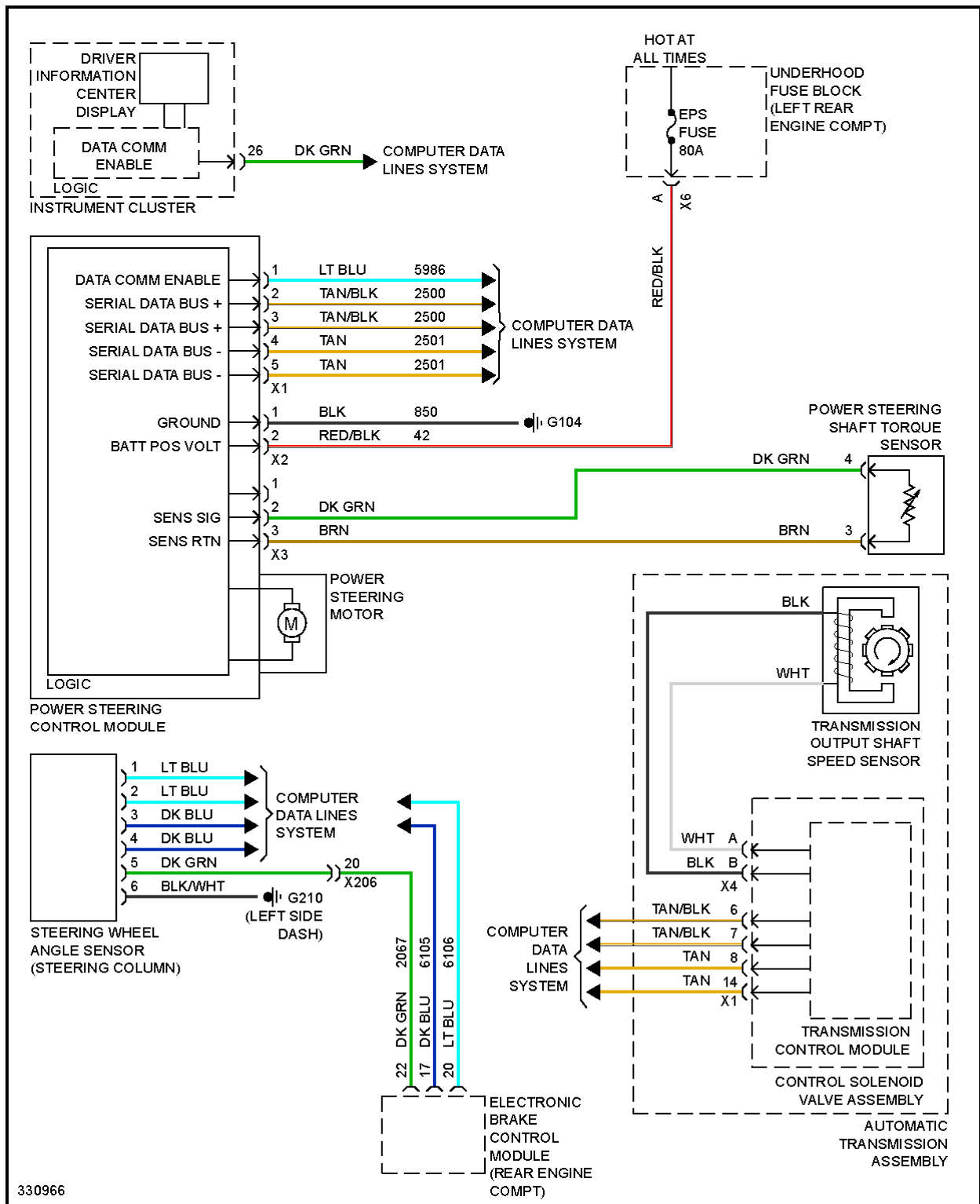
Fig. 18: Electronic Power Steering Circuit
