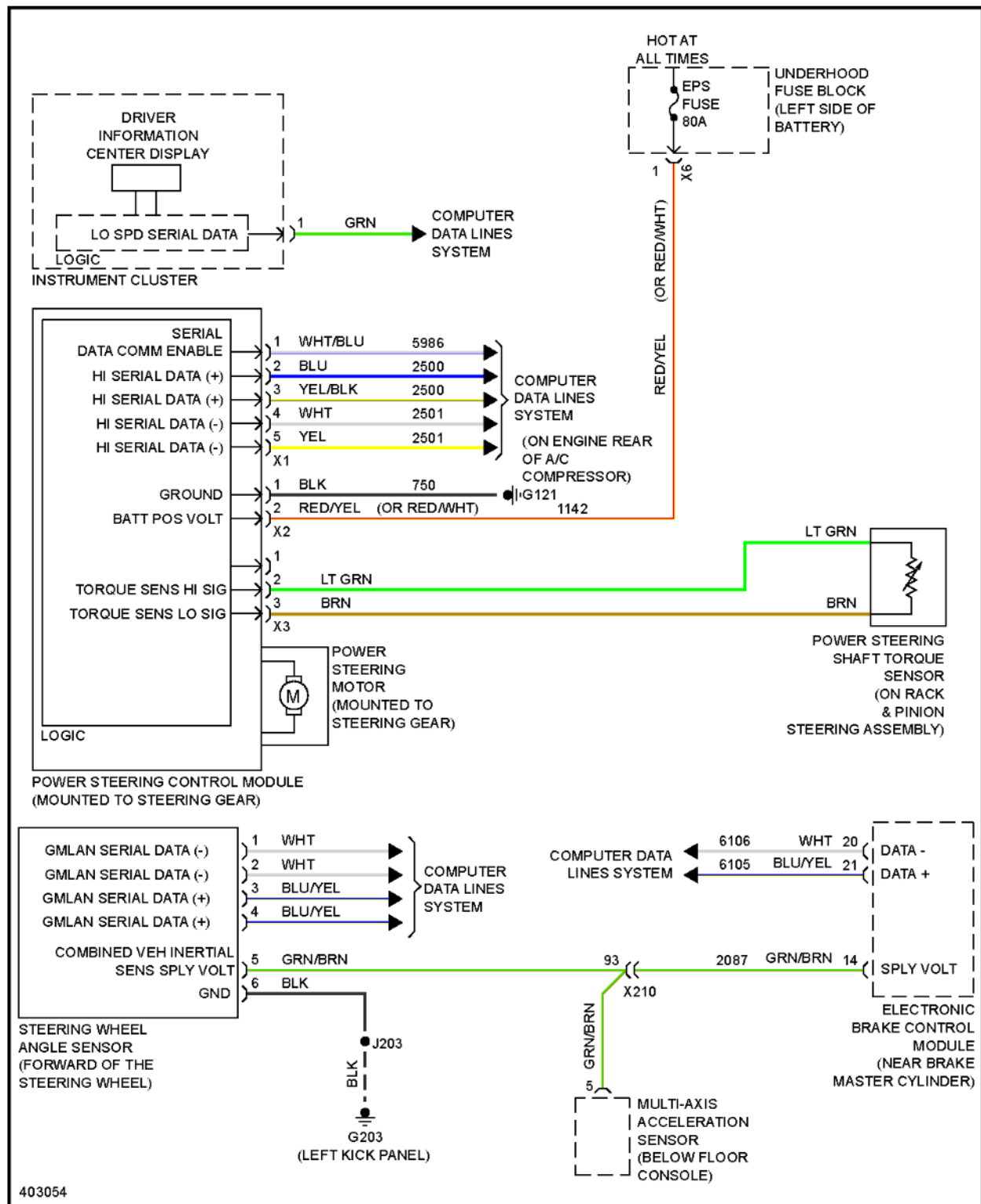
Fig. 28: Electronic Power Steering Circuit
