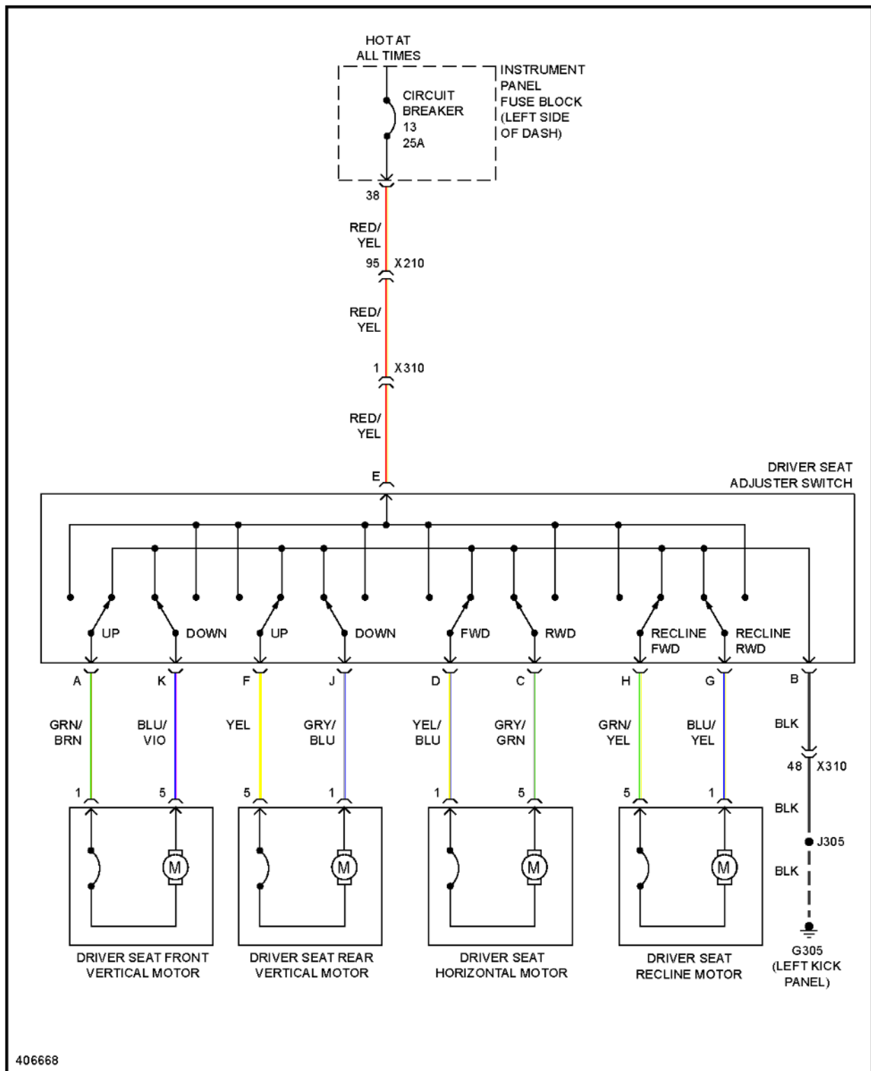
Fig. 103: Driver Power Seat Circuit, 8-Way Power Seat
