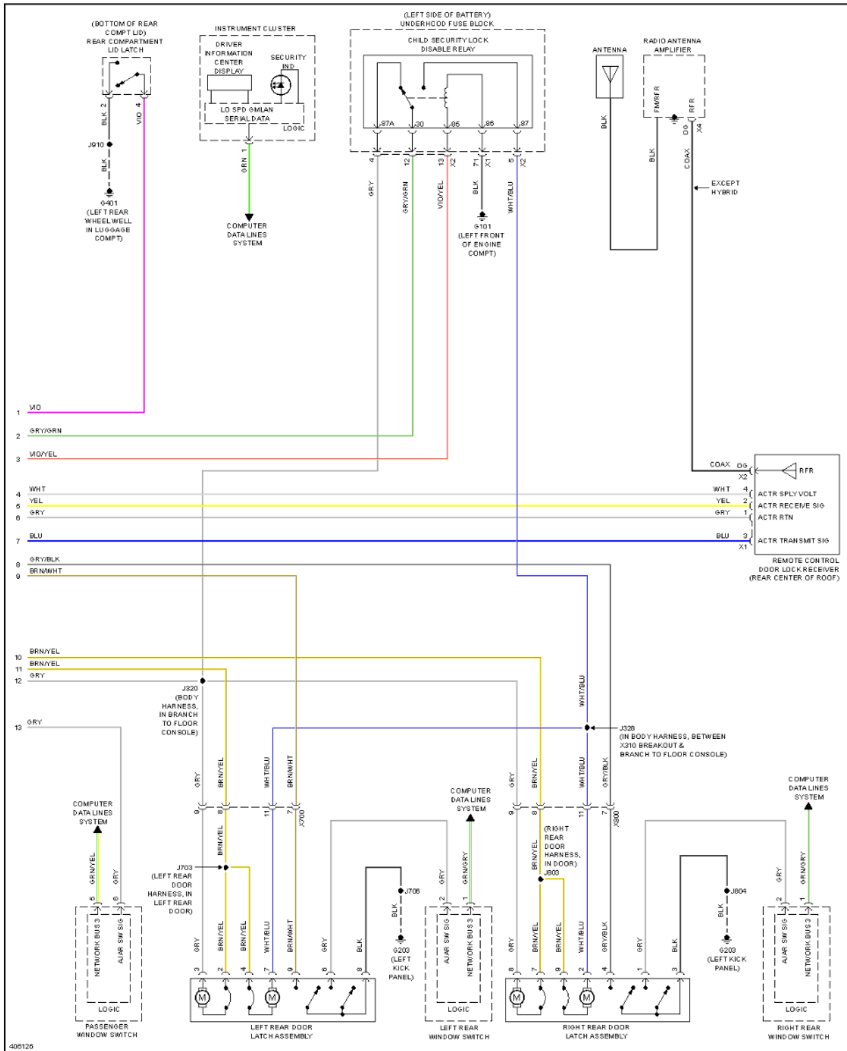
Fig. 99: Power Door Locks Circuit, W/O Passive Keyless Entry (2 of 2)
