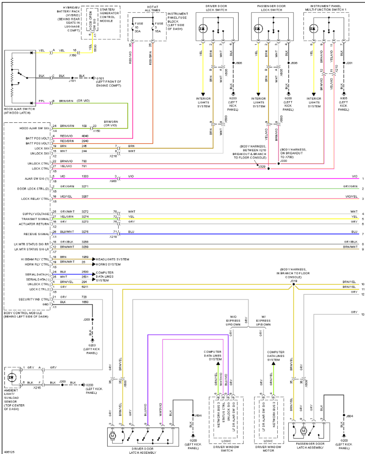
Fig. 98: Power Door Locks Circuit, W/O Passive Keyless Entry (1 of 2)
