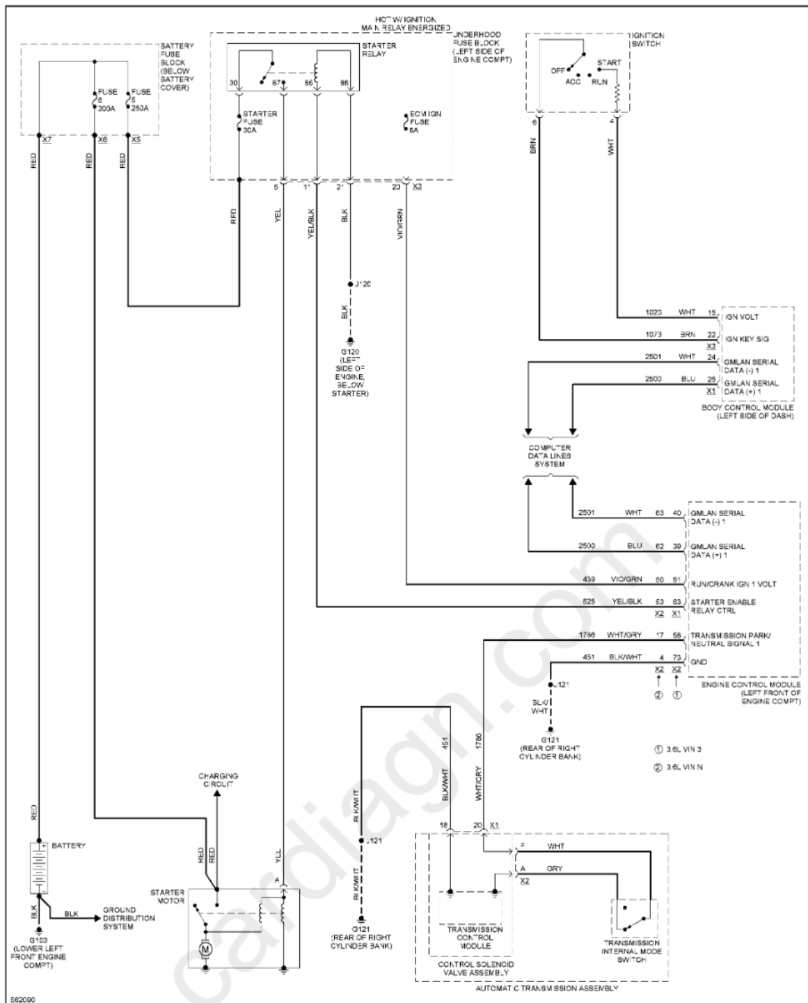
Fig. 121: Starting Circuit, W/O Start-Stop System
