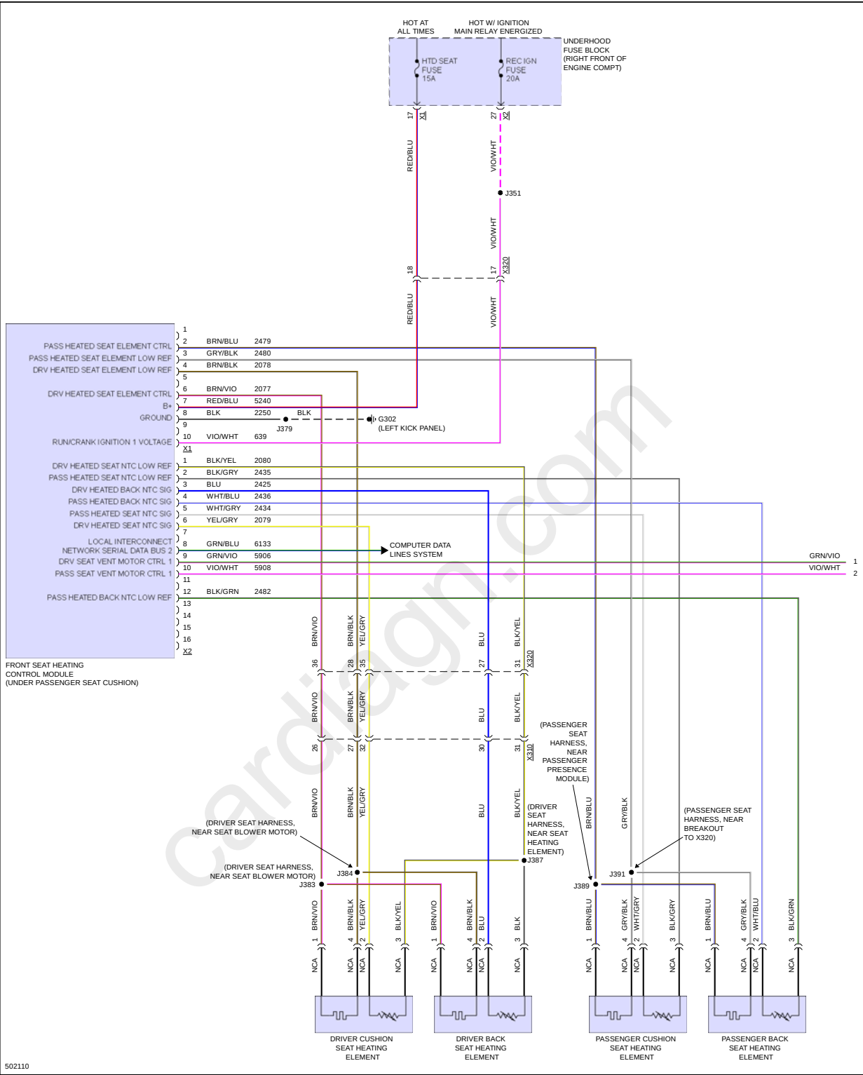
Fig 2: Front Heated Seats Circuit (1 of 2)
