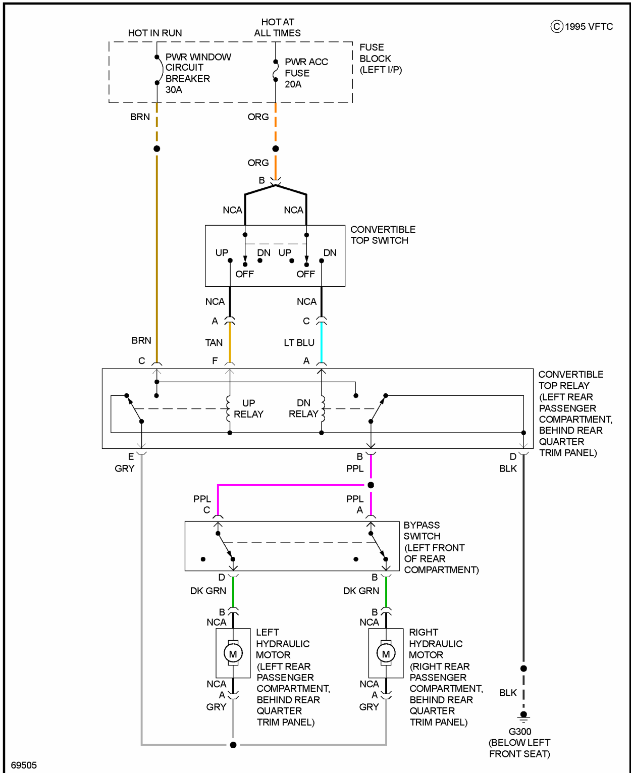
Fig. 34: Convertible Top Circuit
