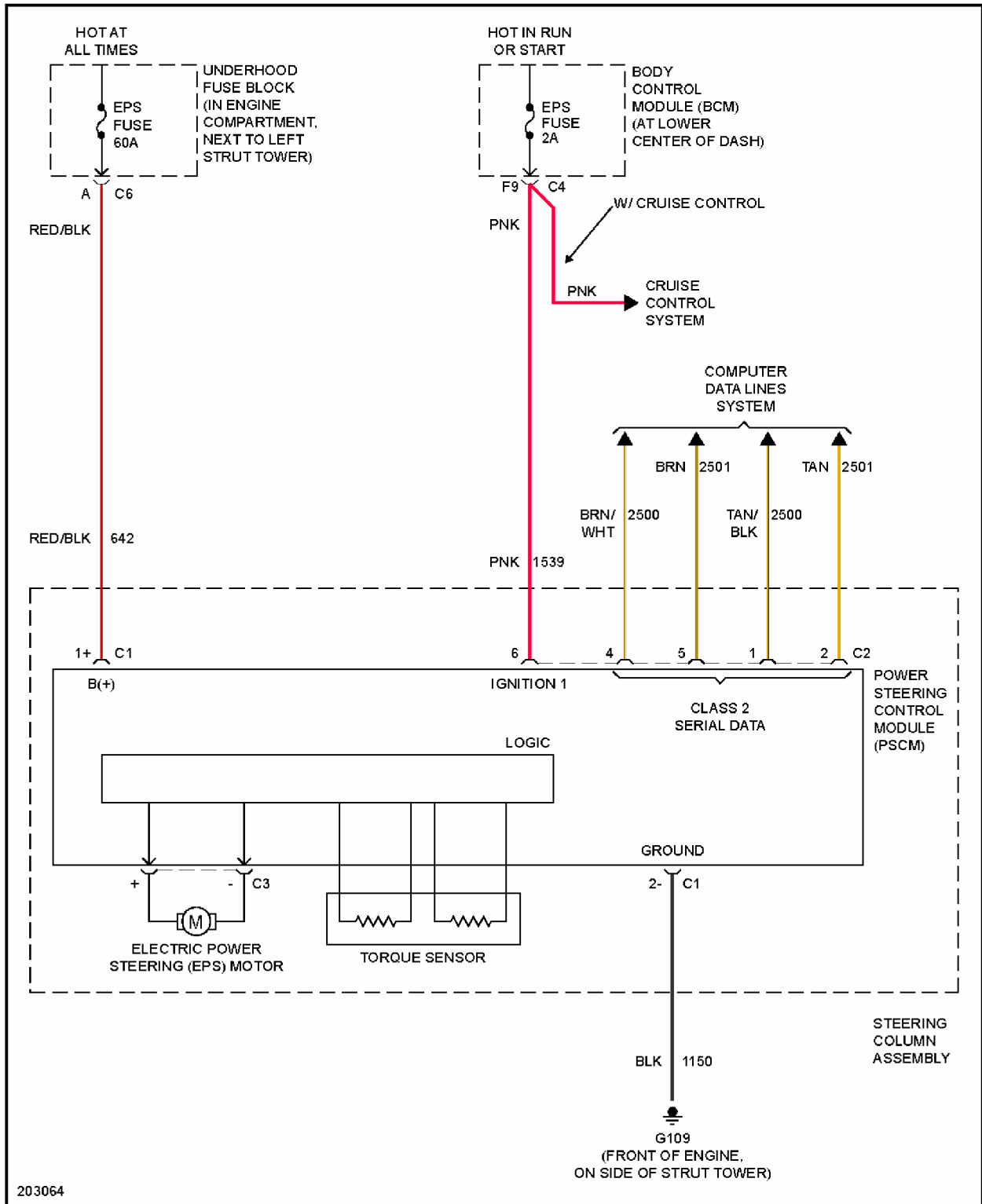
Fig. 20: Electronic Power Steering Circuit
