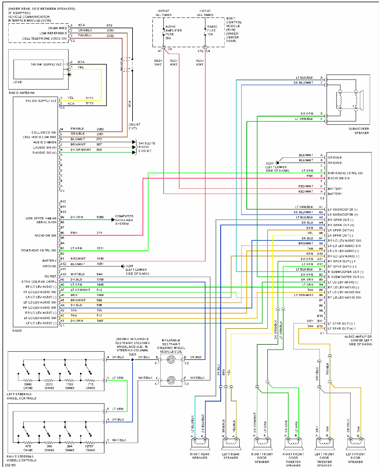
Fig. 50: Radio Circuit, W/ Amplifier
