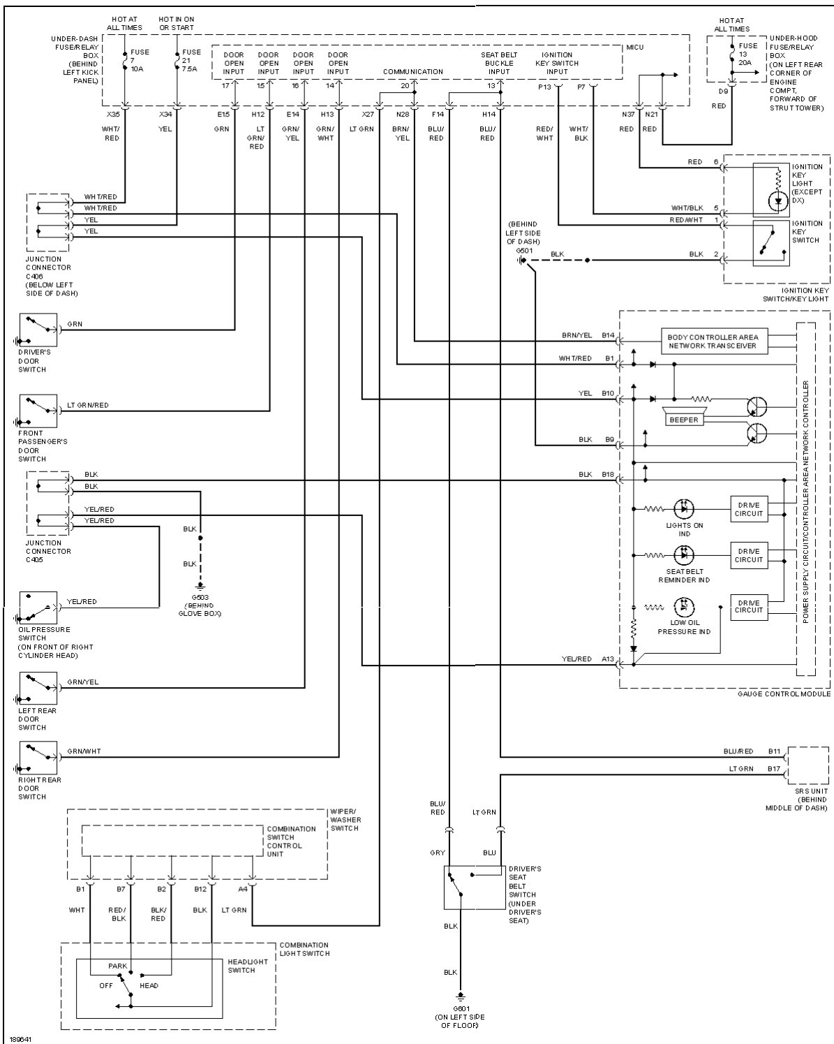
Fig. 72: Warning Systems Circuit
