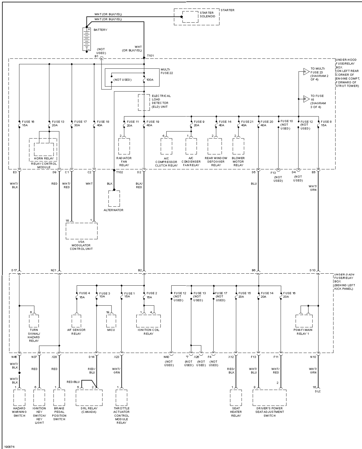
Fig. 39: Power Distribution Circuit (1 of 4)
