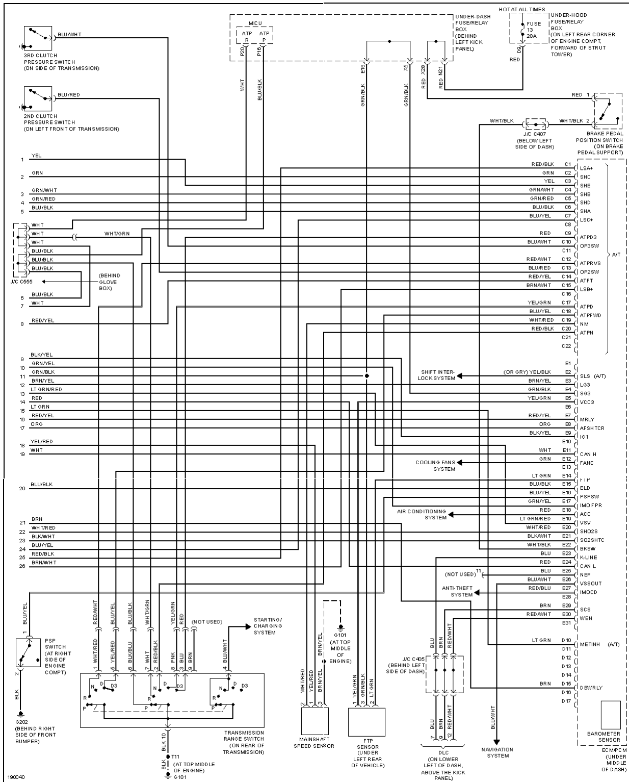
Fig. 19: 2.4L, Engine Performance Circuit (4 of 4)
