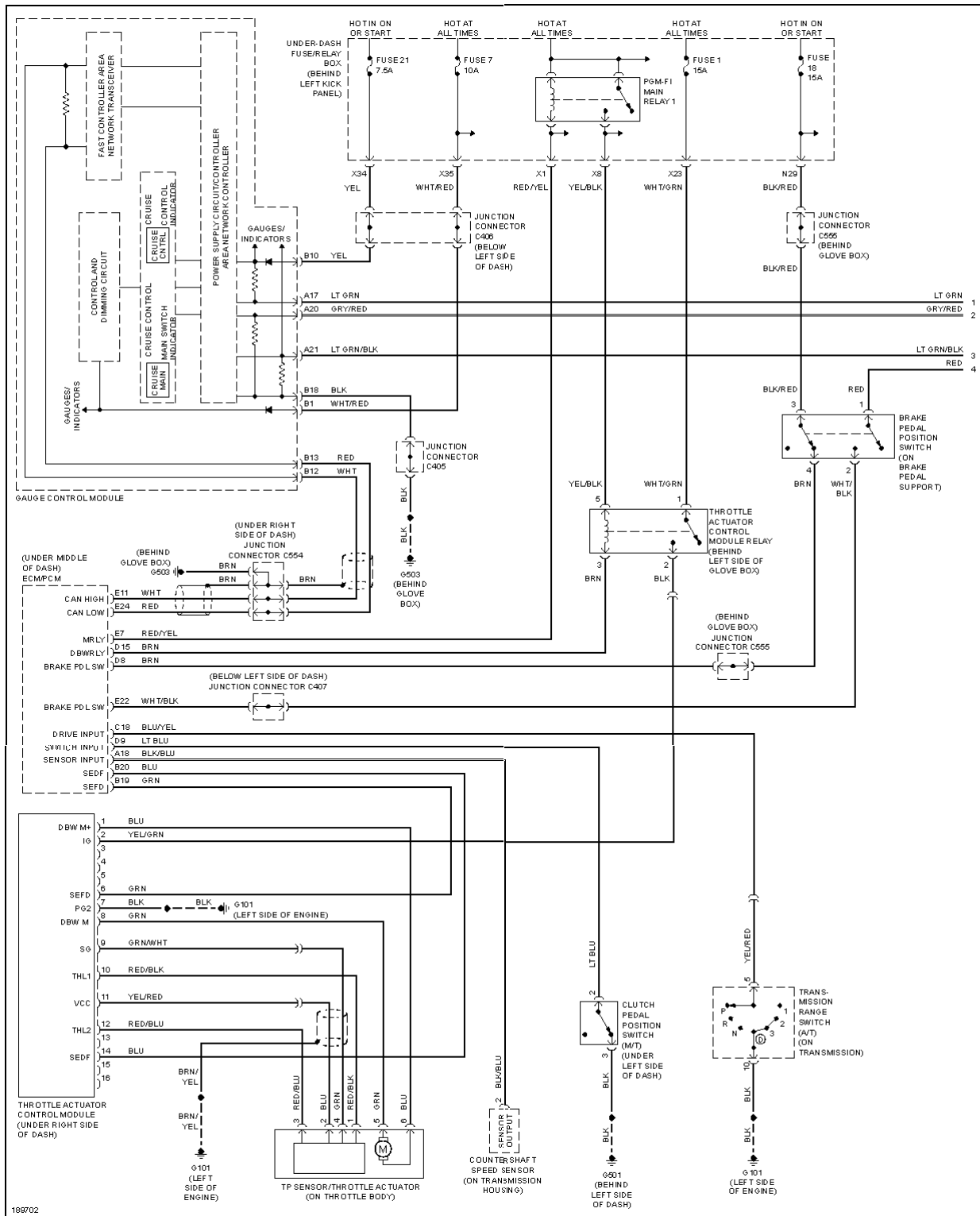
Fig. 12: Cruise Control Circuit (1 of 2)
