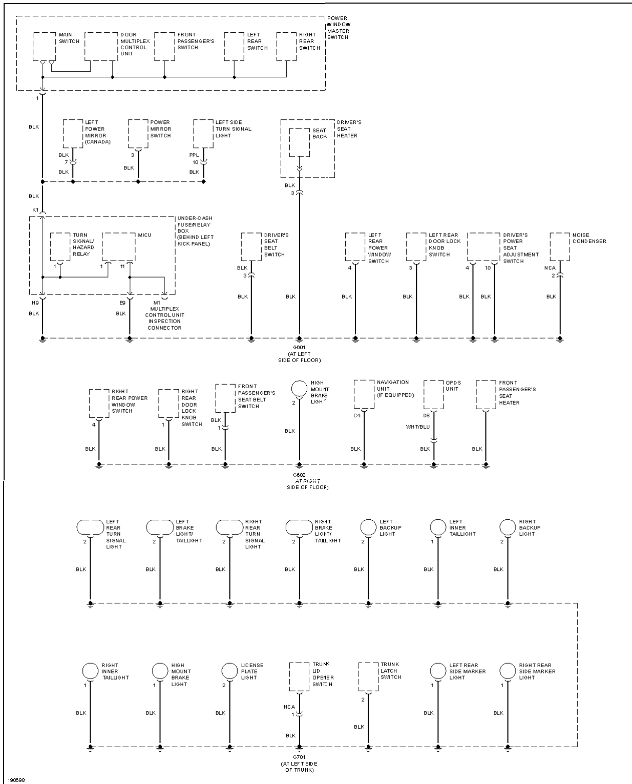
Fig. 27: Ground Distribution Circuit (4 of 4)
