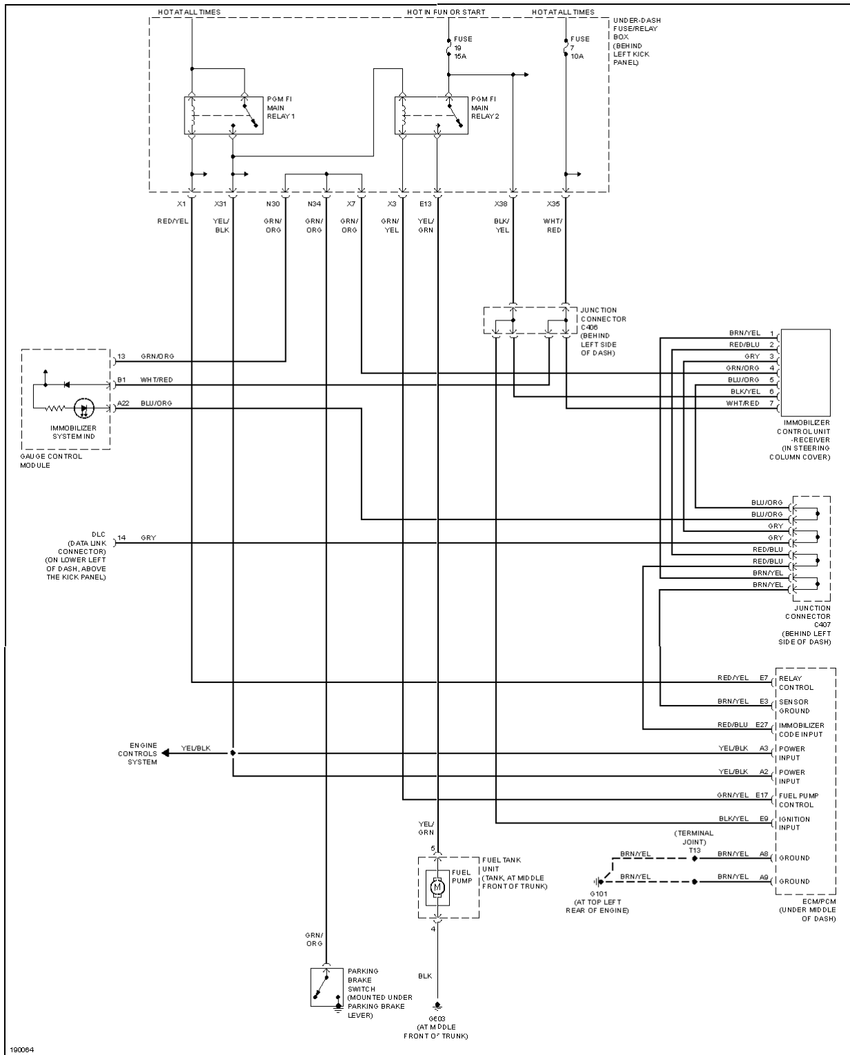
Fig. 8: Immobilizer Circuit
