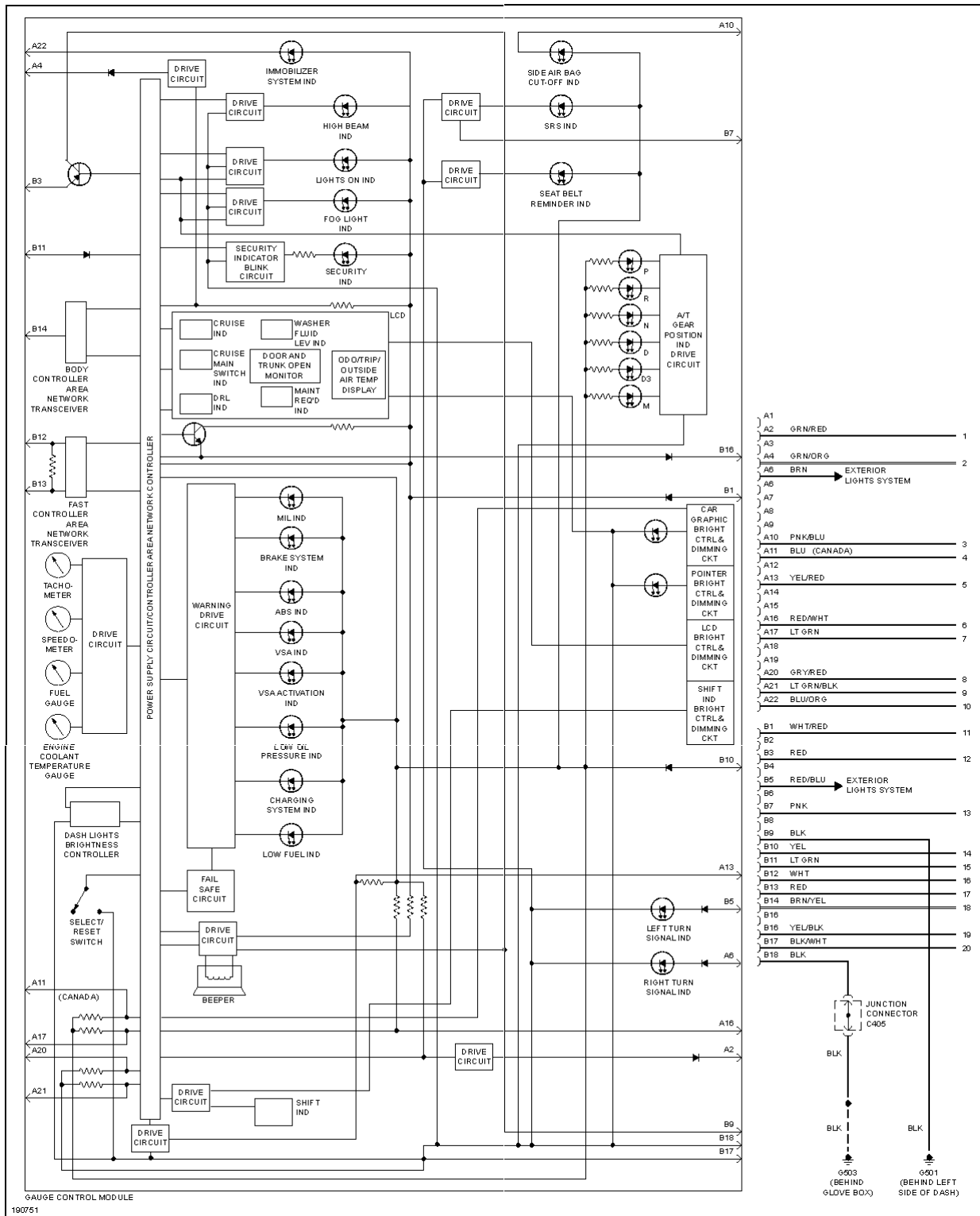
Fig. 32: Instrument Cluster Circuit (1 of 2)
