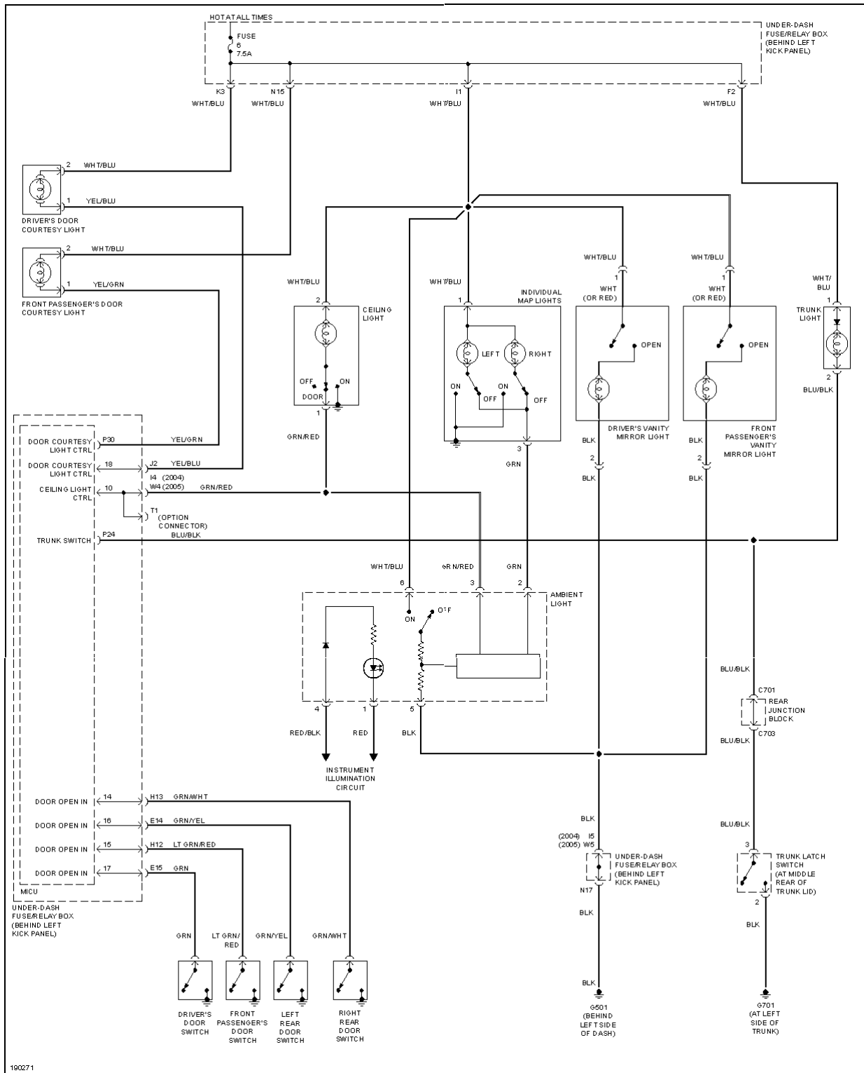
Fig. 34: Courtesy Lamps Circuit
