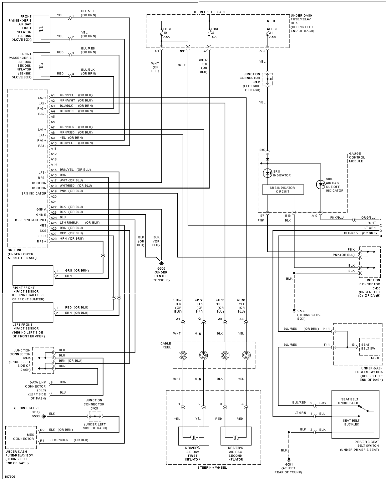
Fig. 67: Supplemental Restraints Circuit (1 of 2)
