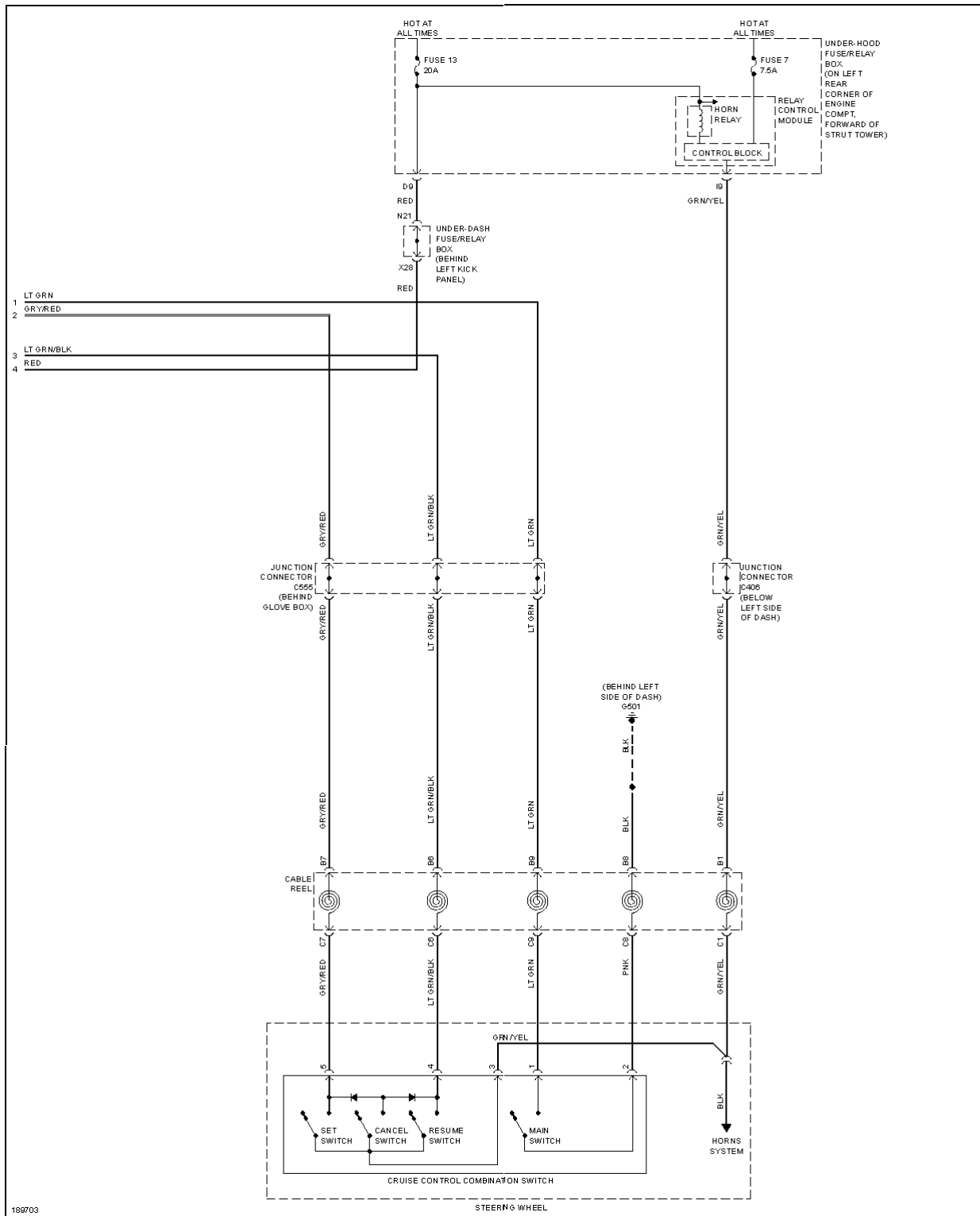
Fig. 13: Cruise Control Circuit (2 of 2)
