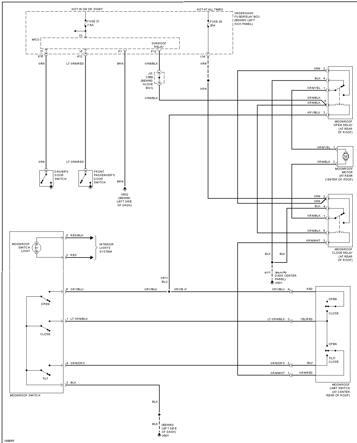
Fig. 48: Power Top/Sunroof Circuit
