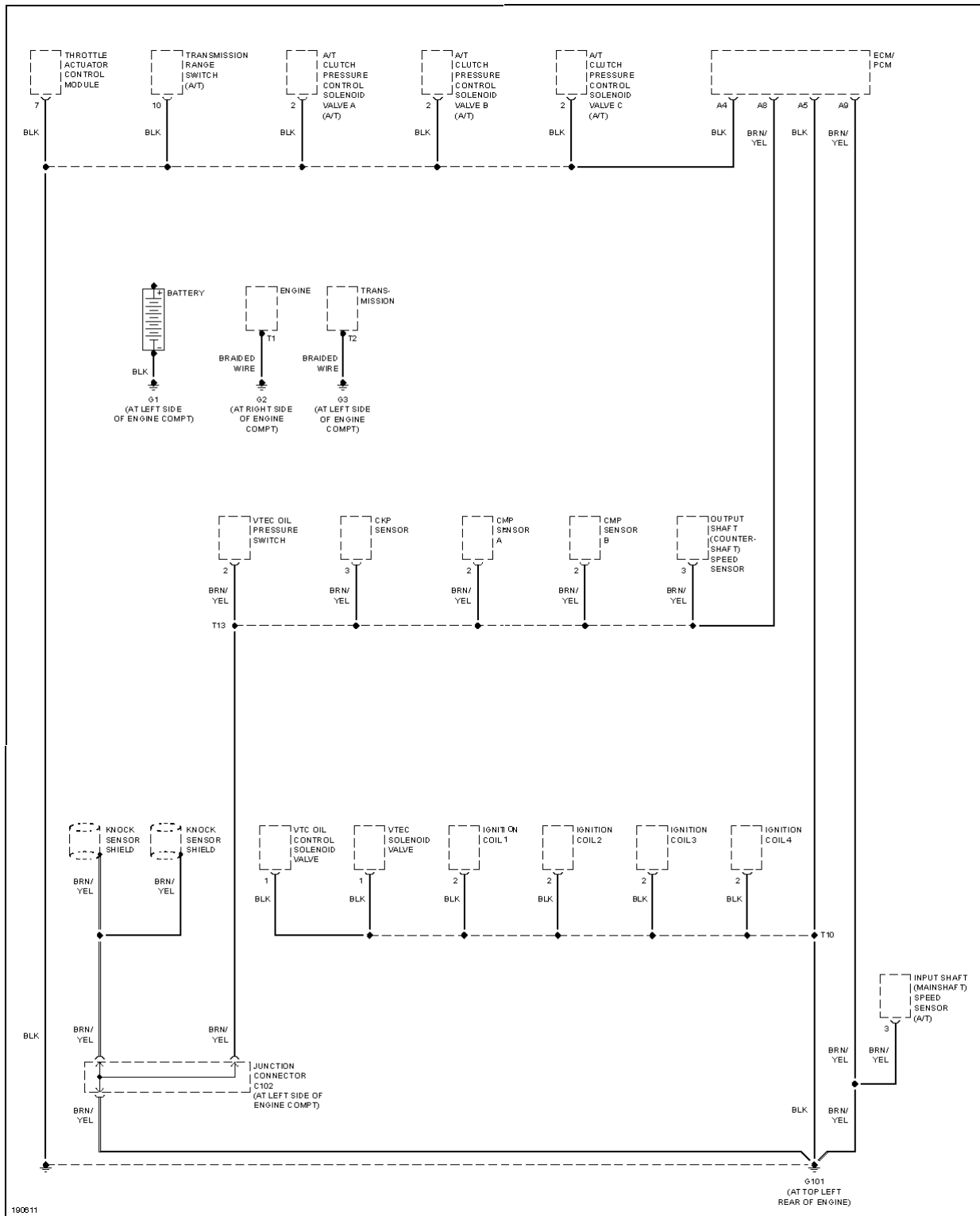
Fig. 24: Ground Distribution Circuit (1 of 4)
