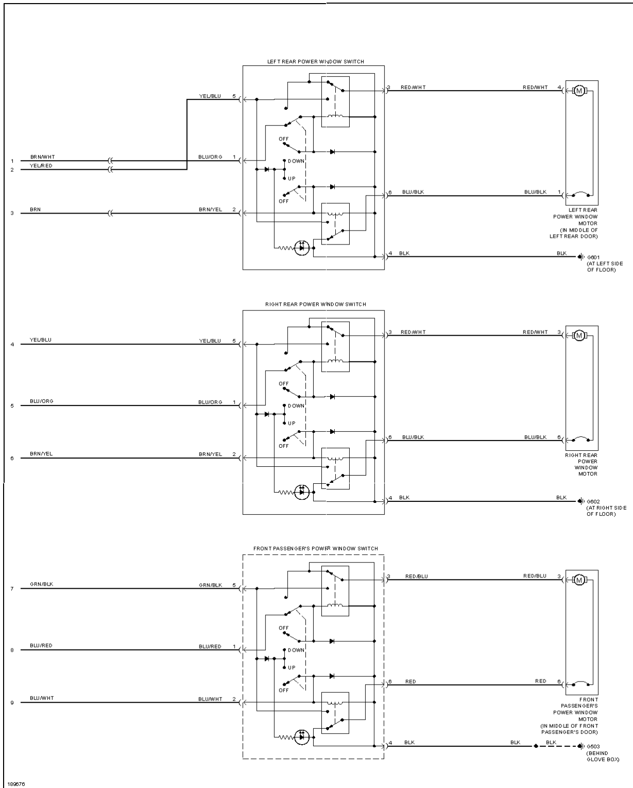
Fig. 50: Power Windows Circuit (2 of 2)
