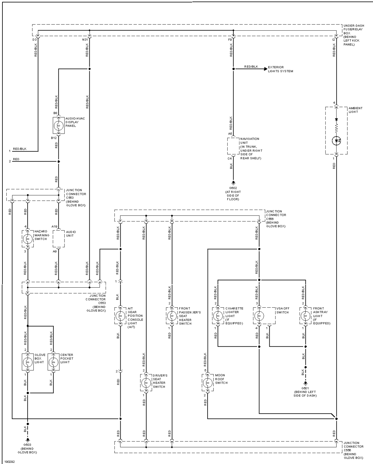
Fig. 37: Instrument Illumination Circuit (2 of 2)
