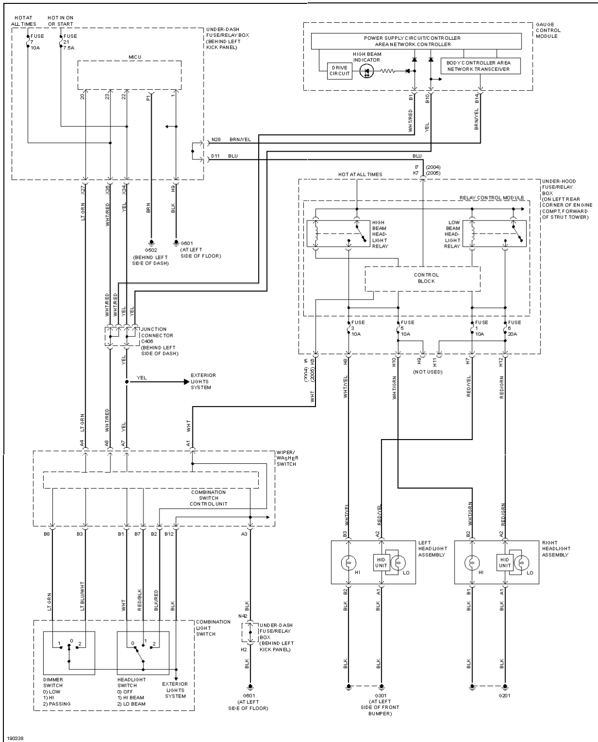
Fig. 30: Headlamps Circuit, W/O DRL
