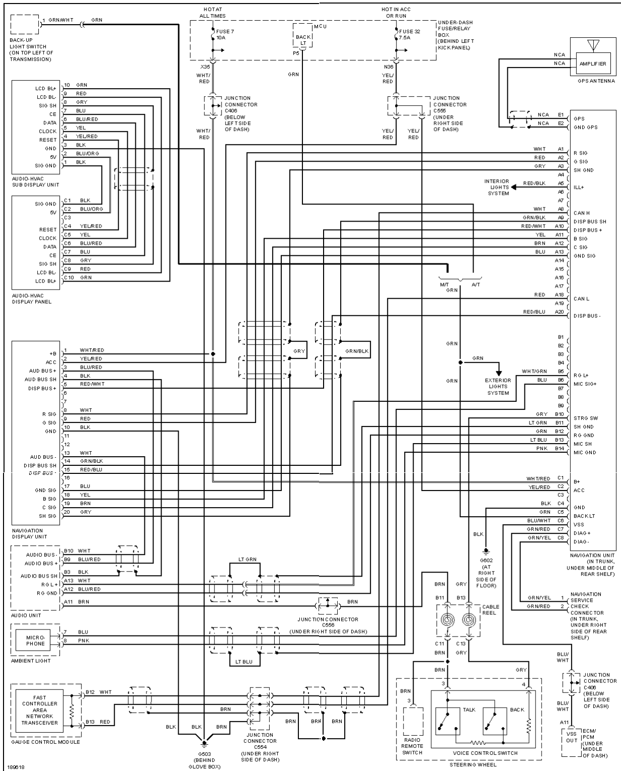
Fig. 38: Navigation Circuit
