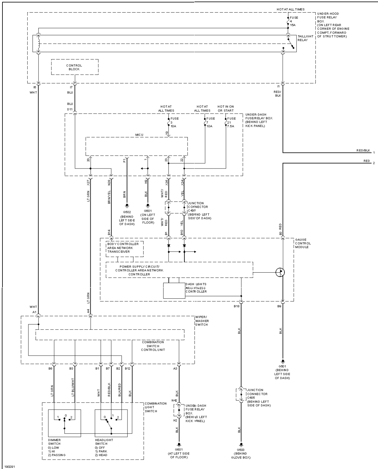
Fig. 36: Instrument Illumination Circuit (1 of 2)
