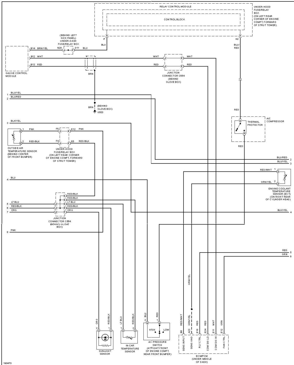
Fig. 2: Air Conditioning Circuit (2 of 3)
