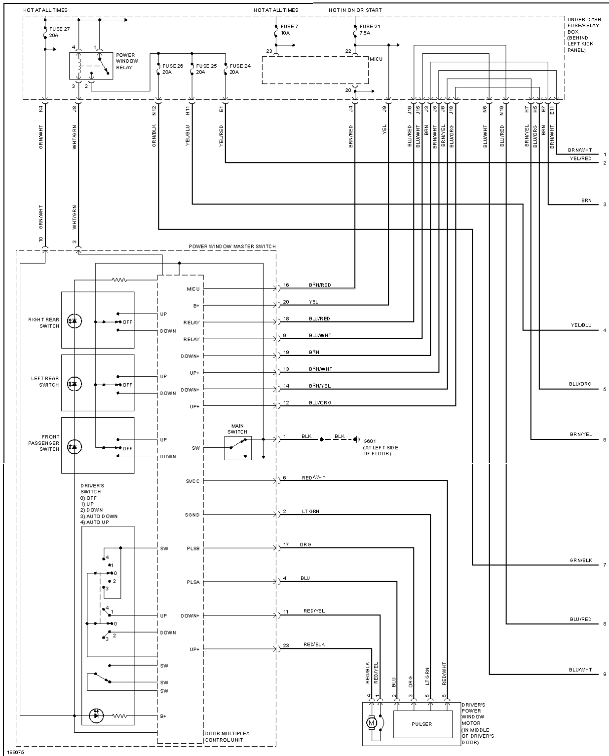
Fig. 49: Power Windows Circuit (1 of 2)
