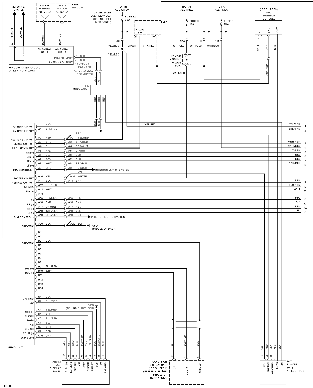
Fig. 54: DVD Player Circuit, W/O Cassette or MP3 Player (1 of 3)
