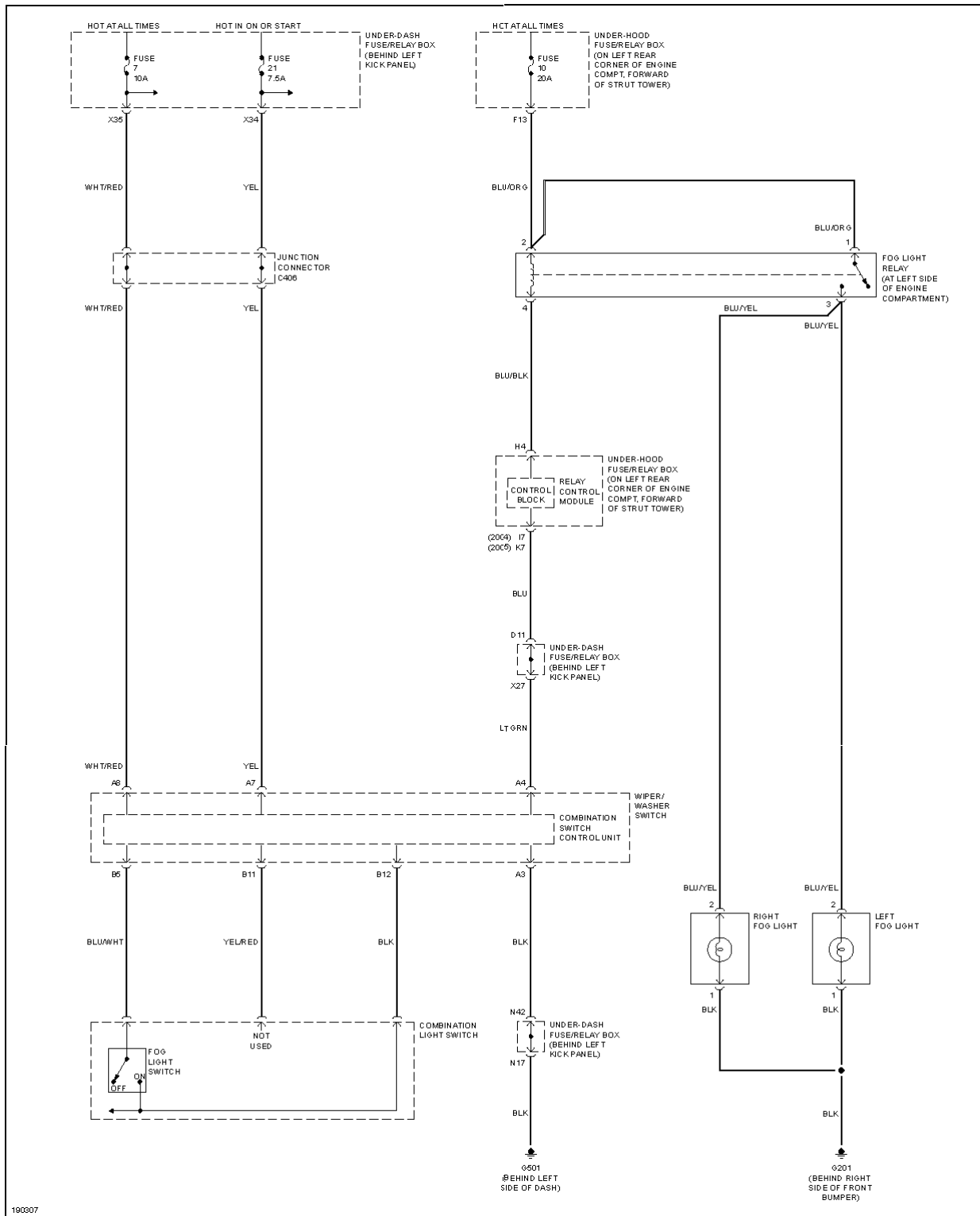
Fig. 28: Fog Lamp Circuit, Accessory
