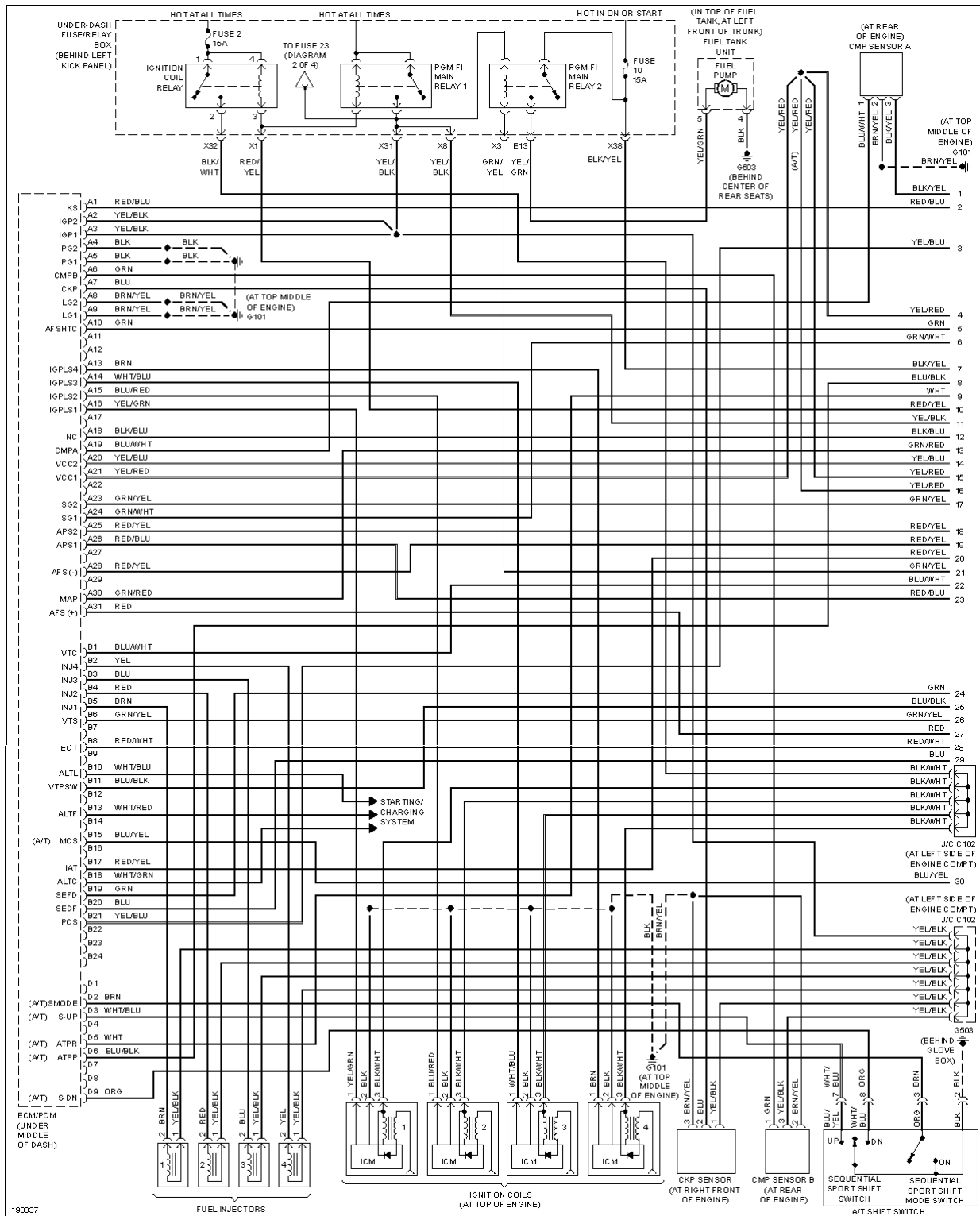
Fig. 16: 2.4L, Engine Performance Circuit (1 of 4)
