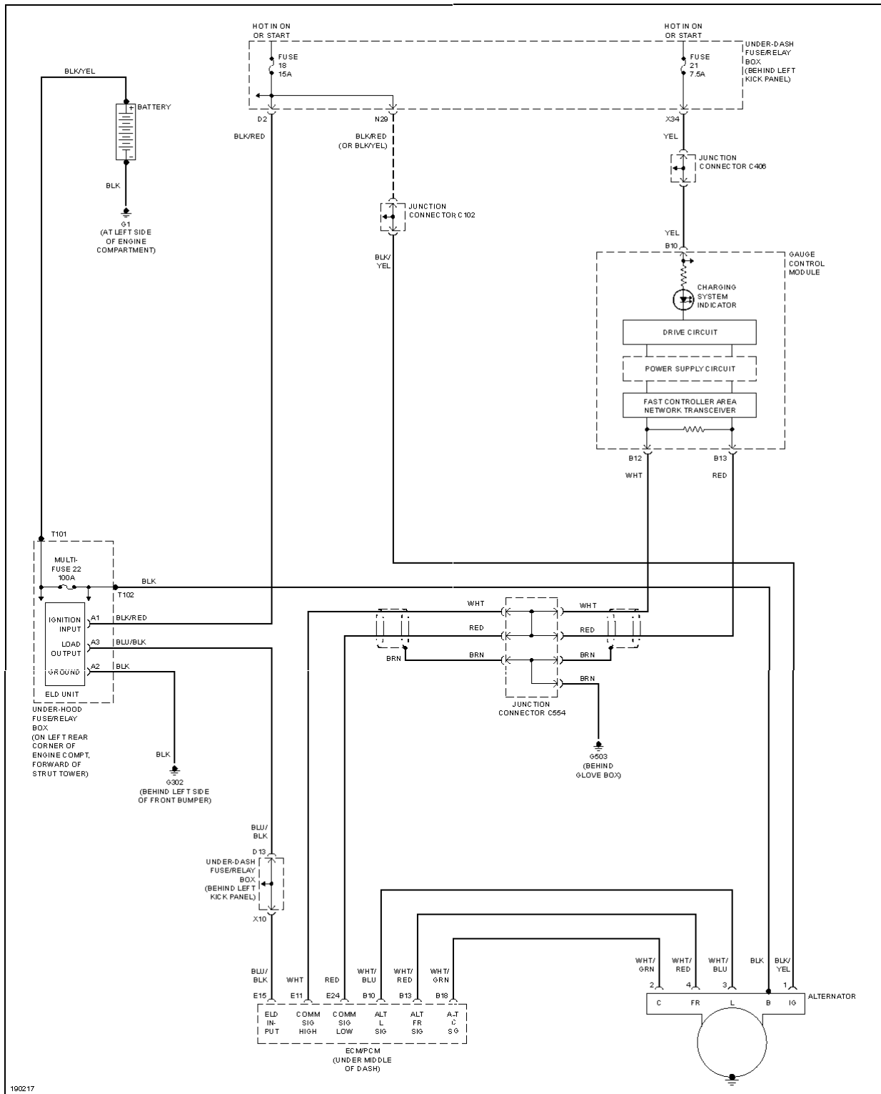
Fig. 65: Charging Circuit
