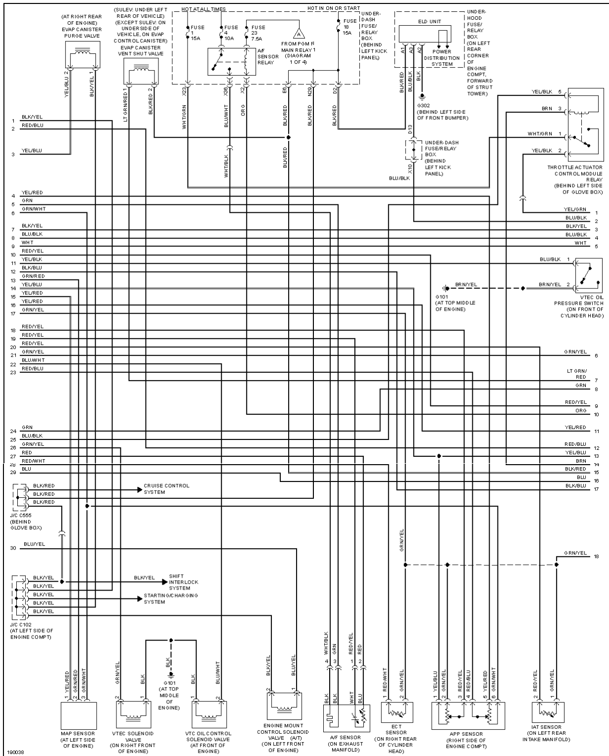
Fig. 17: 2.4L, Engine Performance Circuit (2 of 4)
