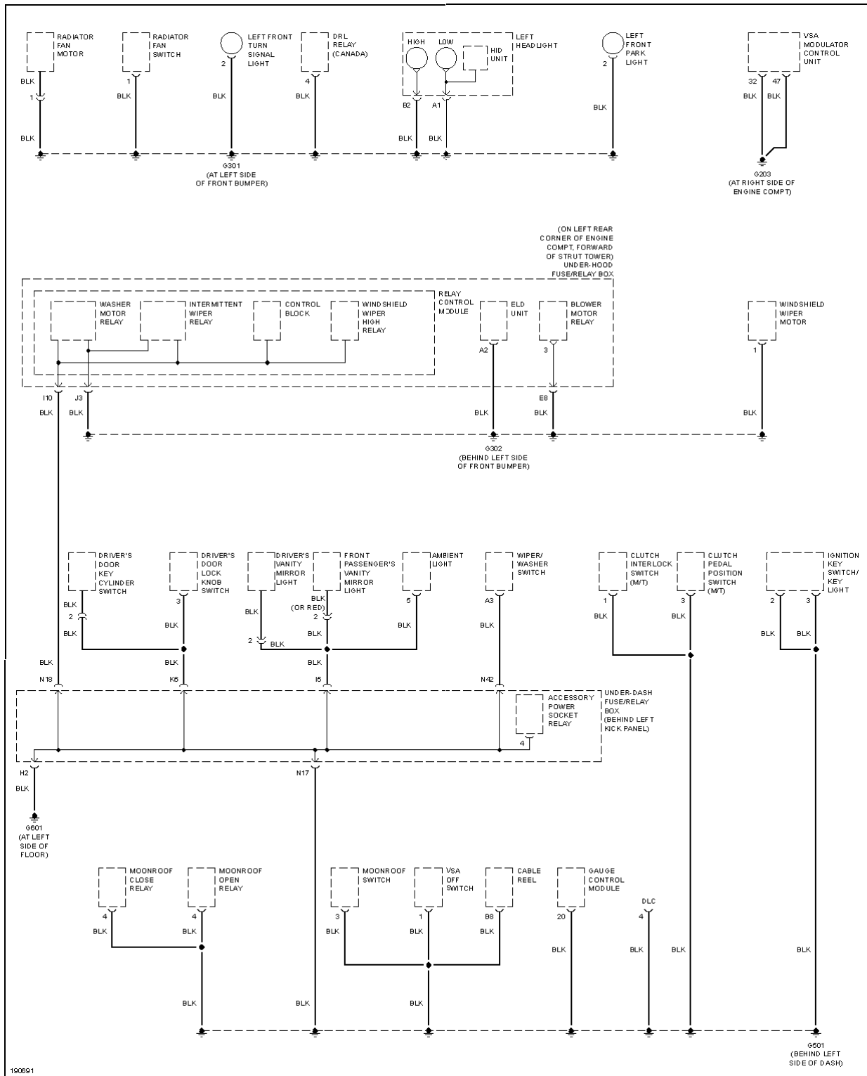
Fig. 25: Ground Distribution Circuit (2 of 4)
