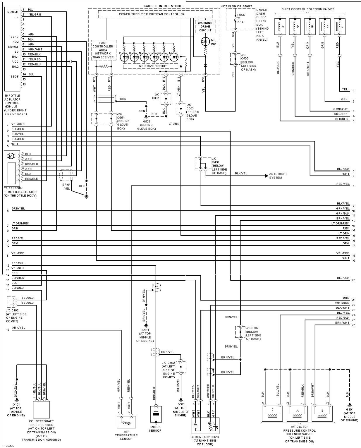
Fig. 18: 2.4L, Engine Performance Circuit (3 of 4)
