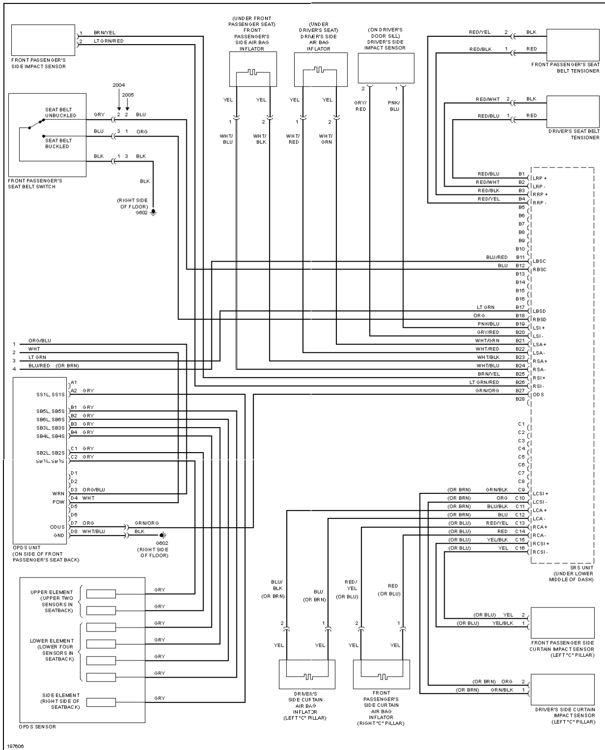
Fig. 68: Supplemental Restraints Circuit (2 of 2)
