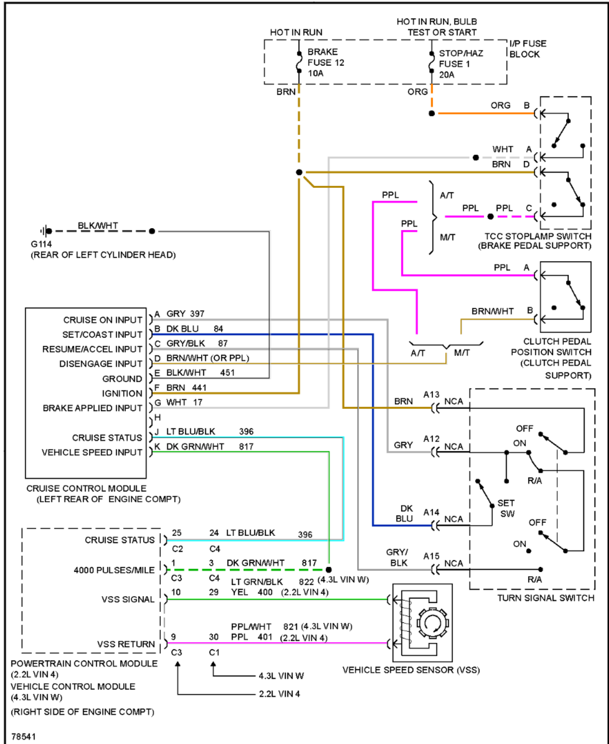
Fig. 4: Cruise Control Circuit
