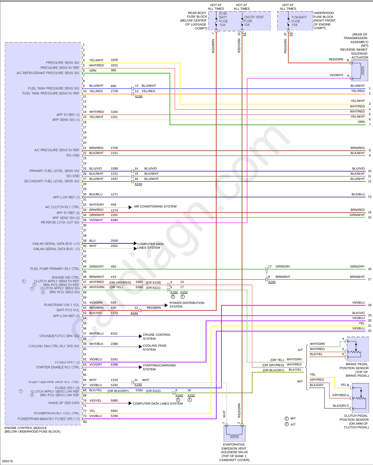
Fig 1: 6.2L VIN 7, Engine Performance Circuit (1 of 8)
