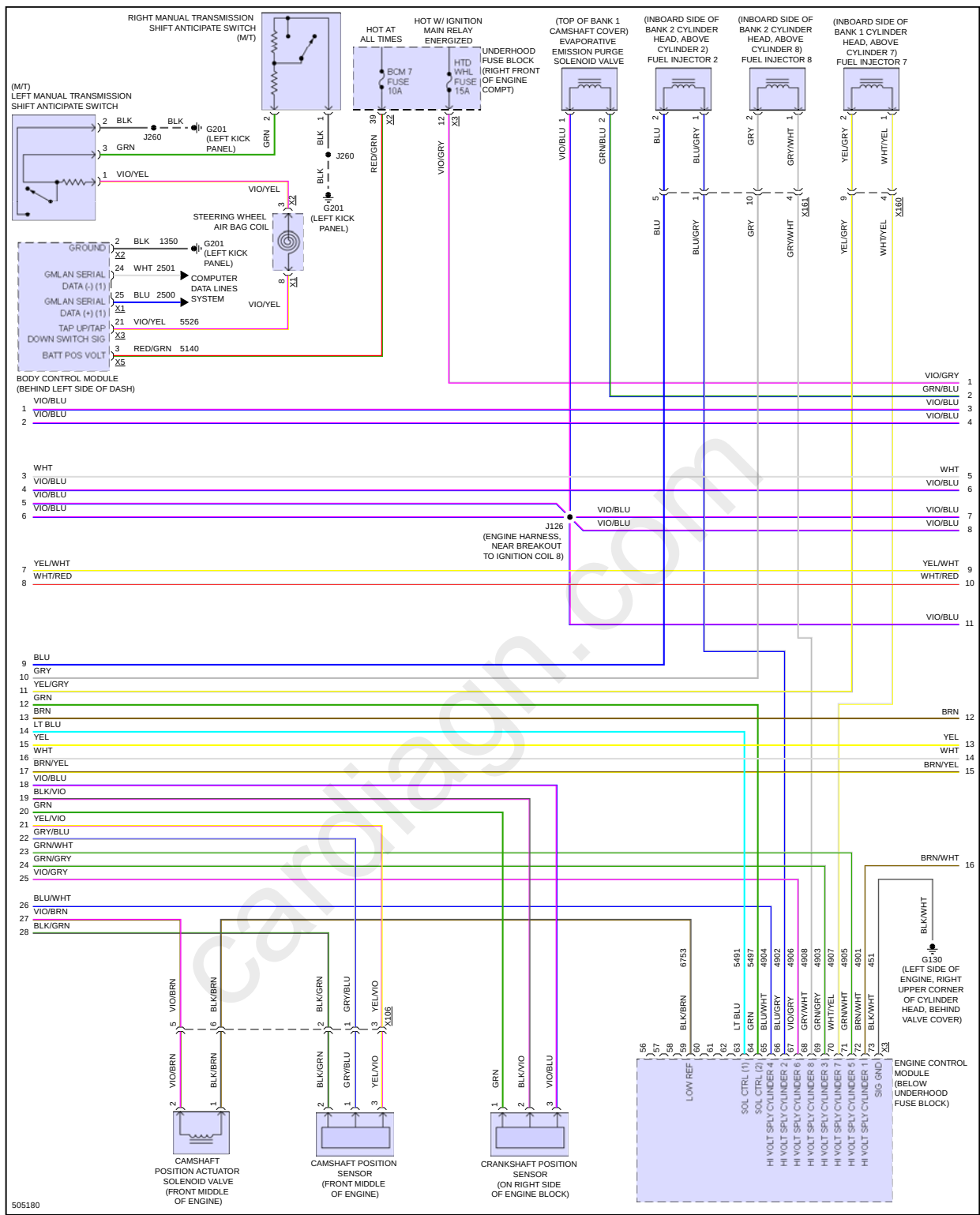
Fig 6: 6.2L VIN 7, Engine Performance Circuit (6 of 8)
