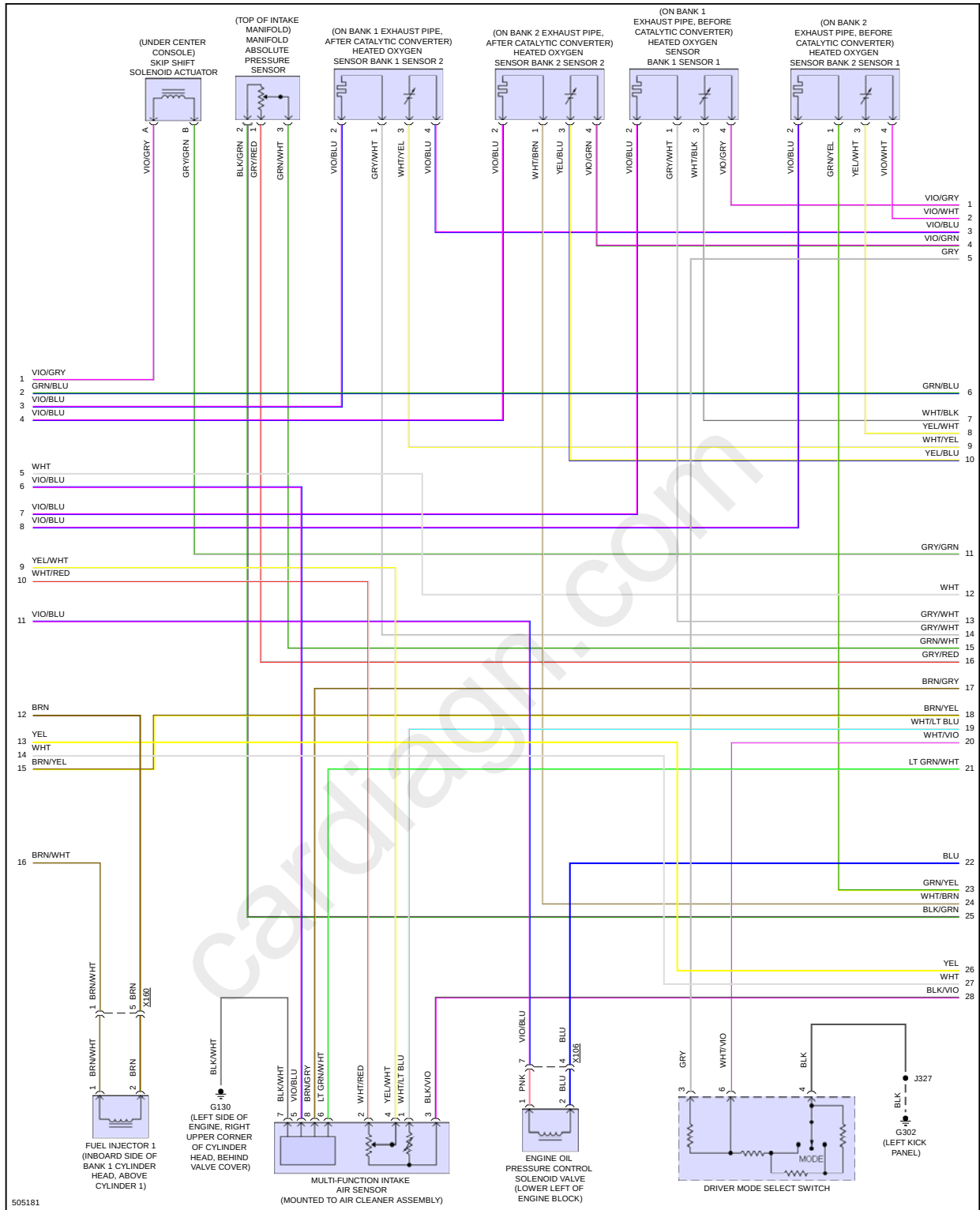
Fig 7: 6.2L VIN 7, Engine Performance Circuit (7 of 8)
