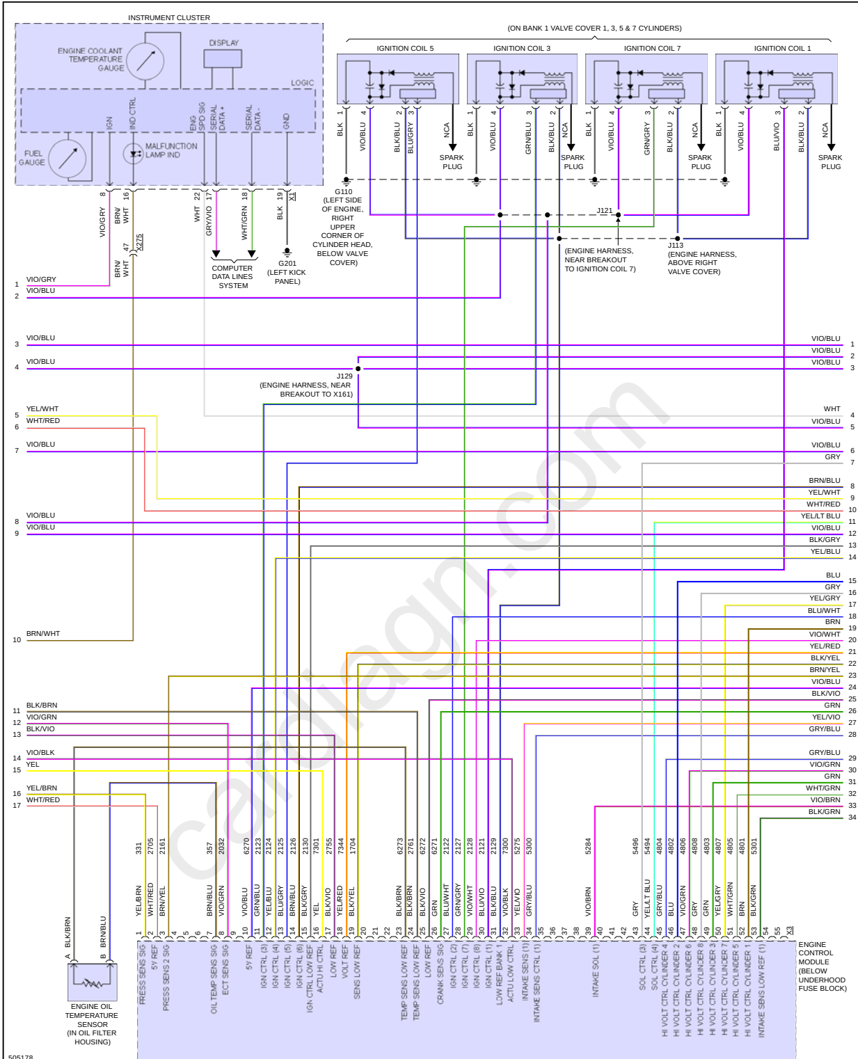
Fig 4: 6.2L VIN 7, Engine Performance Circuit (4 of 8)
