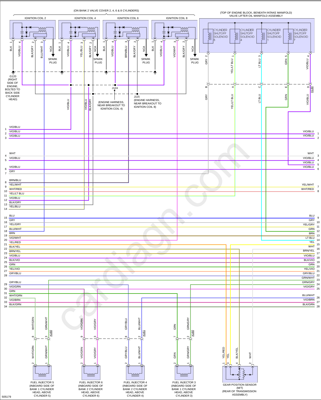
Fig 5: 6.2L VIN 7, Engine Performance Circuit (5 of 8)
