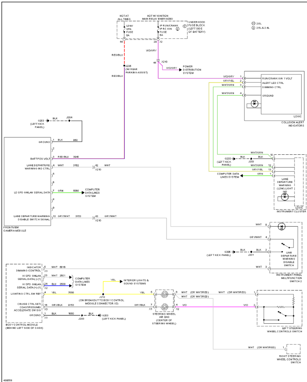
Fig. 77: Lane Departure Warning Circuit
