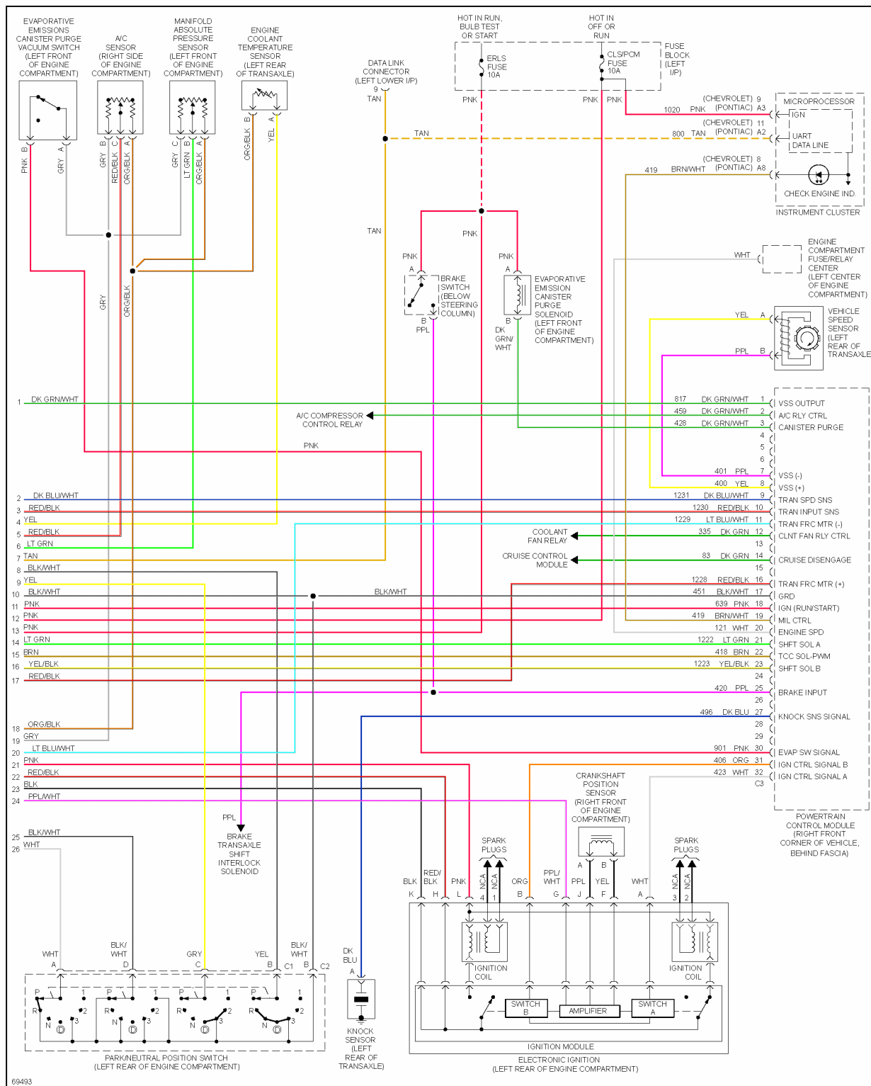
Fig. 14: 2.3L (VIN D), Engine Performance Circuits, A/T (3 of 3)
