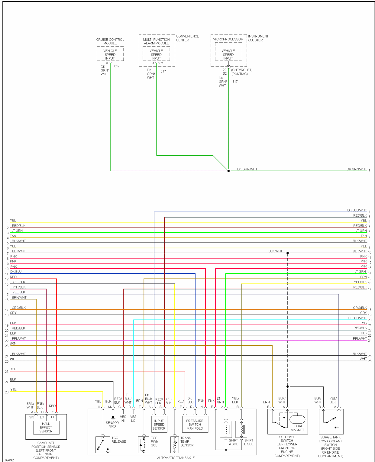
Fig. 13: 2.3L (VIN D), Engine Performance Circuits, A/T (2 of 3)
