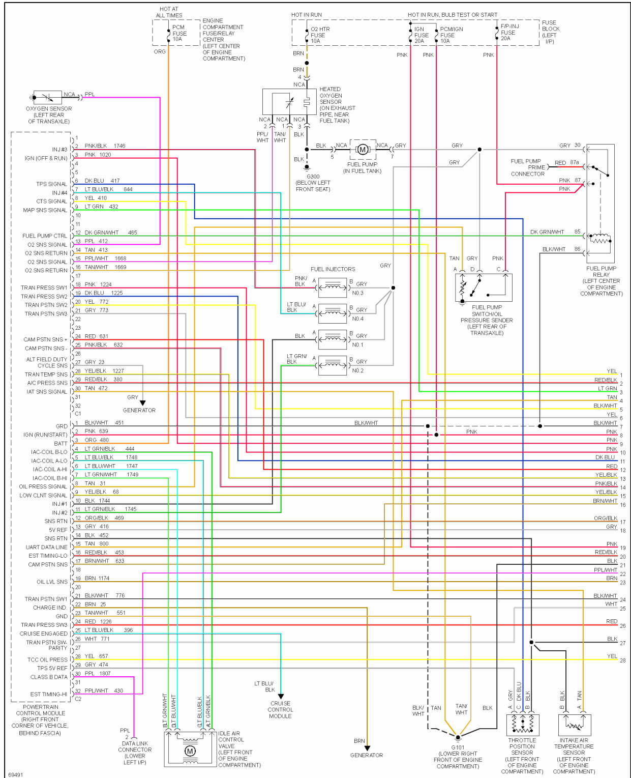
Fig. 12: 2.3L (VIN D), Engine Performance Circuits, A/T (1 of 3)
