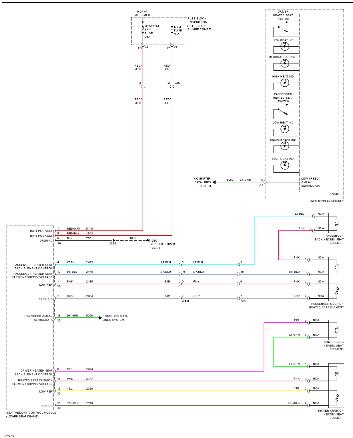
Fig. 61: Heated Seats Circuit, W/O SPO Heated Seats W/ Memory
