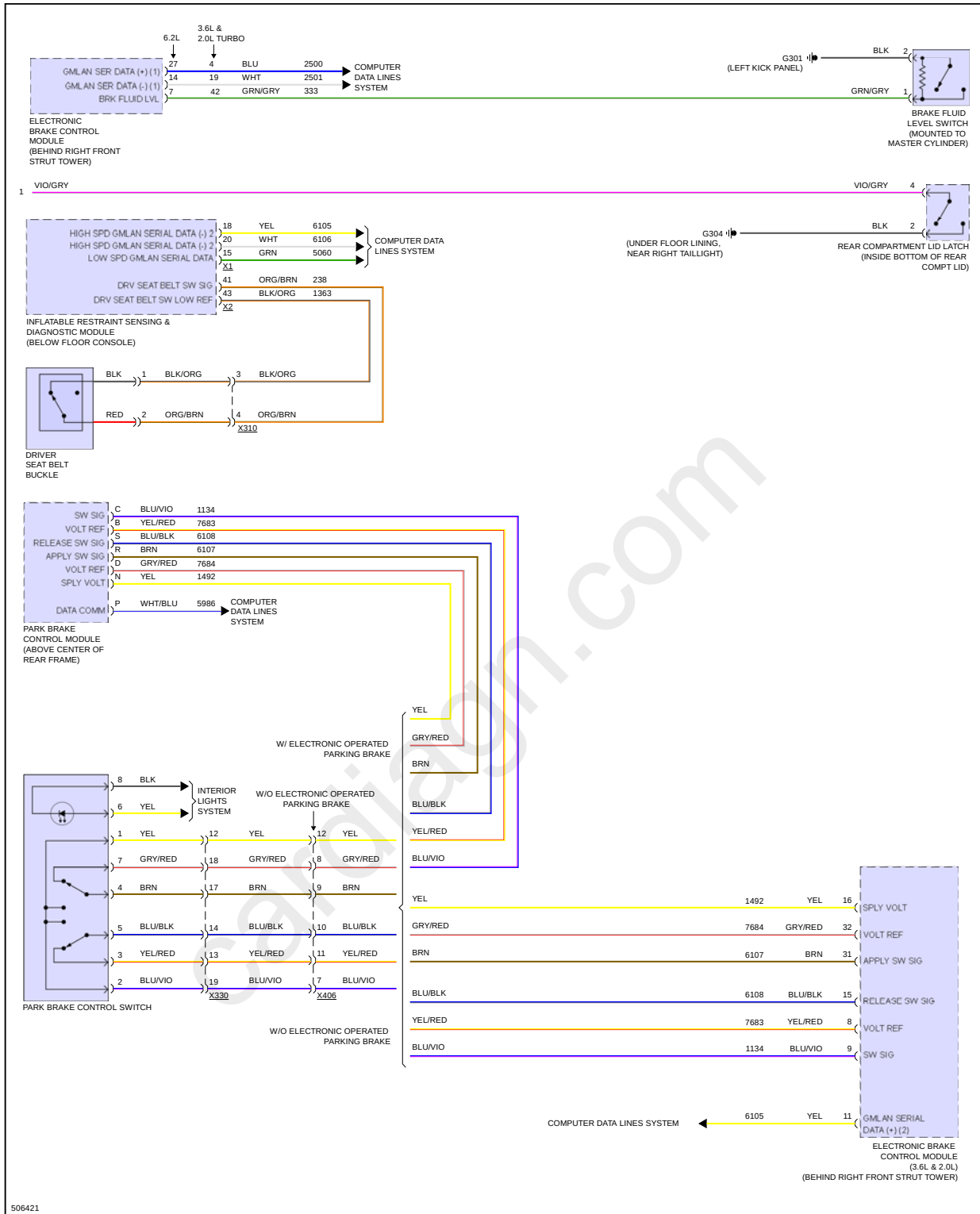
Fig 2: Warning Systems Circuit (2 of 2)
