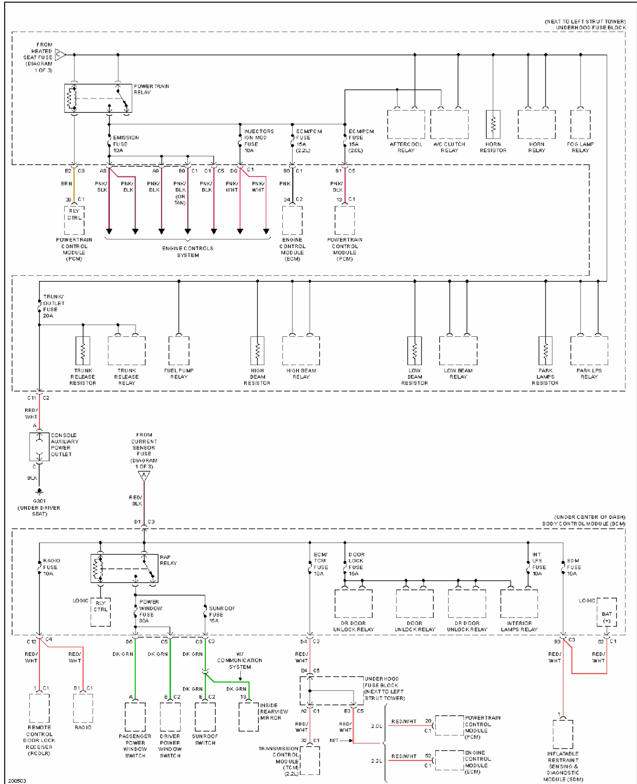
Fig. 41: Power Distribution Circuit (2 of 3)
