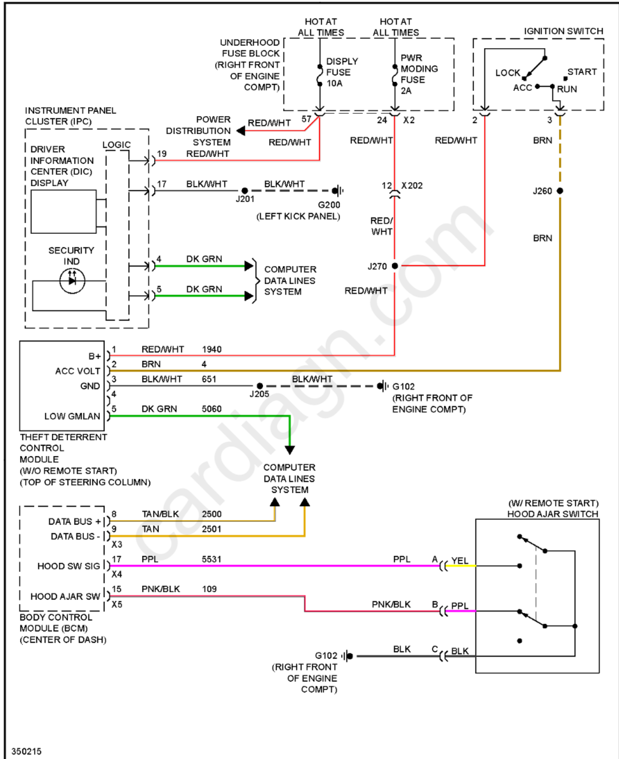
Fig. 9: Pass-Key Circuit
