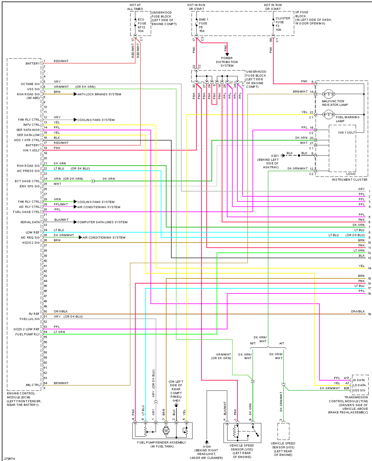
Fig. 27: 1.6L VIN 6, Engine Performance Circuit, Notchback W/O Throttle Actuator Control (1 of 4)
