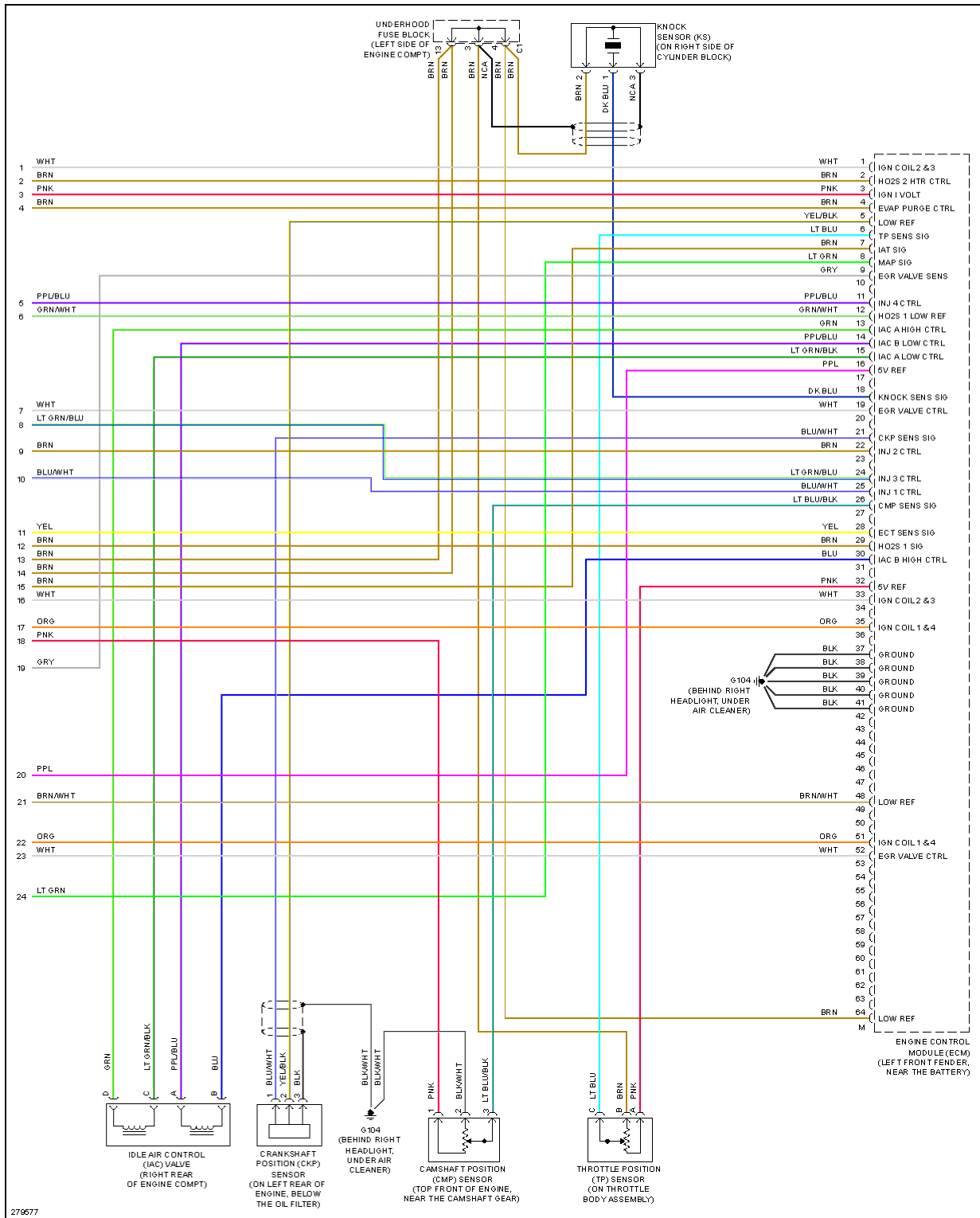
Fig. 30: 1.6L VIN 6, Engine Performance Circuit, Notchback W/O Throttle Actuator Control (4 of 4)
