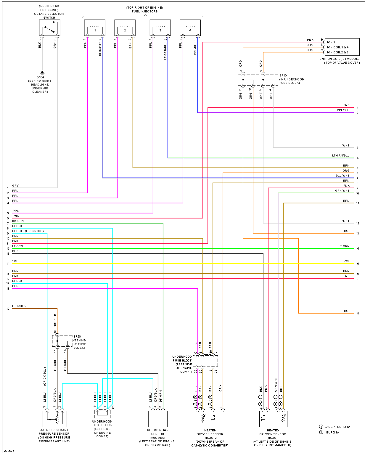
Fig. 28: 1.6L VIN 6, Engine Performance Circuit, Notchback W/O Throttle Actuator Control (2 of 4)
