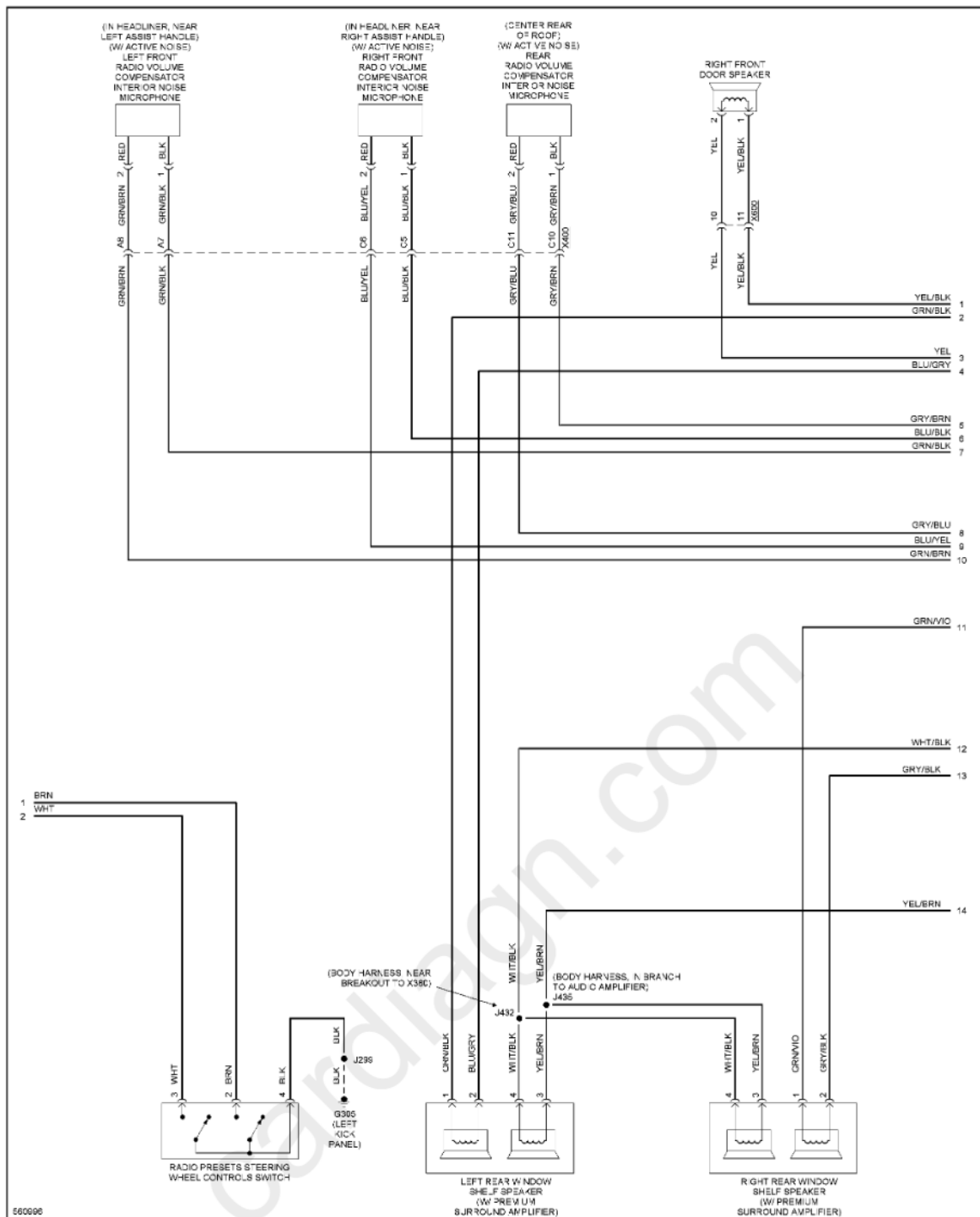
Fig. 113: Radio Circuit (4 of 5)
