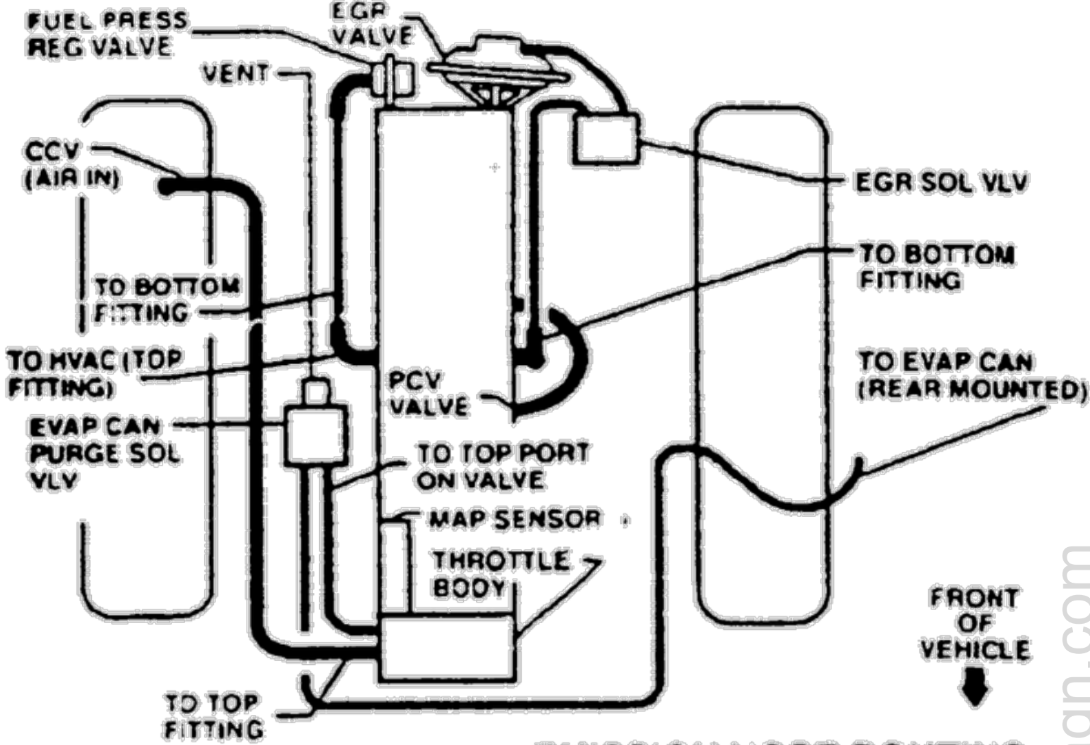
EMISSION HOSE ROUTING
