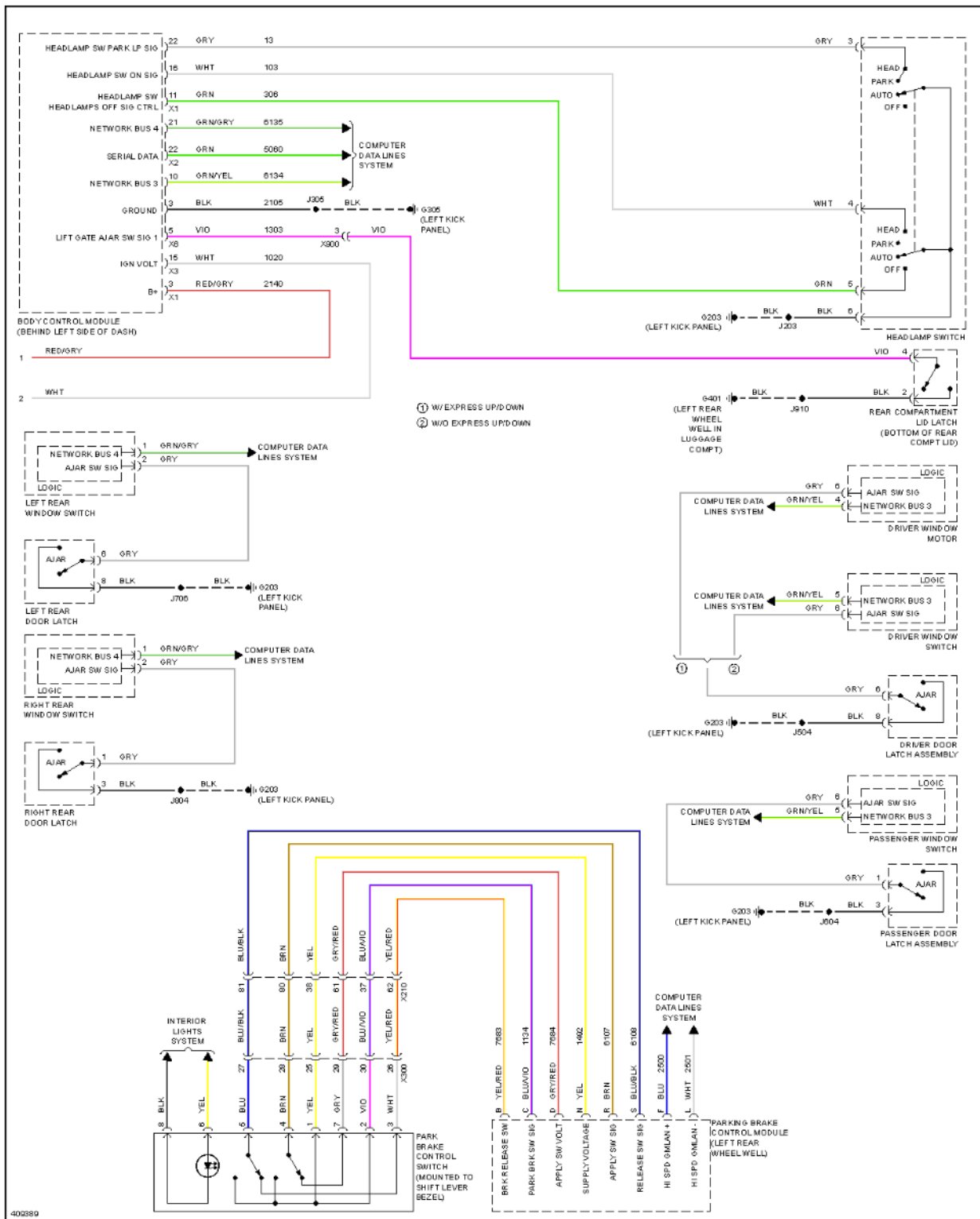
Fig. 138: Warning Systems Circuit (2 of 2)
