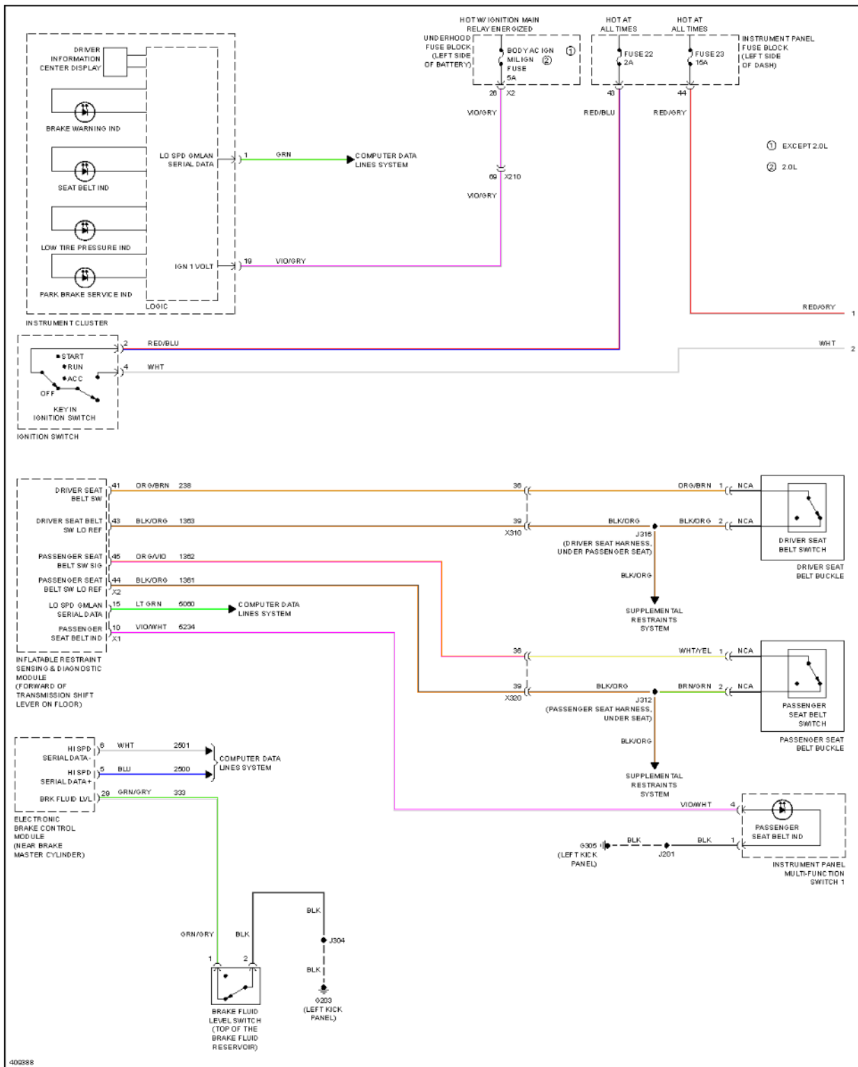
Fig. 137: Warning Systems Circuit (1 of 2)
