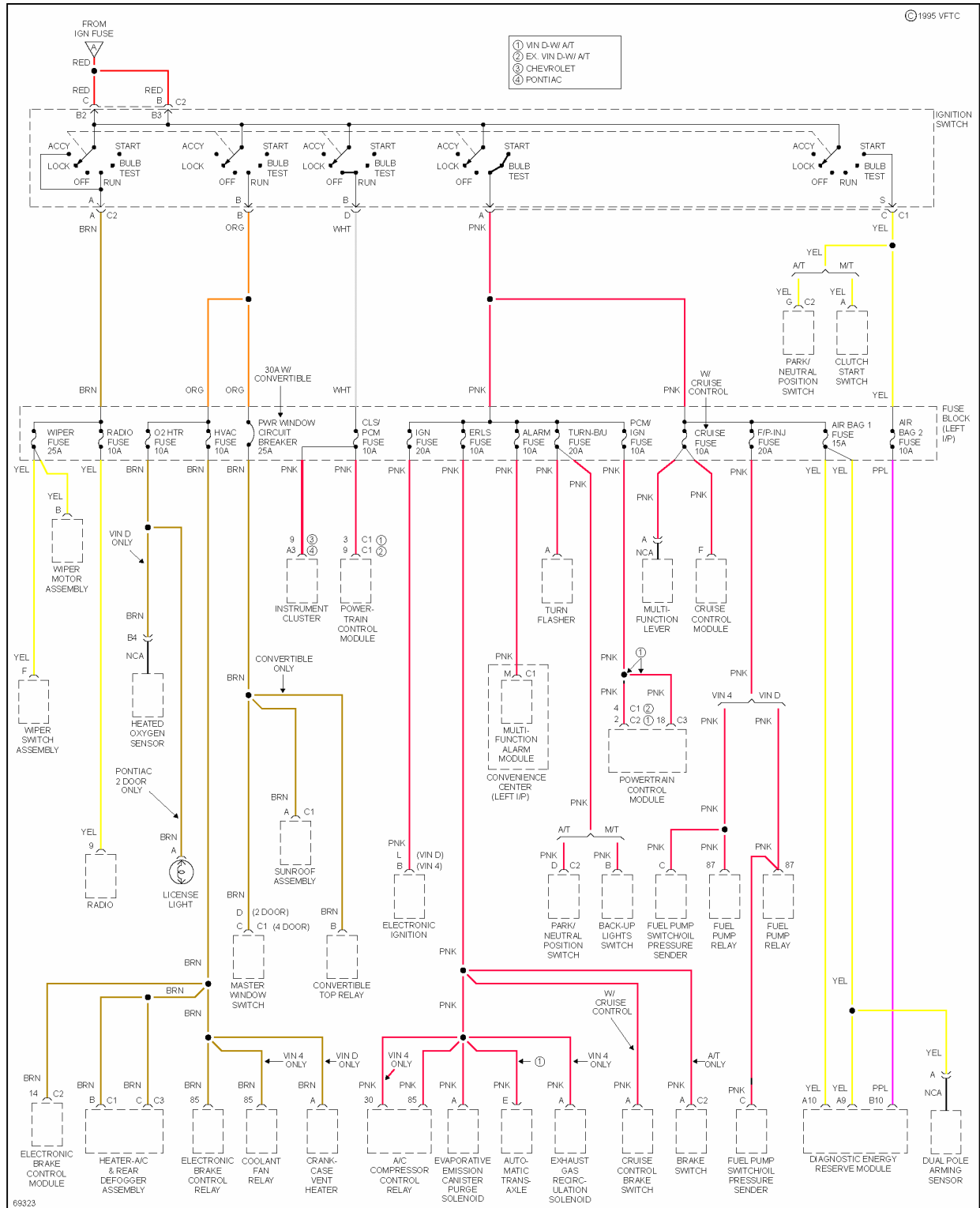
Fig. 31: Power Distribution Circuit (2 of 2)
