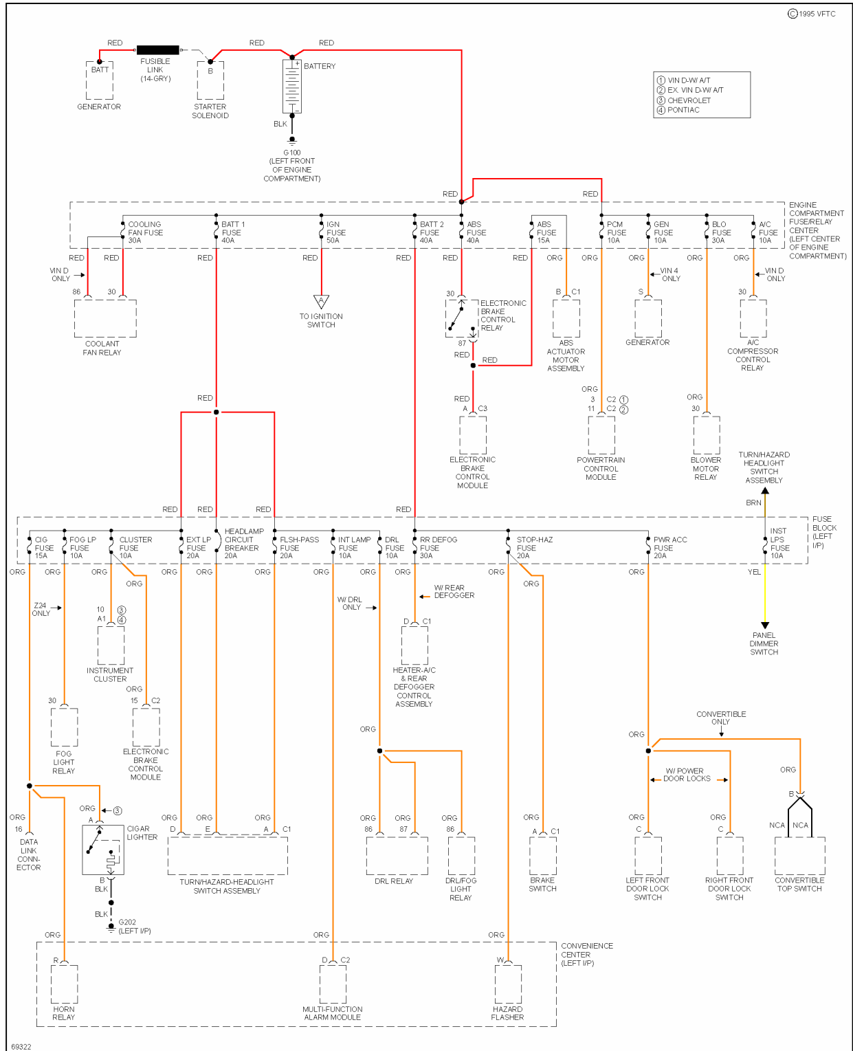
Fig. 30: Power Distribution Circuit (1 of 2)
