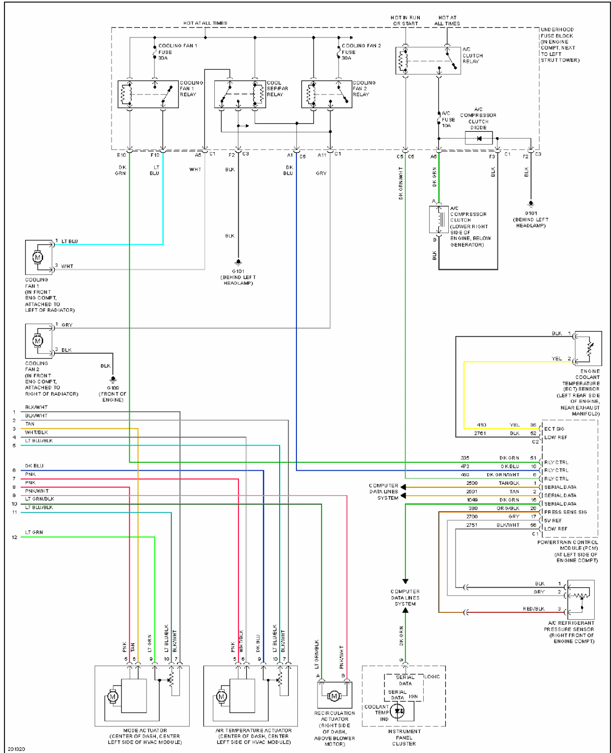
Fig. 3: 2.0L VIN P, Manual A/C Circuit (2 of 2)
