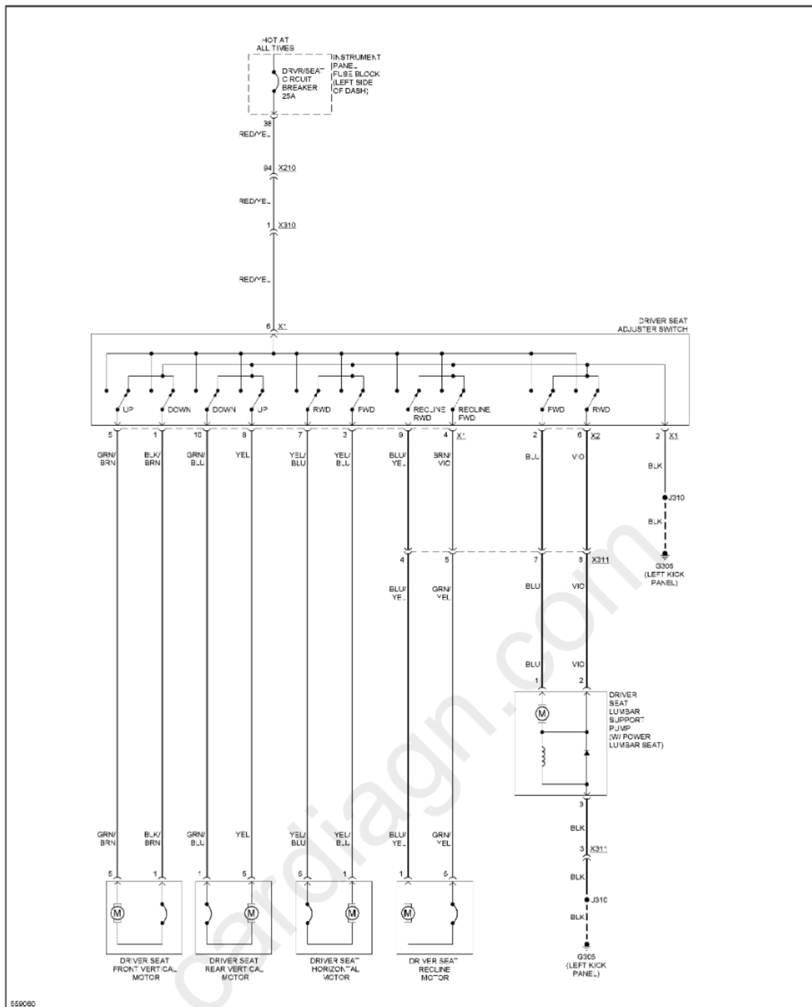
Fig. 101: Driver Power Seat Circuit
