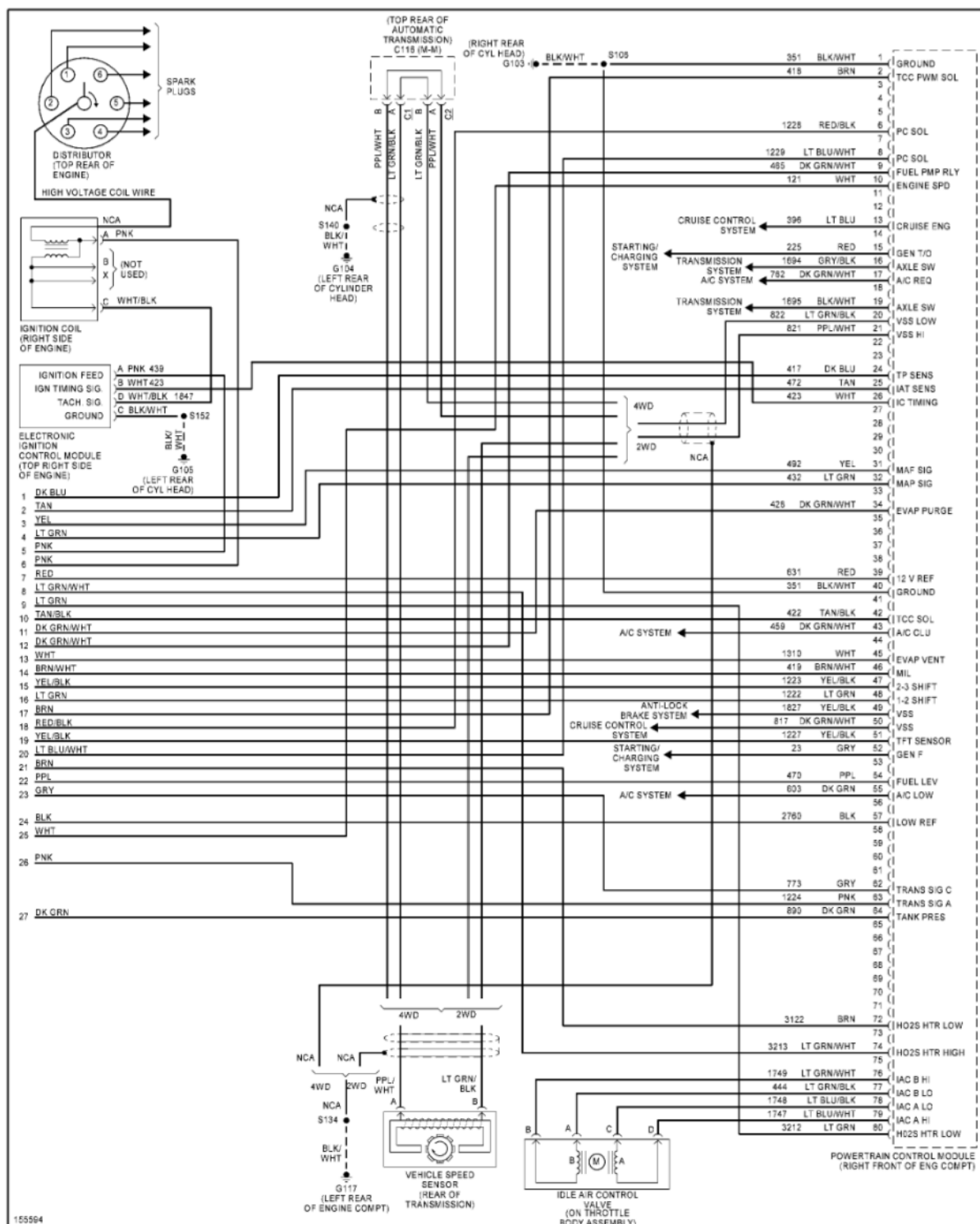
Fig. 16: 4.3L VIN W, Engine Performance Circuits (4 of 4)
