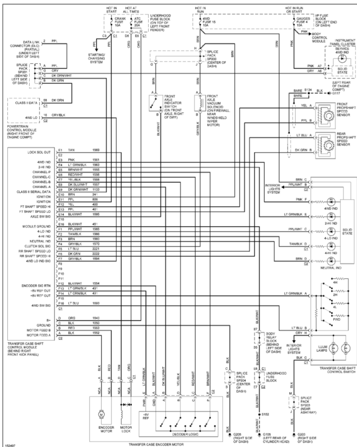
Fig. 56: 4.3L VIN W, Transfer Case Circuit, W/ 2-Speed Automatic Transfer Case
