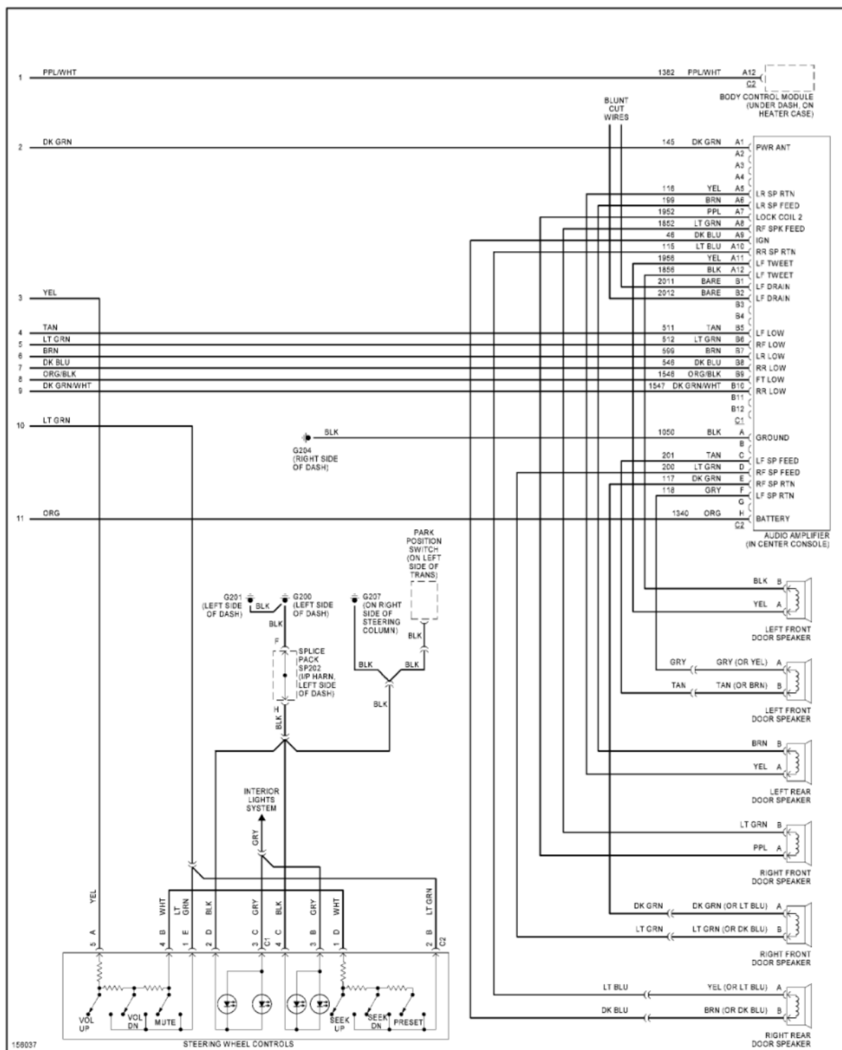
Fig. 48: Radio Circuits, W/ Amplifier (2 of 2)
