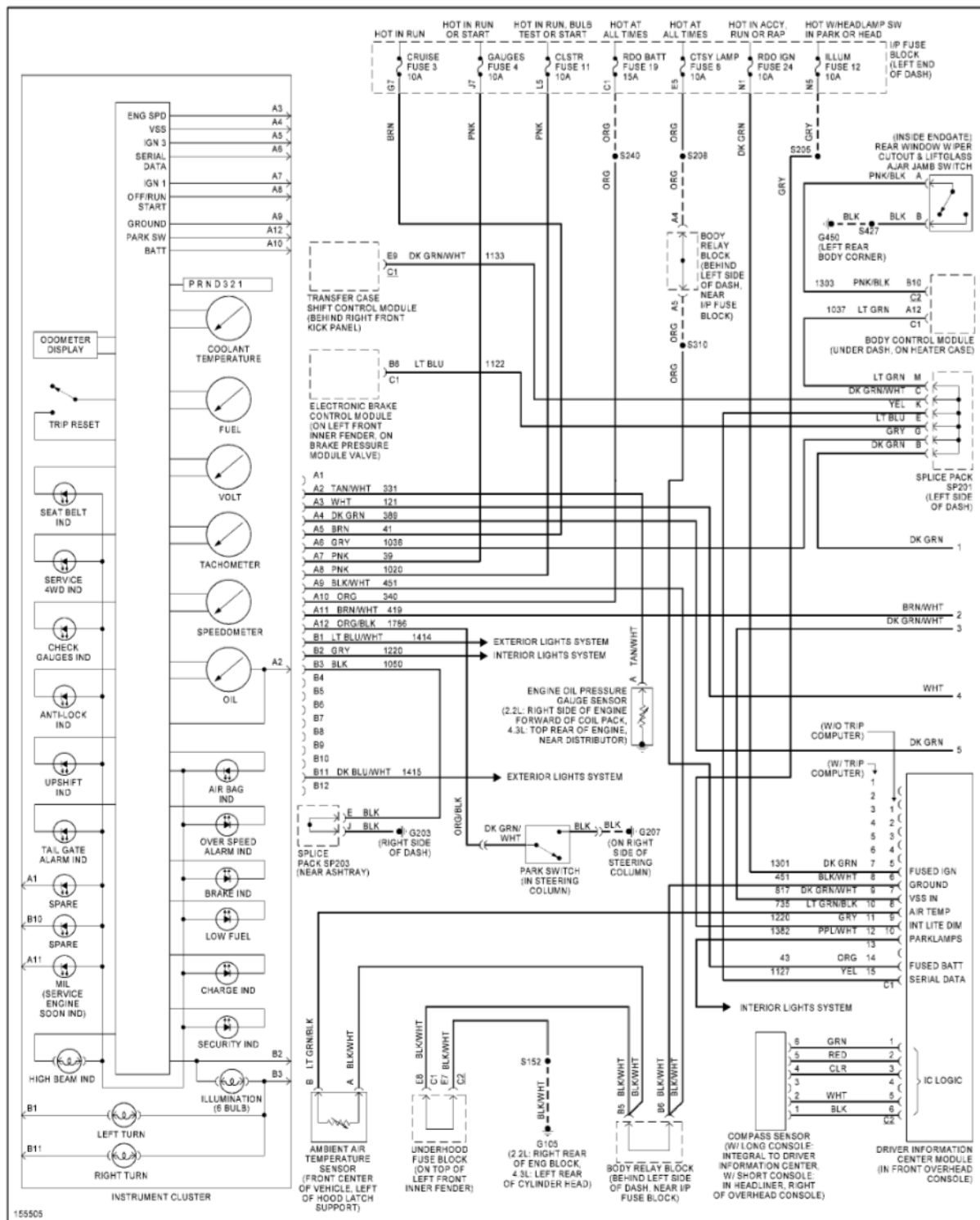
Fig. 25: Instrument Cluster Circuit (1 of 2)
