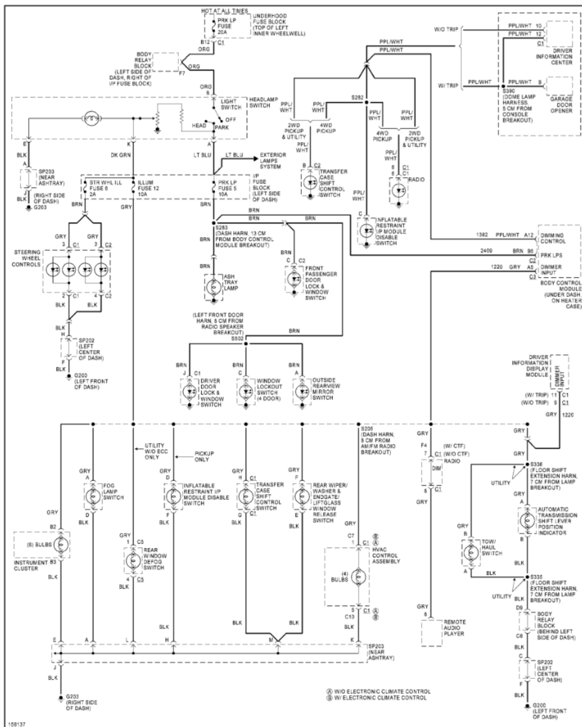
Fig. 29: Instrument Illumination Circuit
