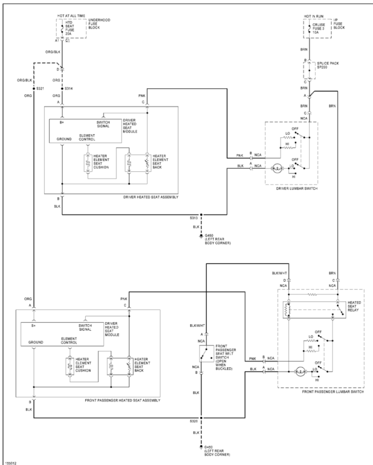
Fig. 41: Heated Seats Circuit
