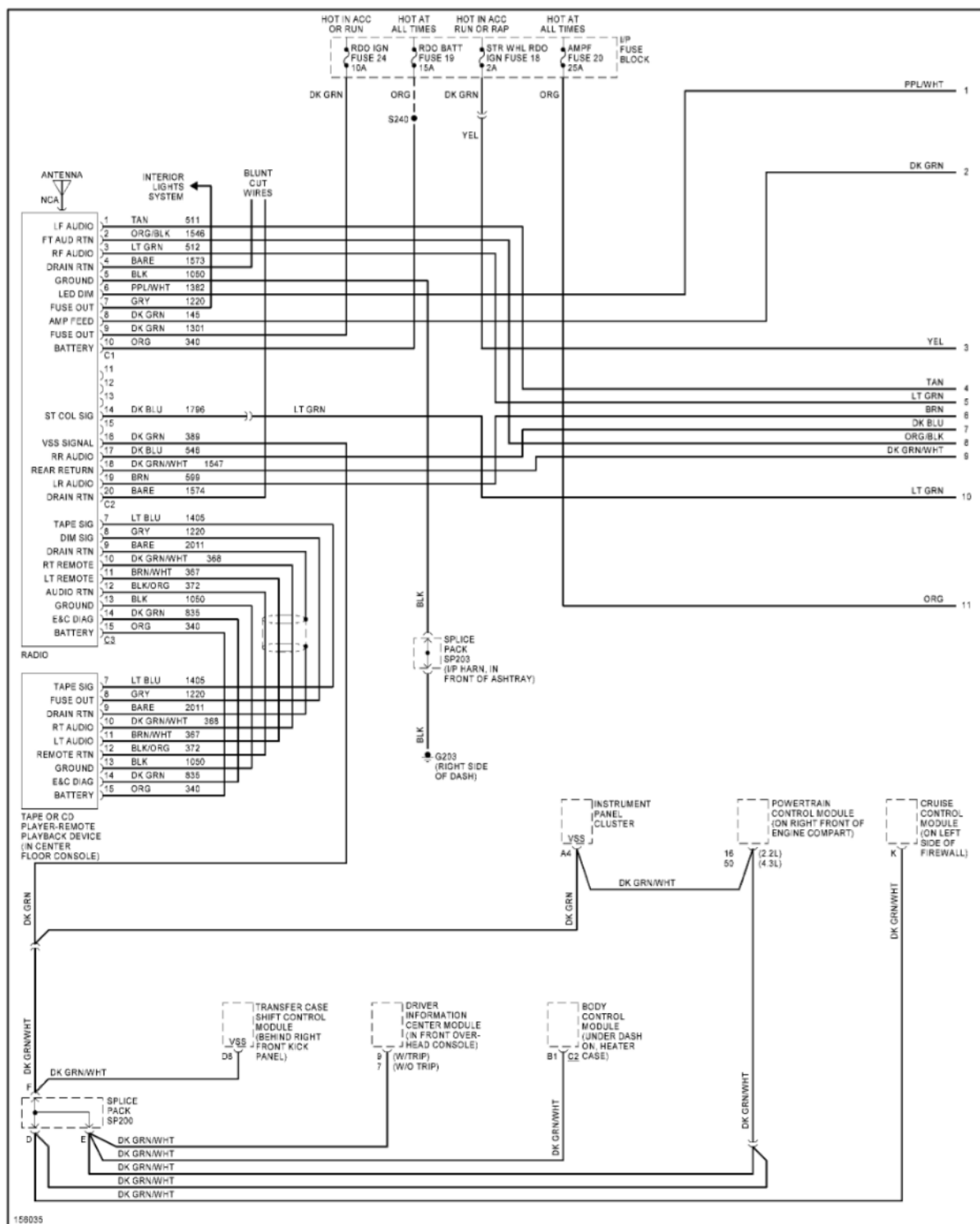
Fig. 47: Radio Circuits, W/ Amplifier (1 of 2)
