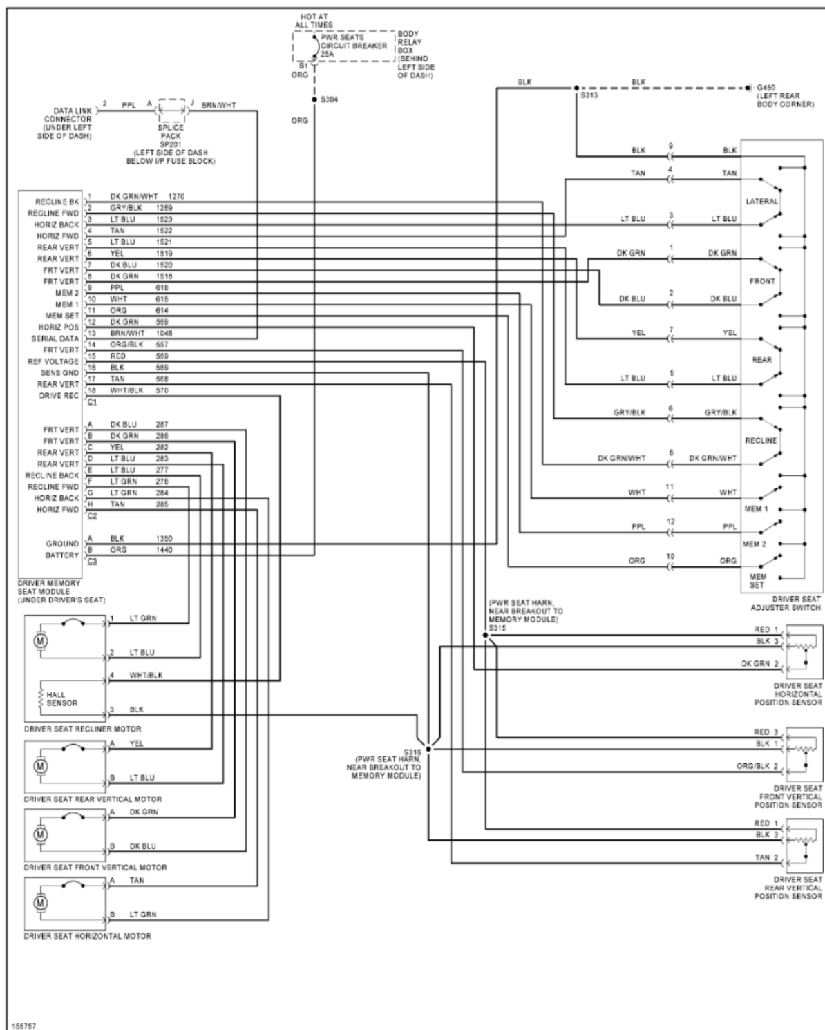
Fig. 30: Memory Seat Circuit
