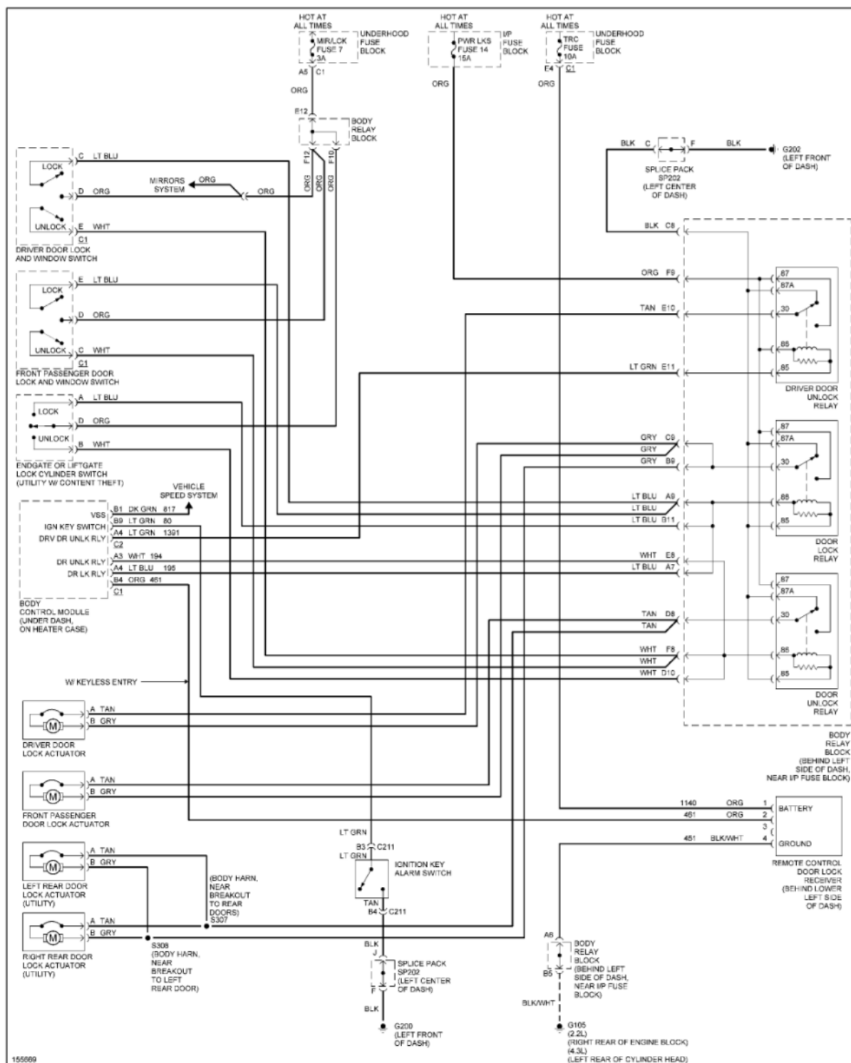
Fig. 36: Power Door Lock Circuit
