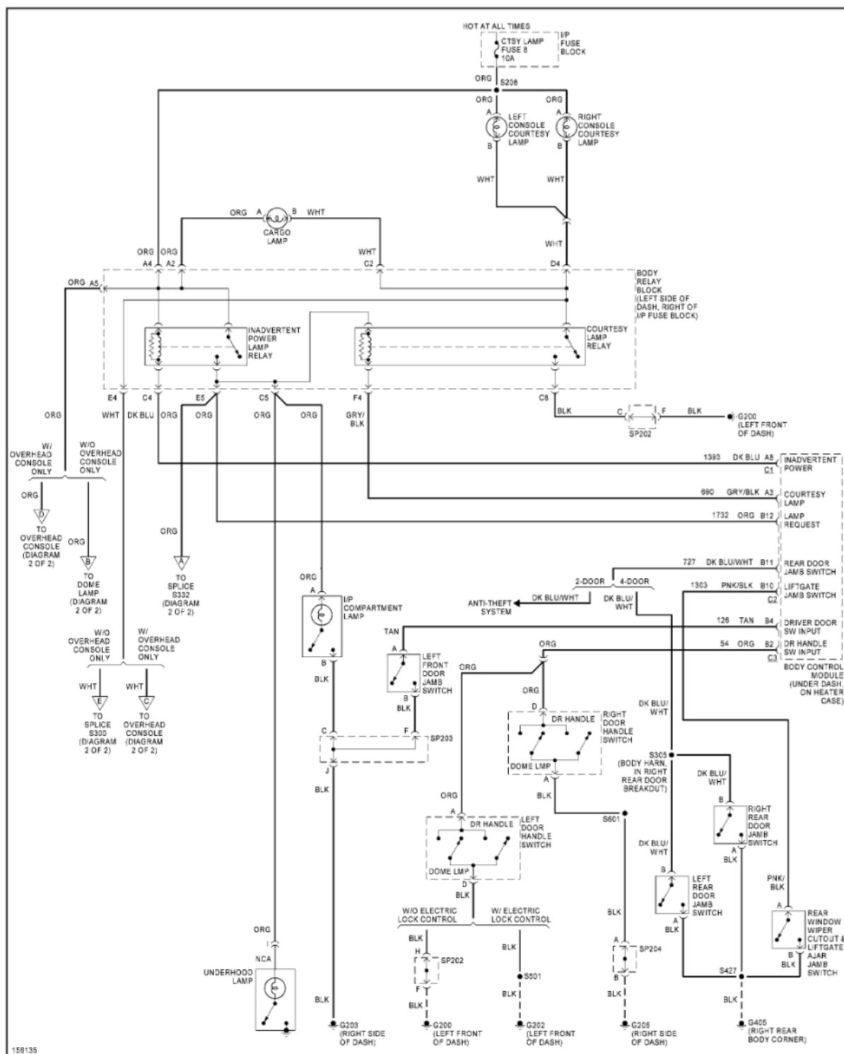
Fig. 27: Courtesy Lamps Circuit (1 of 2)
