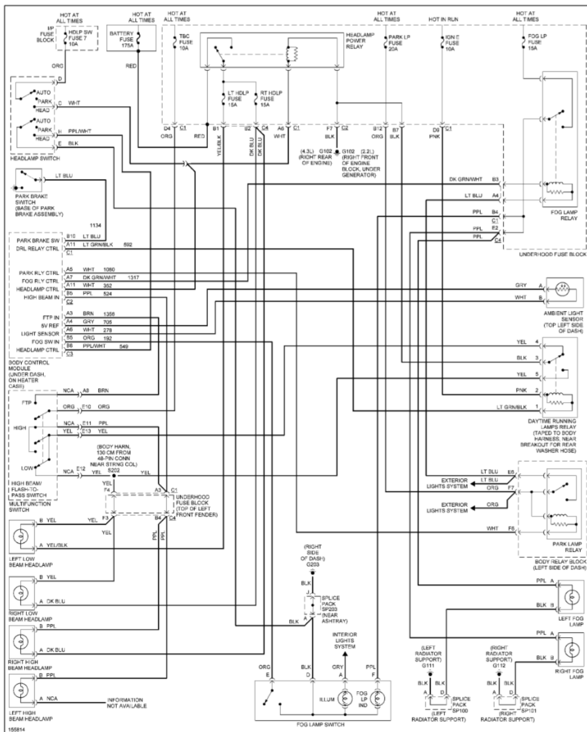
Fig. 22: Headlight Circuit, W/ ZR2
