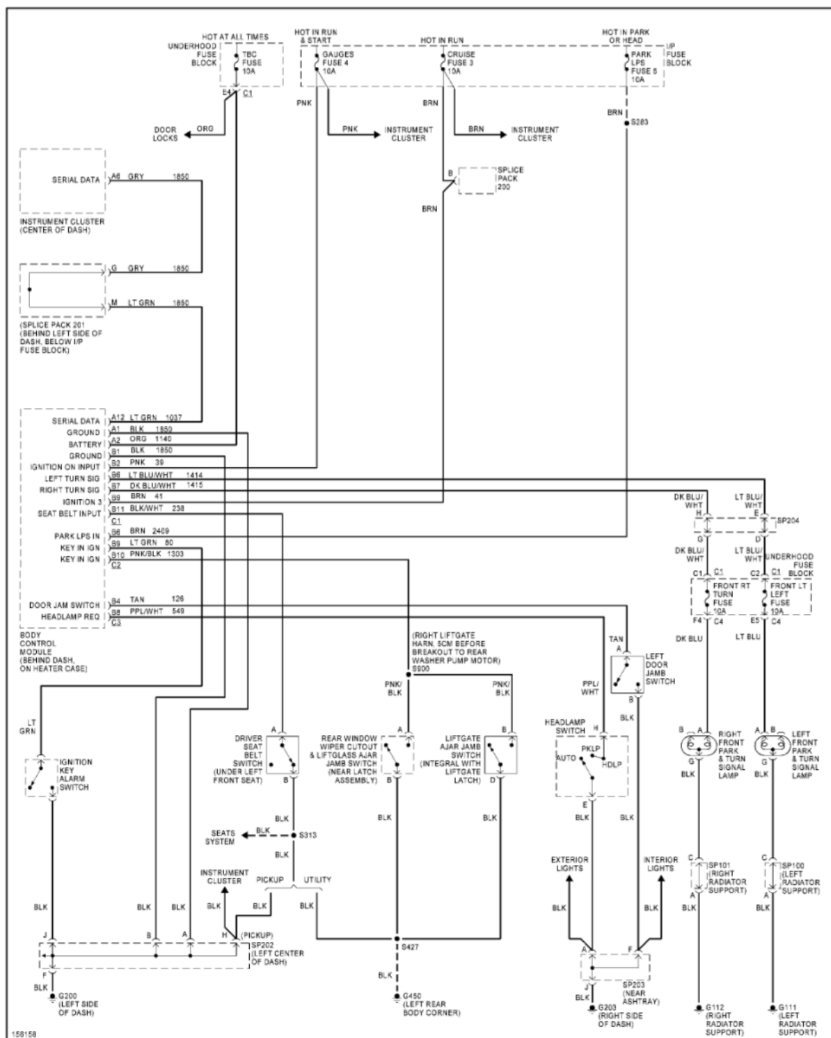
Fig. 59: Warning System Circuits
