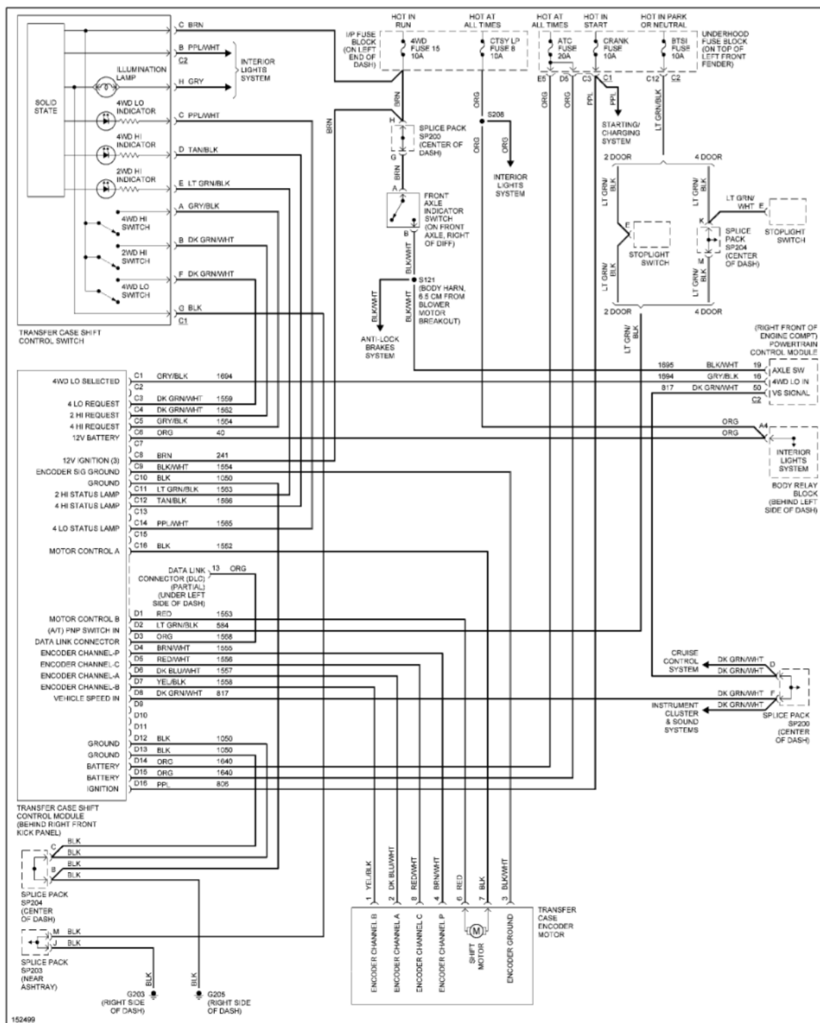
Fig. 57: 4.3L VIN W, Transfer Case Circuit, W/ 2-Speed Selectable Transfer Case
