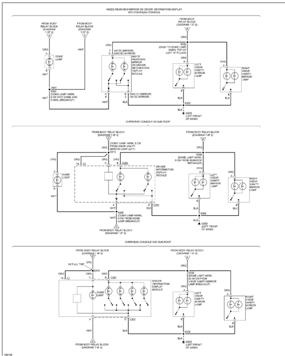
Fig. 28: Courtesy Lamps Circuit (2 of 2)
