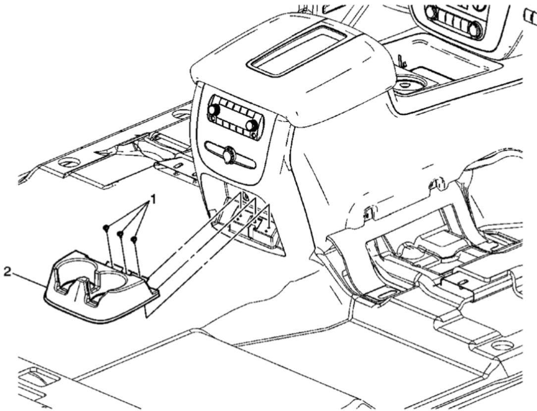
Fig. 39: View Of Front Floor Console Rear Cupholder Assembly & Screws Courtesy of GENERAL MOTORS CORP.
