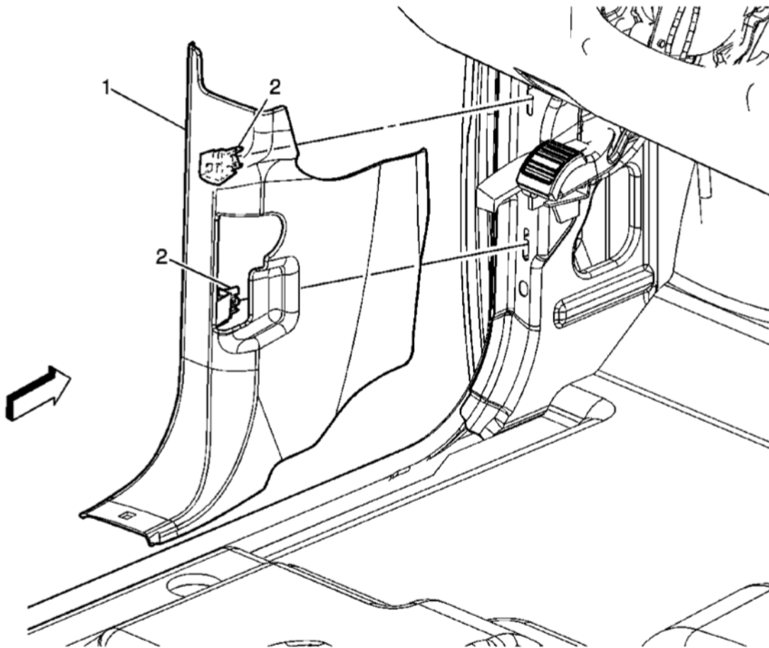
Fig. 25: View Of Front Hinge Pillar Trim Panel Assembly & Retainers Courtesy of GENERAL MOTORS CORP.
