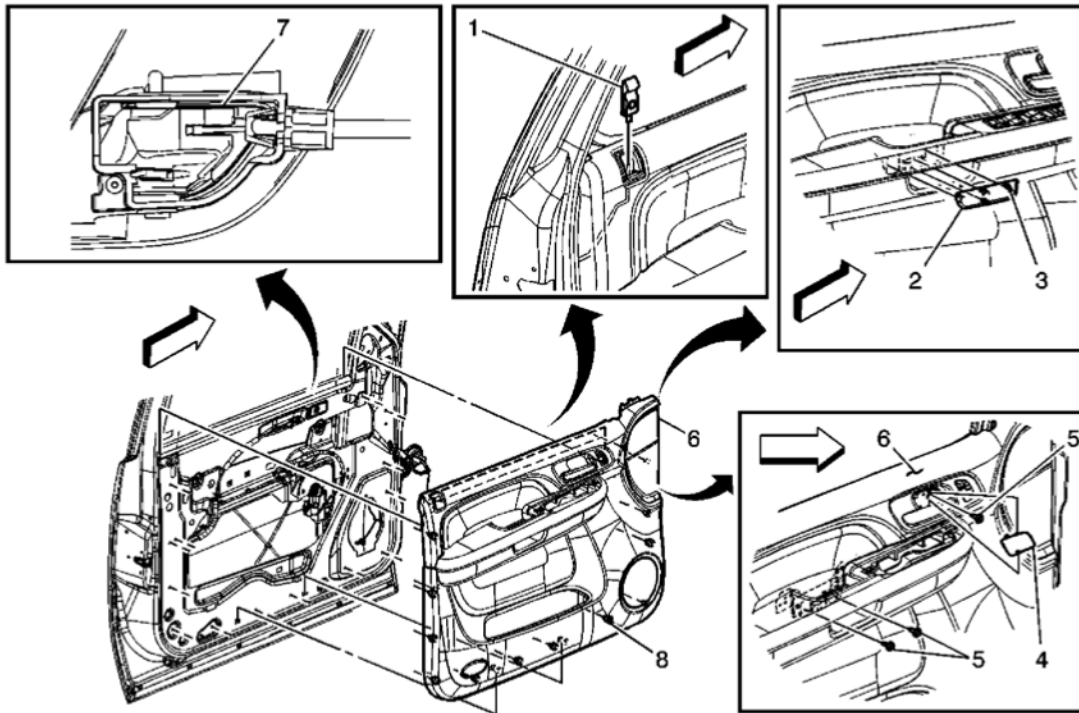
Fig. 3: View Of Front Side Door Trim Panel Assembly & Components Courtesy of GENERAL MOTORS CORP.
