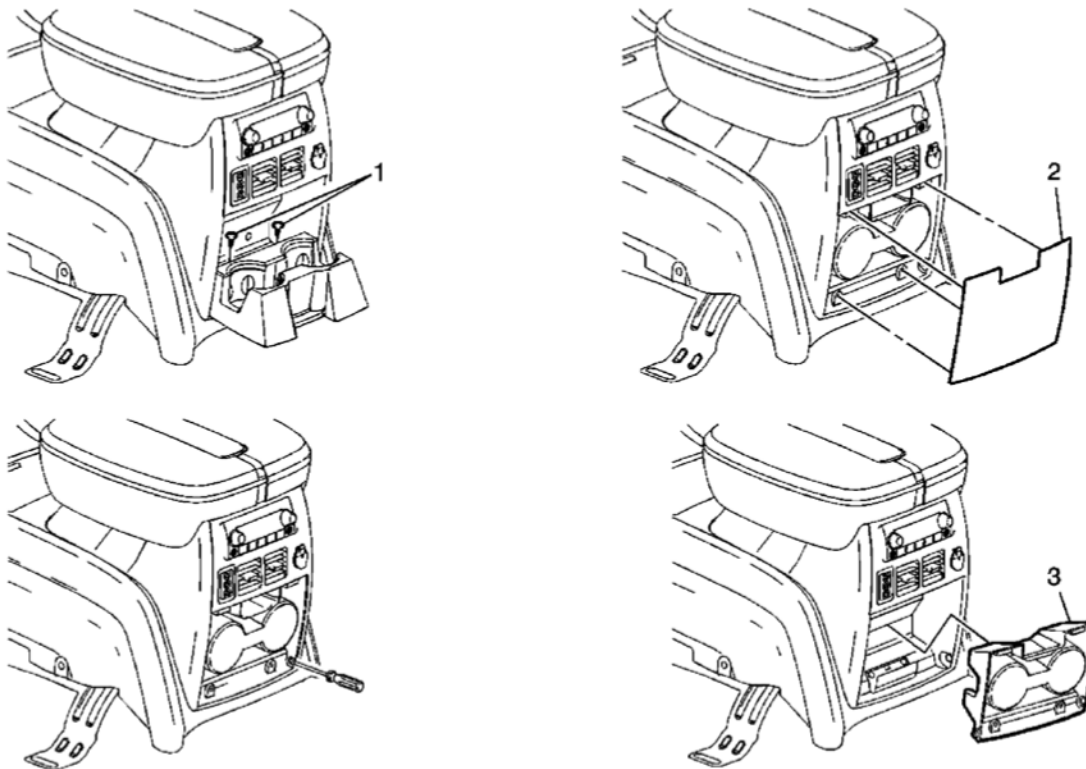
Fig. 38: View Of Front Floor Console Rear Cupholder Assembly, Door & Screws Courtesy of GENERAL MOTORS CORP.
