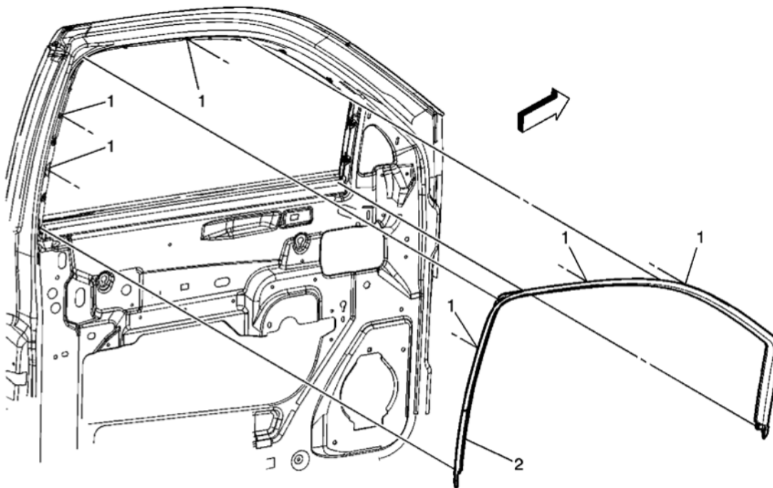
Fig. 8: View Of Front Side Door Window Garnish Molding & Retainers Courtesy of GENERAL MOTORS CORP.
