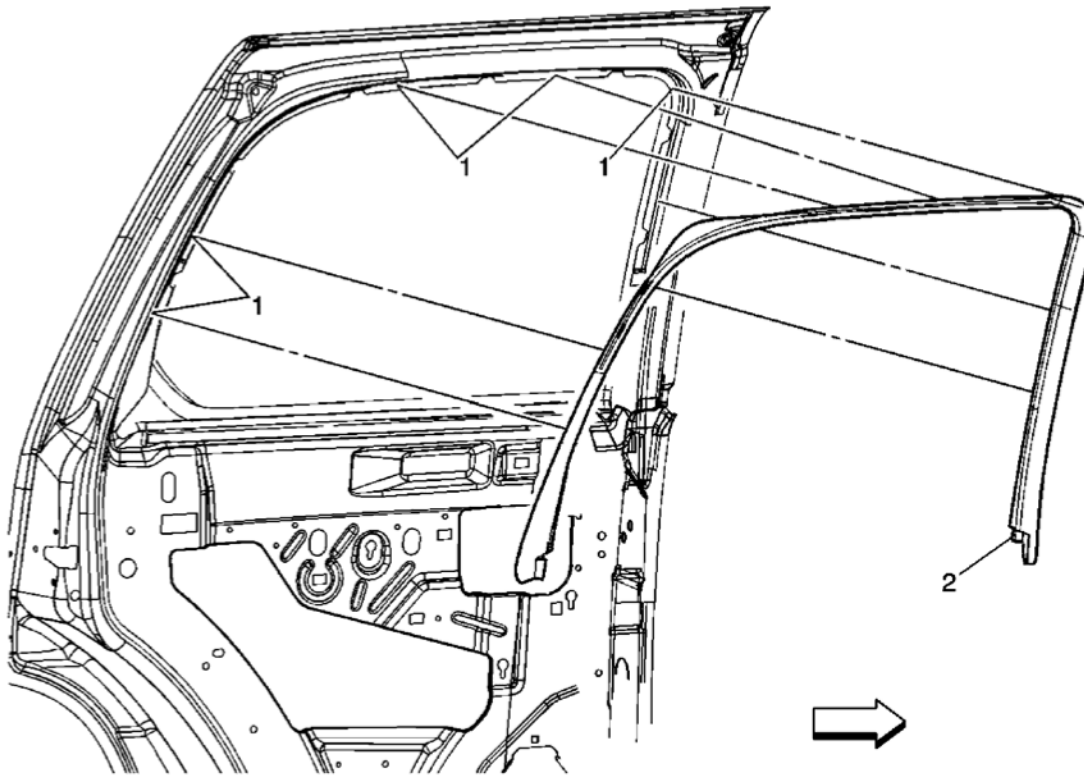
Fig. 9: View Of Rear Side Door Window Garnish Molding & Retainers Courtesy of GENERAL MOTORS CORP.
