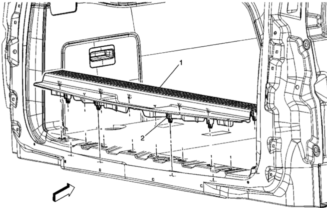
Fig. 14: View Of Rear Floor Rear Trimplate Assembly & Retainers Courtesy of GENERAL MOTORS CORP.
