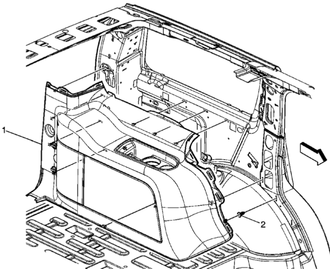
Fig. 29: View Of Body Side Trim Panel Assembly & Retainers Courtesy of GENERAL MOTORS CORP.
