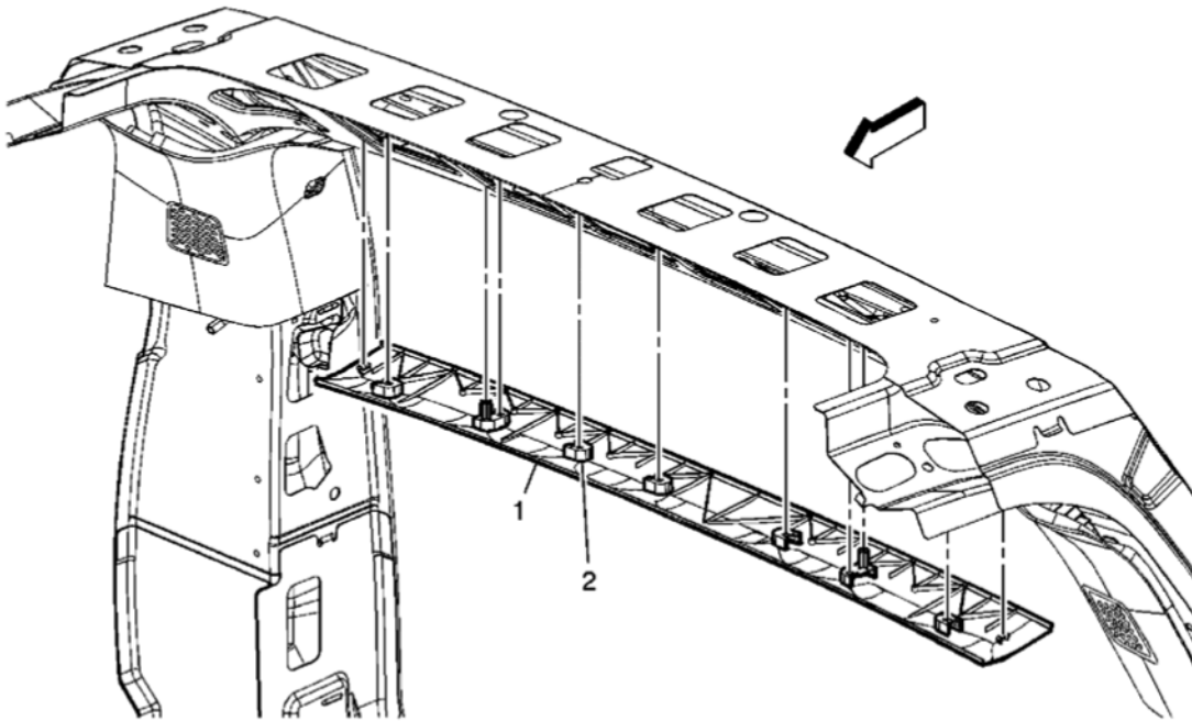
Fig. 24: View Of Back Body Opening Garnish Molding Assembly & Clips Courtesy of GENERAL MOTORS CORP.
