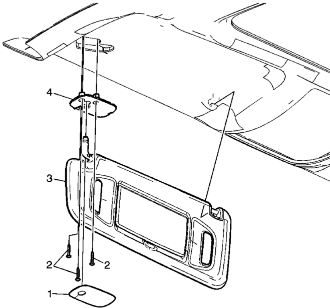
Fig. 18: View Of Sunshade Assembly & Components Courtesy of GENERAL MOTORS CORP.
