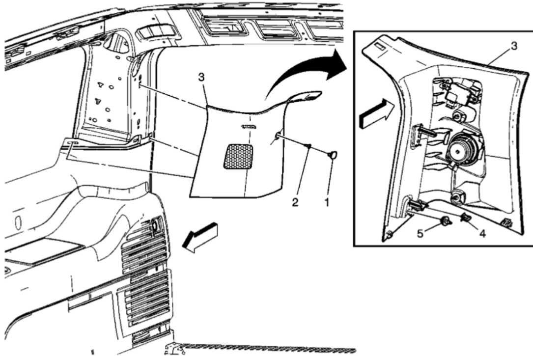
Fig. 23: View Of Body Rear Corner Upper Garnish Molding Assembly & Components Courtesy of GENERAL MOTORS CORP.
