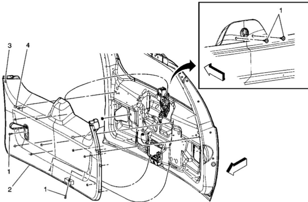
Fig. 34: View Of Liftgate Trim Finish Panel Assembly & Components Courtesy of GENERAL MOTORS CORP.
