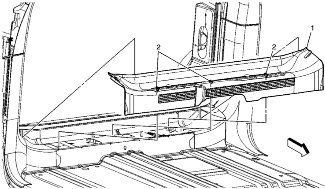
Fig. 35: View Of Rear Floor Trim Plate Assembly & Retainers Courtesy of GENERAL MOTORS CORP.
