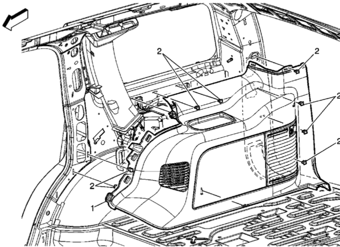
Fig. 31: View Of Body Side Trim Panel Assembly & Retainers
