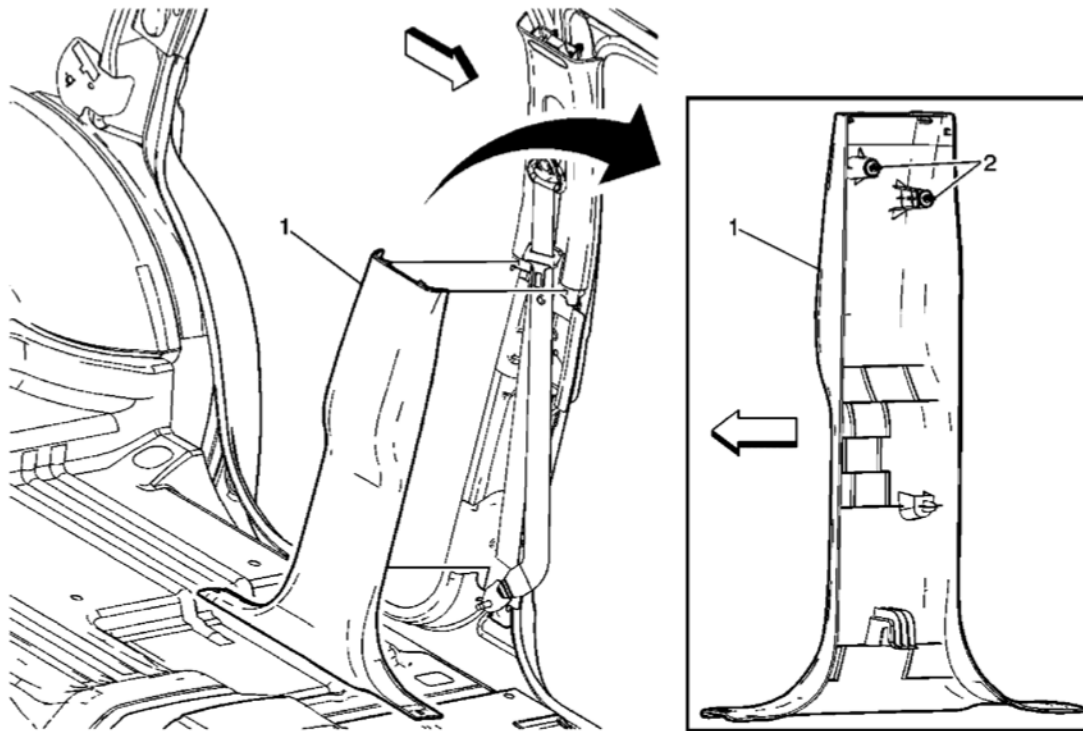
Fig. 21: View Of Center Pillar Lower Garnish Molding Assembly & Retainers Courtesy of GENERAL MOTORS CORP.
