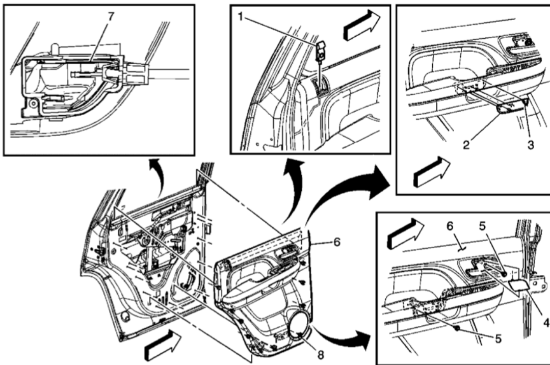
Fig. 5: View Of Rear Side Door Trim Panel Assembly & Components Courtesy of GENERAL MOTORS CORP.
