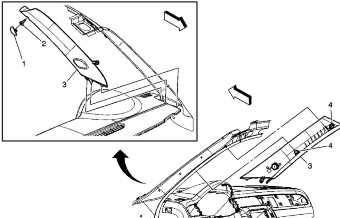
Fig. 19: View Of Windshield Side Garnish Molding Assembly Courtesy of GENERAL MOTORS CORP.
