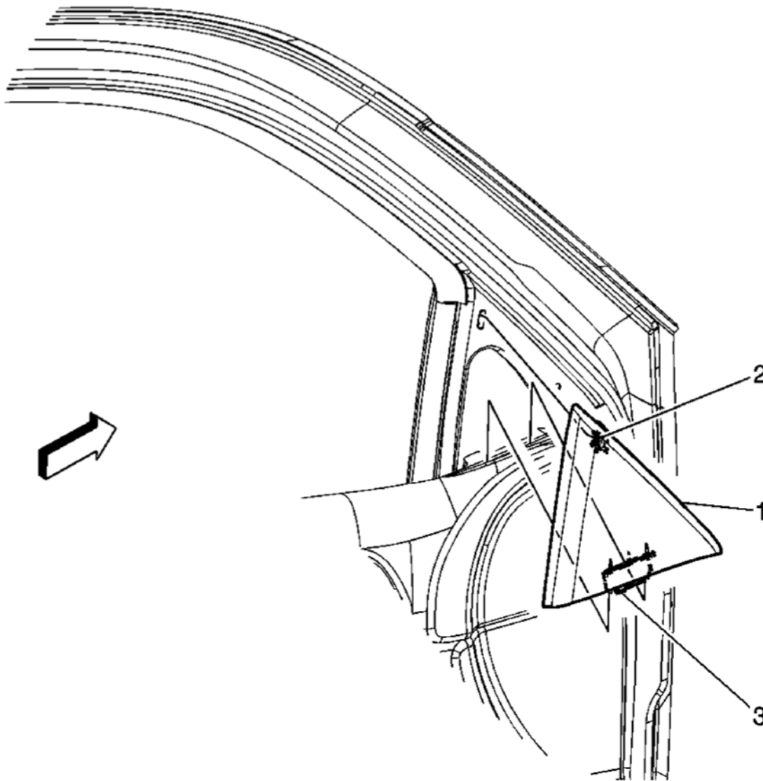
Fig. 1: View Of Front Side Door Trim Panel Assembly & Components Courtesy of GENERAL MOTORS CORP.
