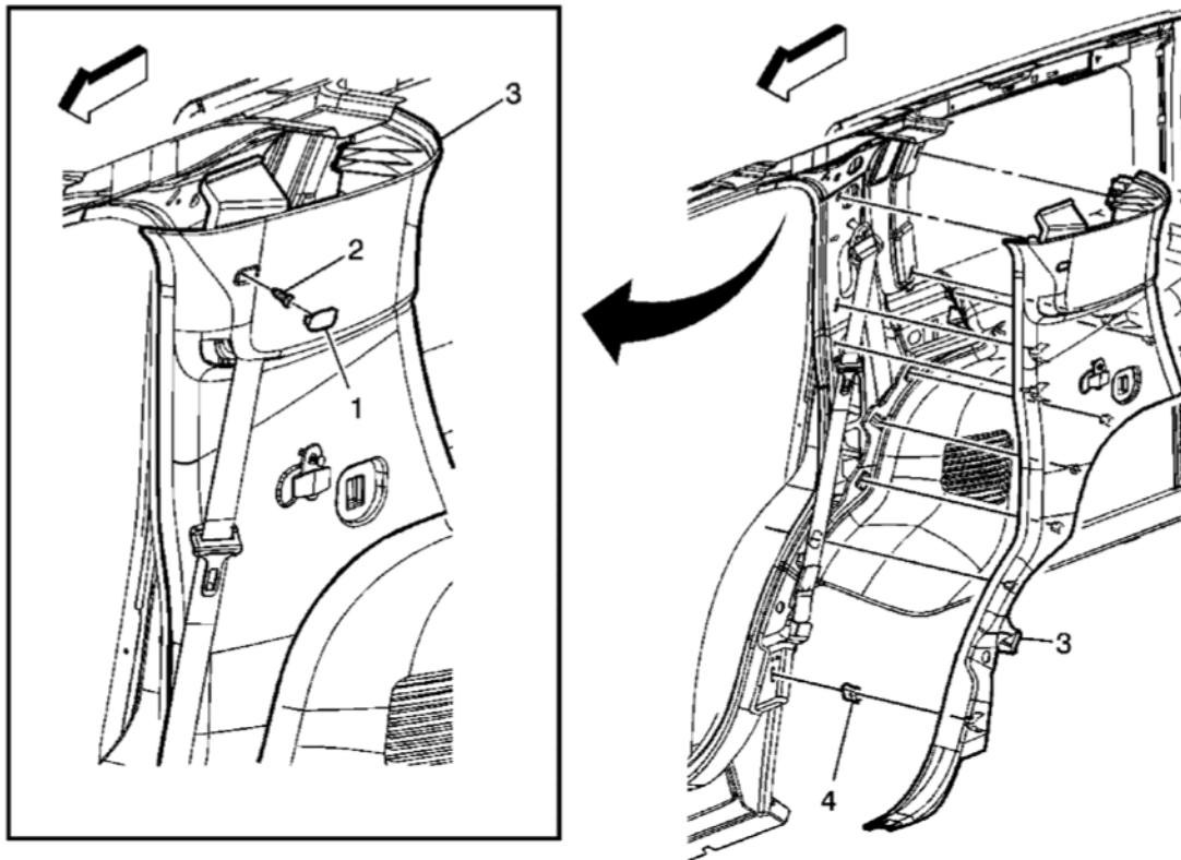
Fig. 42: View Of Body Lock Pillar Garnish Molding Assembly & Components Courtesy of GENERAL MOTORS CORP.
