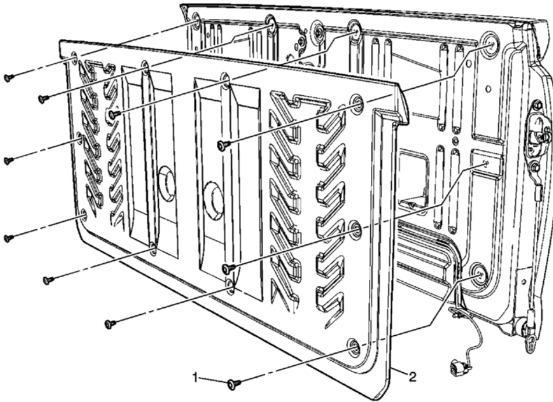
Fig. 33: View Of Endgate Trim Panel & Screws Courtesy of GENERAL MOTORS CORP.
