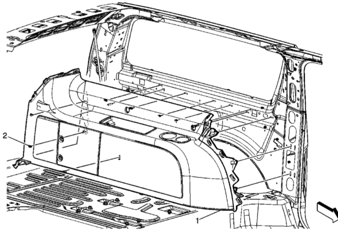
Fig. 26: View Of Body Side Trim Panel Assembly & Retainers Courtesy of GENERAL MOTORS CORP.
