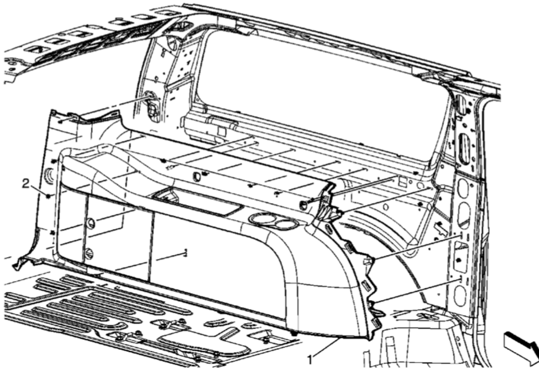
Fig. 27: View Of Body Side Trim Panel Assembly & Retainers Courtesy of GENERAL MOTORS CORP.
