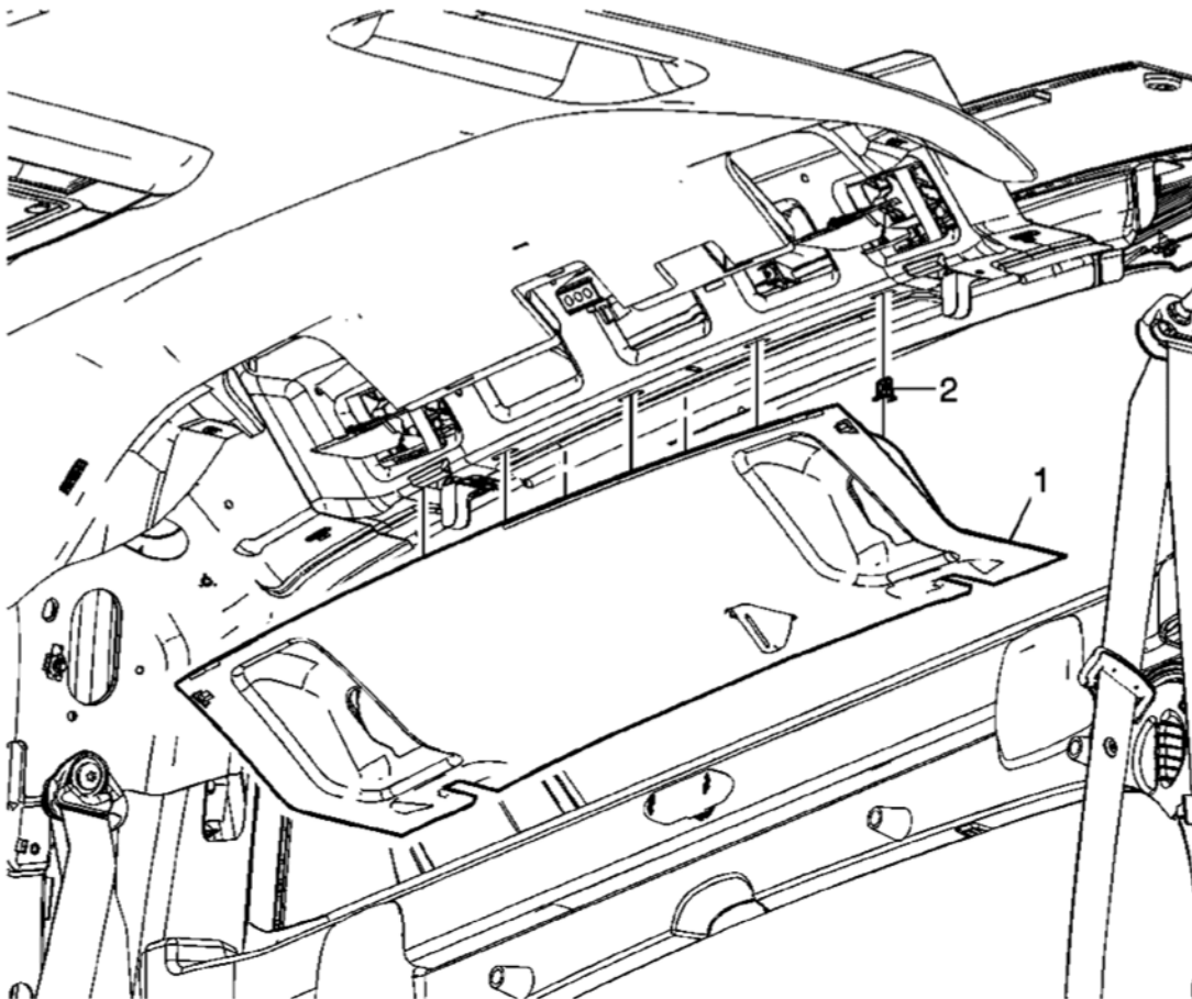
Fig. 22: View Of Headliner Trim Panel Molding Assembly & Retainers Courtesy of GENERAL MOTORS CORP.
