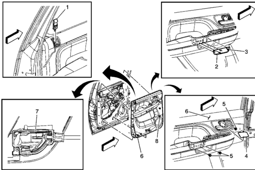
Fig. 4: View Of Rear Side Door Trim Panel Assembly & Components Courtesy of GENERAL MOTORS CORP.
