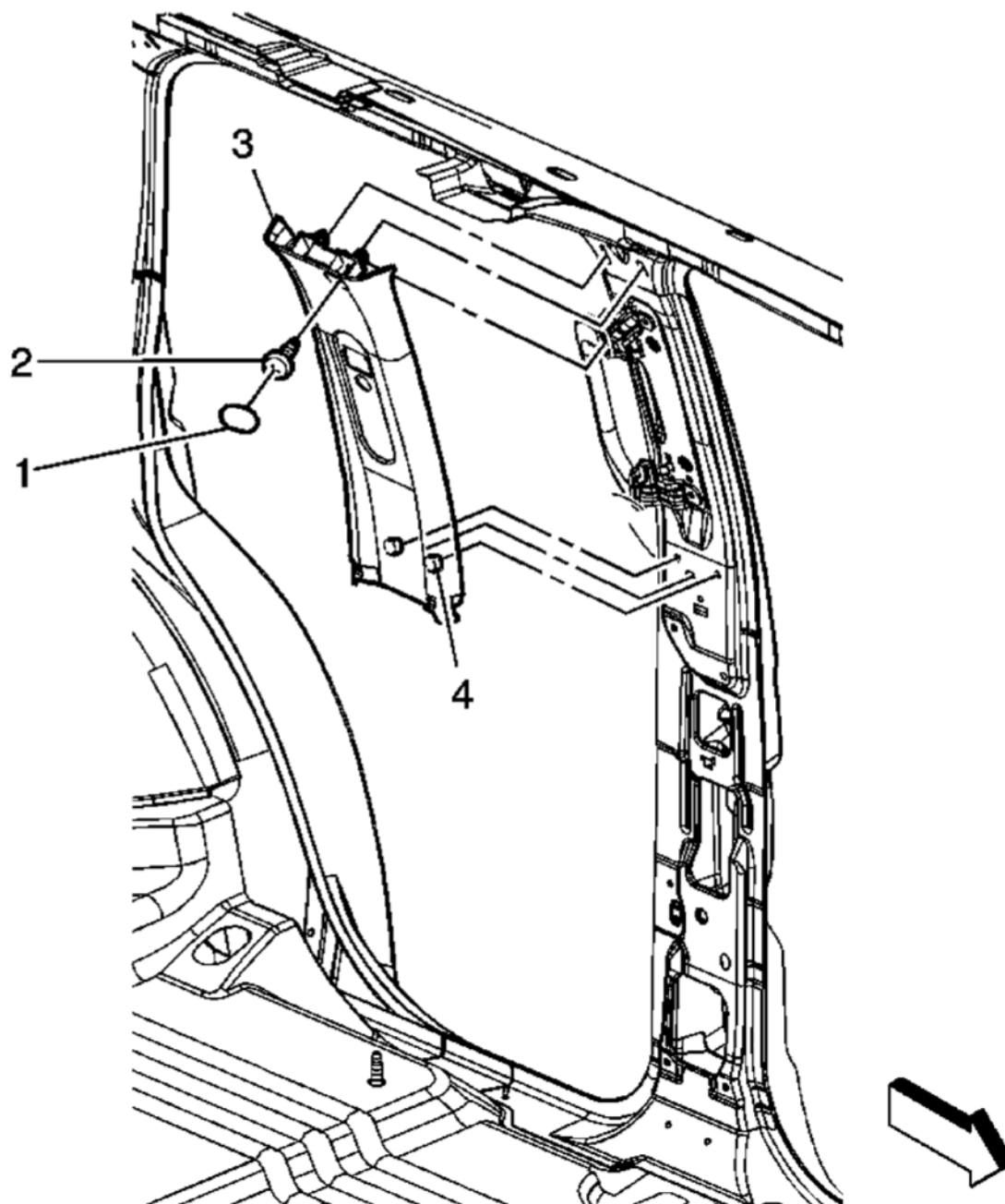
Fig. 20: View Of Center Pillar Upper Garnish Molding Assembly & Components Courtesy of GENERAL MOTORS CORP.
