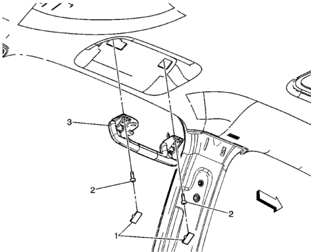
Fig. 16: View Of Roof Rail Rear Assist Handle Assembly & Components Courtesy of GENERAL MOTORS CORP.
