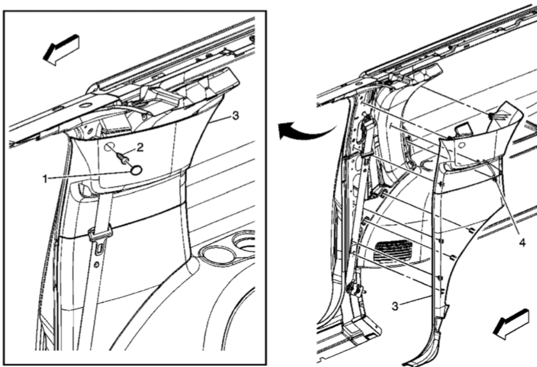
Fig. 41: View Of Body Lock Pillar Garnish Molding Assembly & Components Courtesy of GENERAL MOTORS CORP.
