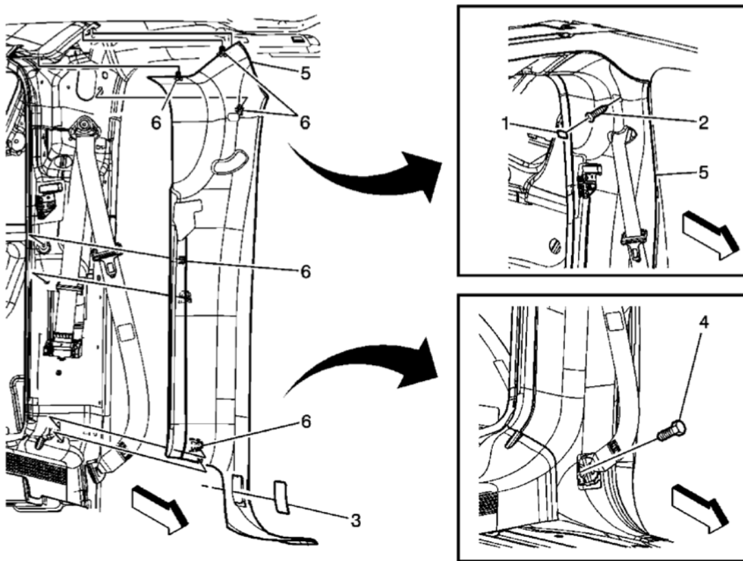
Fig. 40: View Of Body Lock Pillar Garnish Molding Assembly & Components Courtesy of GENERAL MOTORS CORP.
