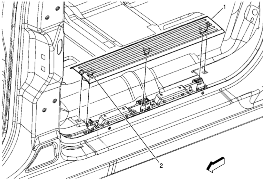
Fig. 12: View Of Rear Side Door Trim Plate Assembly & Retainers Courtesy of GENERAL MOTORS CORP.
