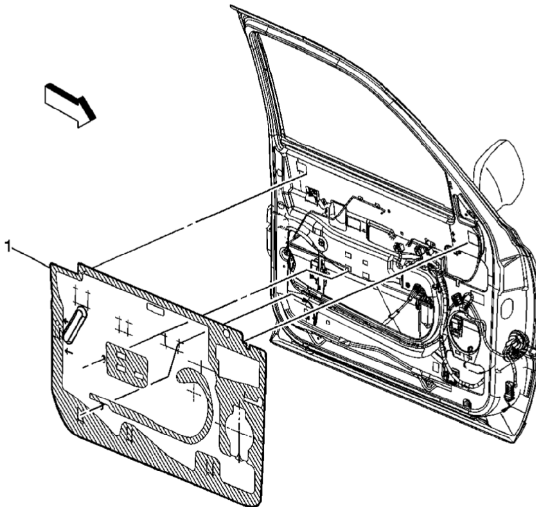
Fig. 6: View Of Front Side Door Water Deflector Courtesy of GENERAL MOTORS CORP.
