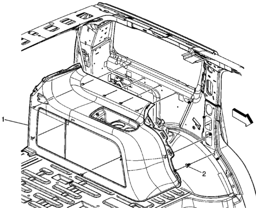
Fig. 28: View Of Body Side Trim Panel Assembly & Retainers Courtesy of GENERAL MOTORS CORP.
