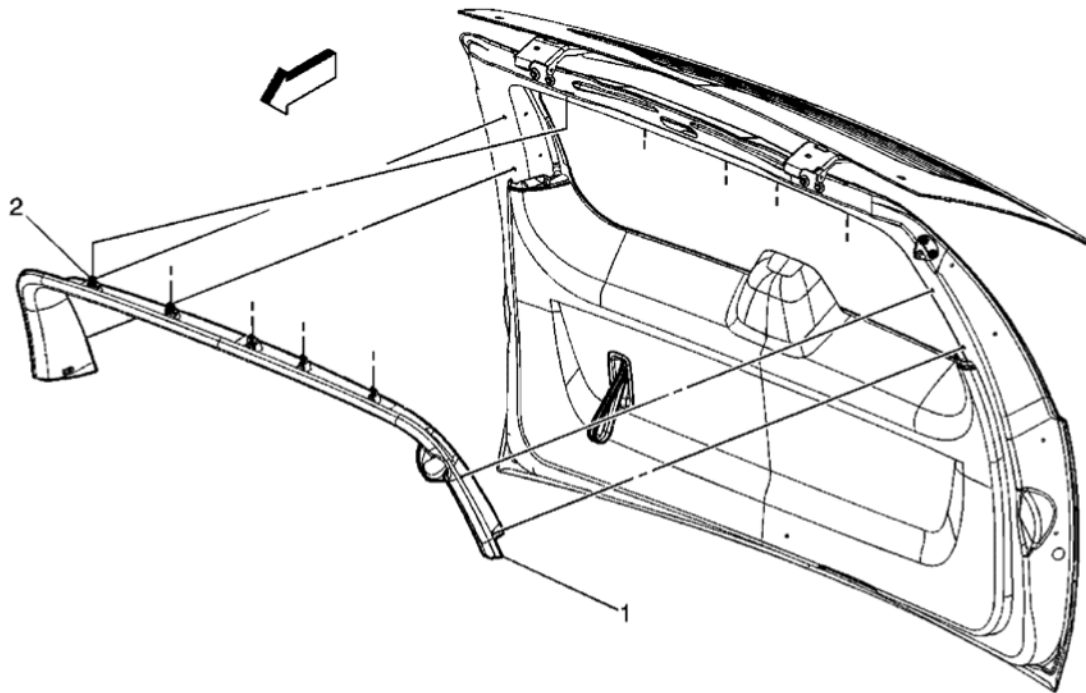
Fig. 32: View Of Liftgate Window Upper Garnish Molding Assembly & Retainers Courtesy of GENERAL MOTORS CORP.
