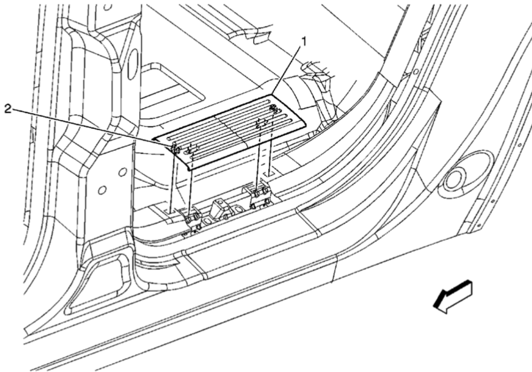
Fig. 13: View Of Rear Side Door Sill Plate Assembly & Retainers Courtesy of GENERAL MOTORS CORP.
