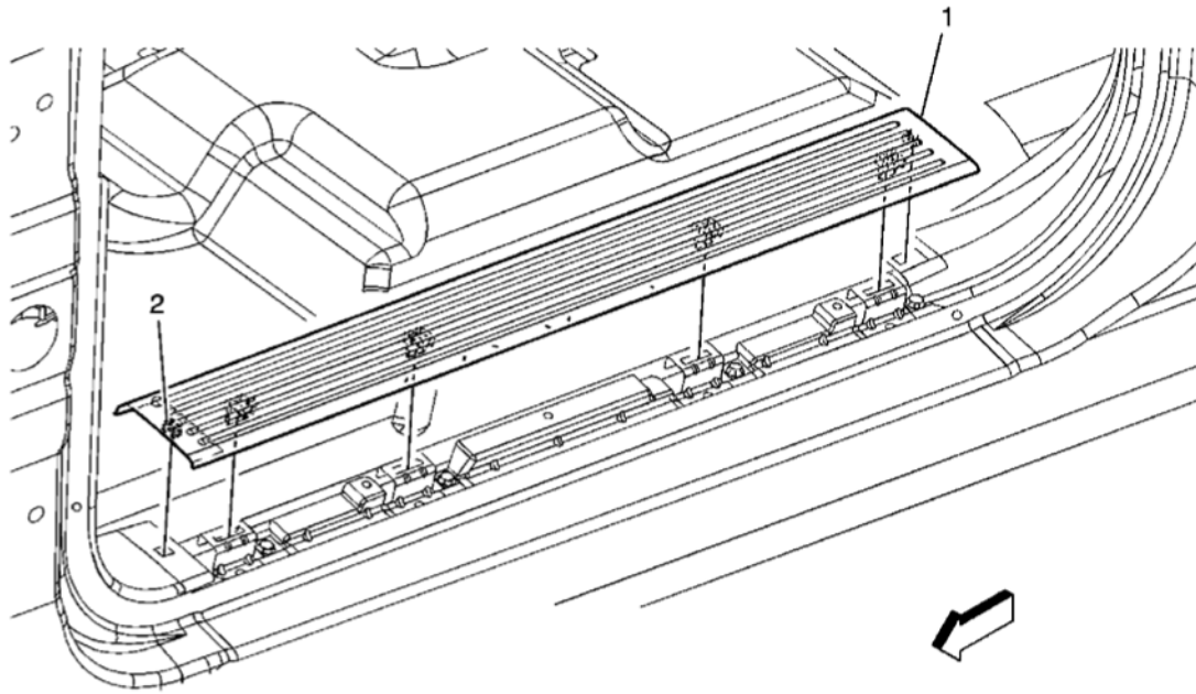
Fig. 11: View Of Front Side Door Sill Plate Assembly & Retainers Courtesy of GENERAL MOTORS CORP.
