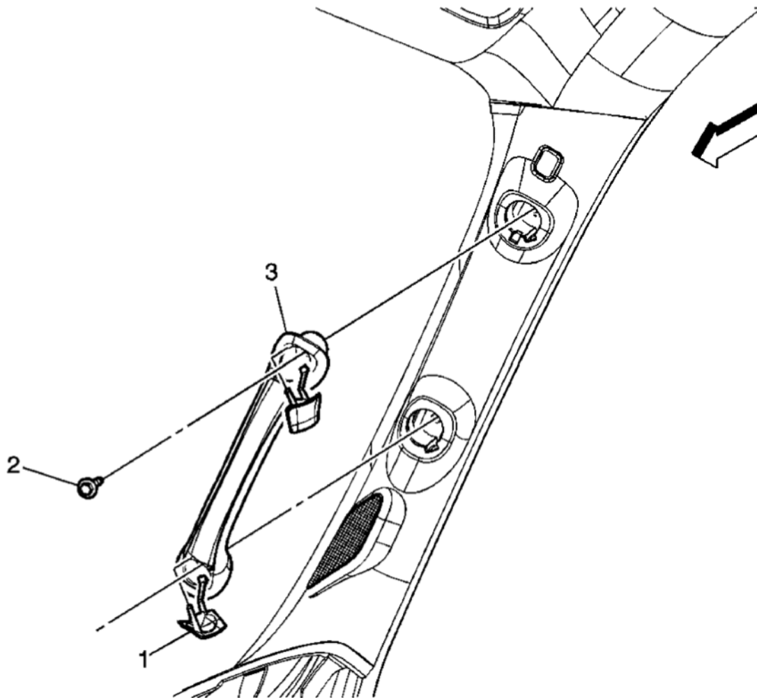
Fig. 15: View Of Windshield Pillar Assist Handle Cover Assembly & Components Courtesy of GENERAL MOTORS CORP.
