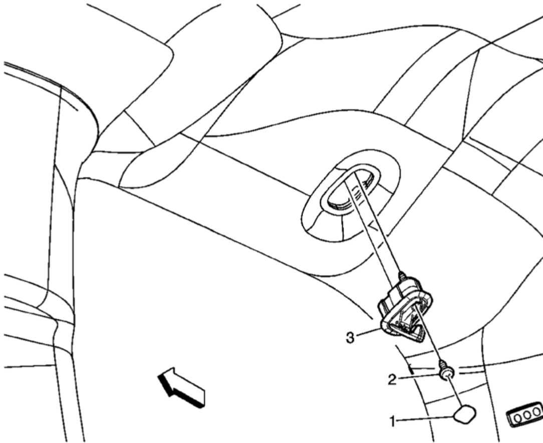
Fig. 17: View Of Coathook Assembly, Cover & Screw Courtesy of GENERAL MOTORS CORP.
